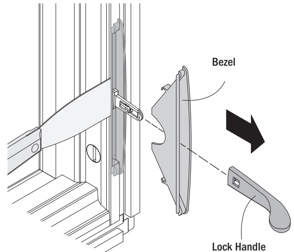
VeriLock Dummy Assembly
