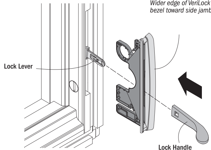
VeriLock Dummy Assembly
