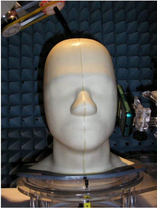
Figure 21 LH-Cheek Position
