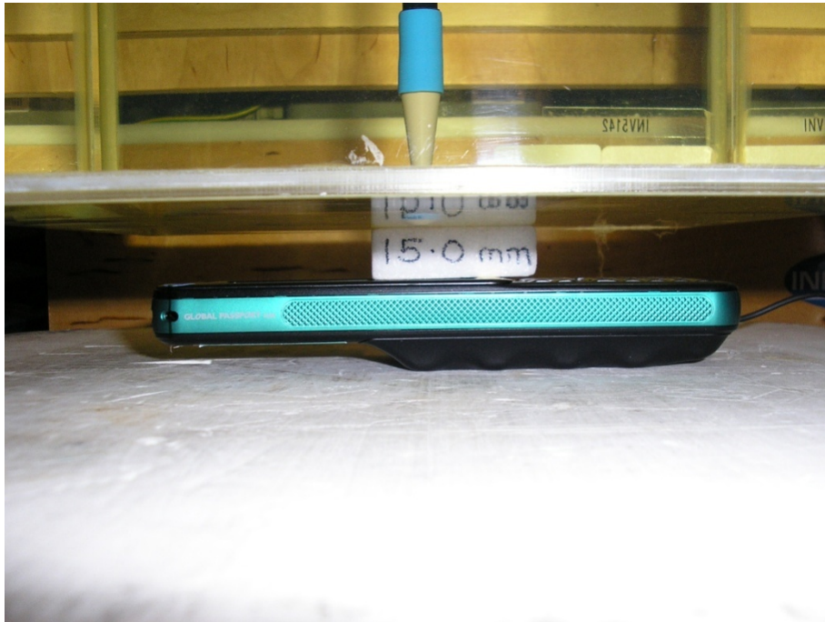
Figure 25 Body-Front Position
