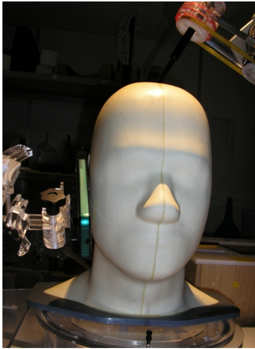
Figure 23 RH-Cheek Position
