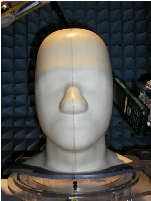
Figure 22 LH-15° Position
