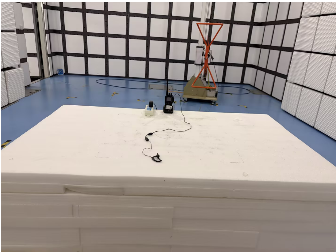
Radiation Emission - Back View (Below 1GHz) – For Charger
