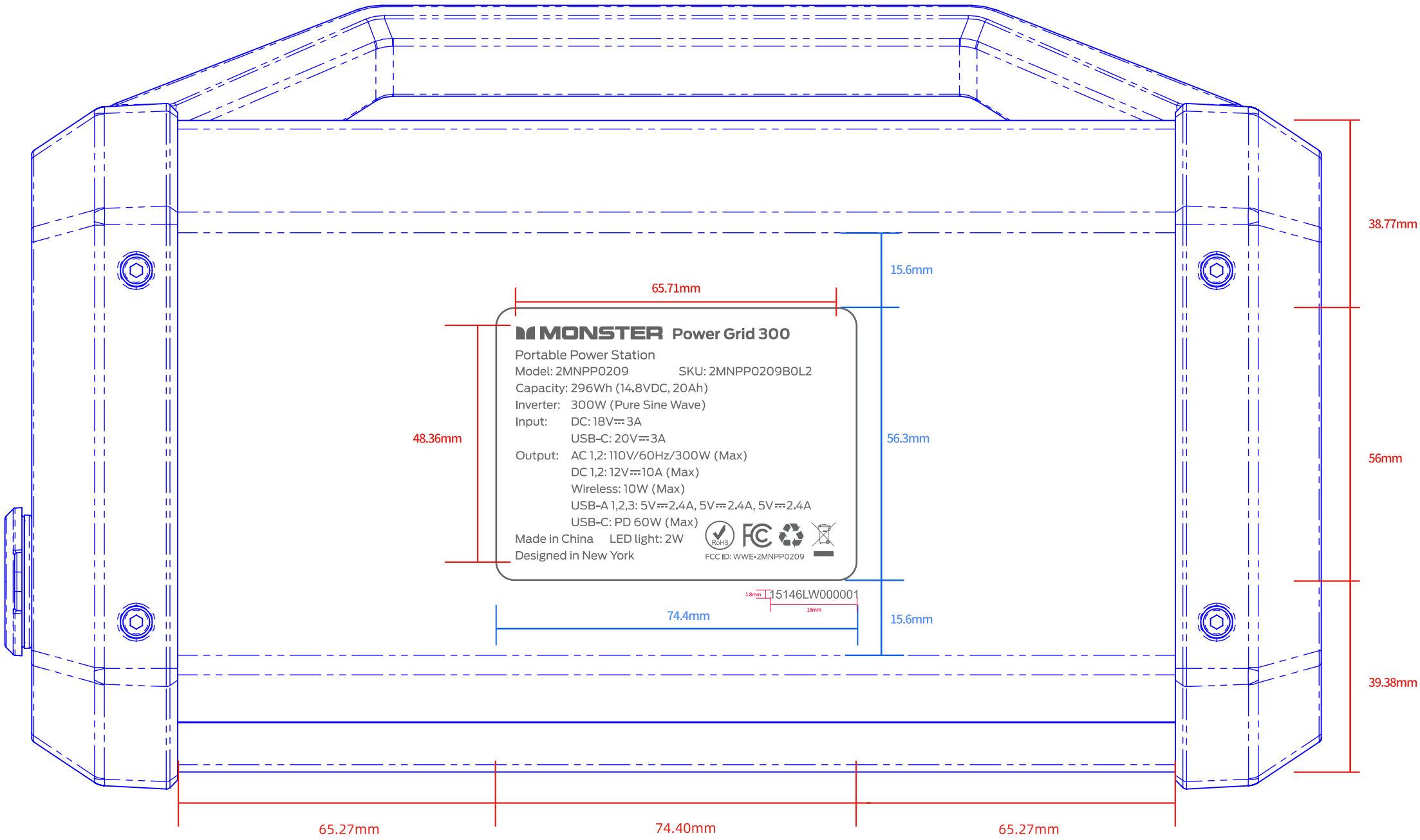
Bottom View
