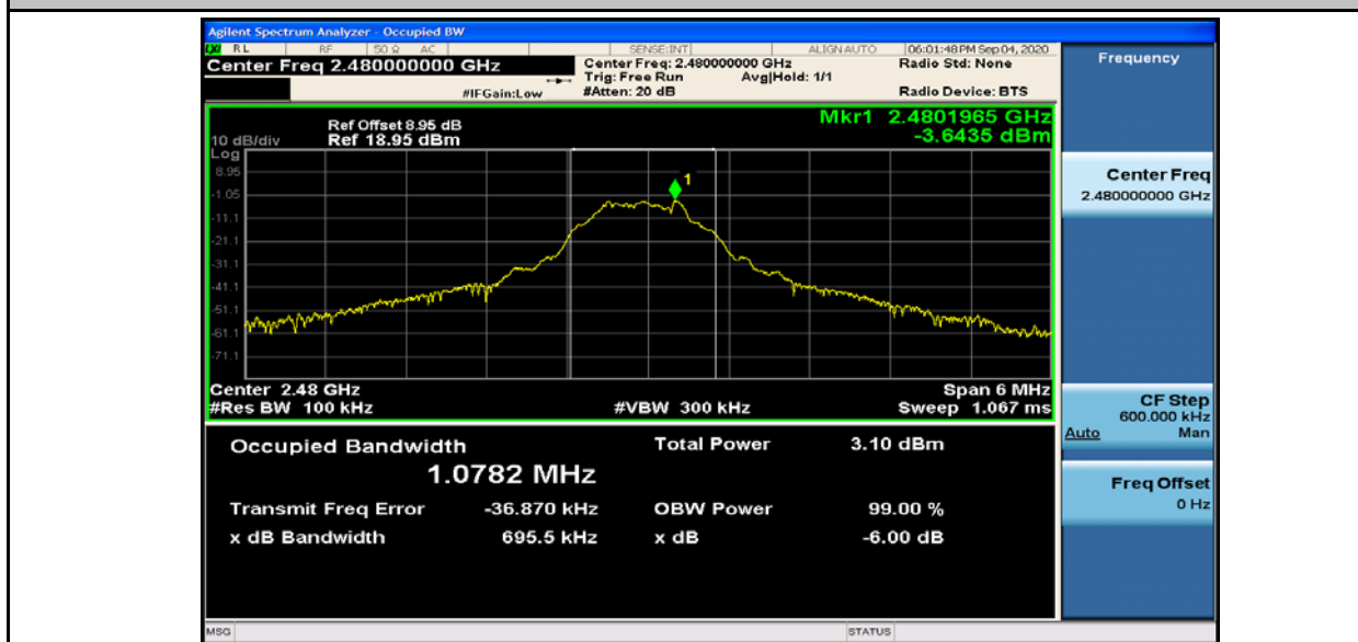
6dB Bandwidth_BLE_2480
