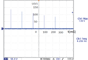
Output waveforms Pulse burst (500 \Omega )
