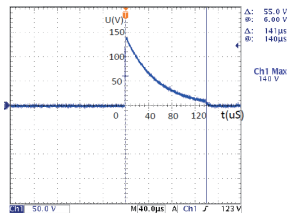
Output waveforms at loads of 10k \Omega
