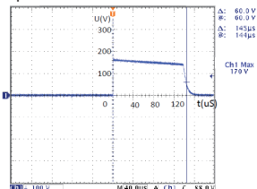
Output waveforms at loads of 10k \Omega
