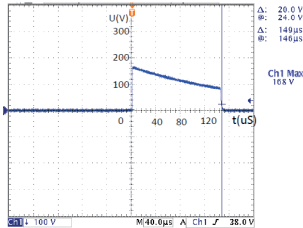
Output waveforms Pulse burst (500 \Omega )
