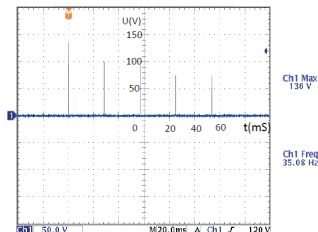
Output waveforms Pulse burst (500 \Omega )
