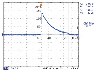
Output waveforms at loads of 10k \Omega
