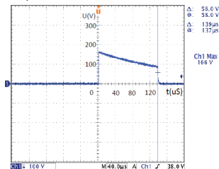
Output waveforms Pulse burst (500 \Omega )
