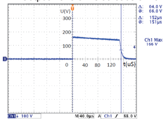
Output waveforms at loads of 10k \Omega
