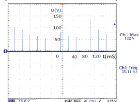
Output waveforms Pulse burst (500 \Omega )
