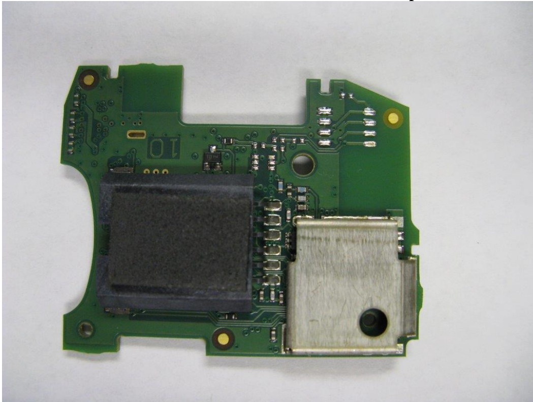
Bottom View of COMMS Board - Close Up
