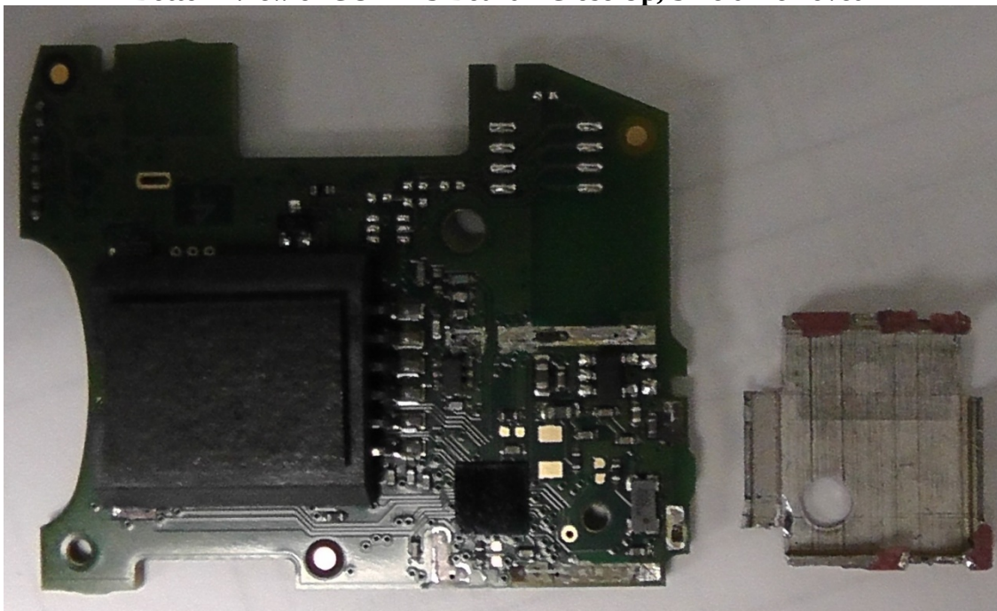
Bottom View of COMMS Board - Close Up, Shield Removed
