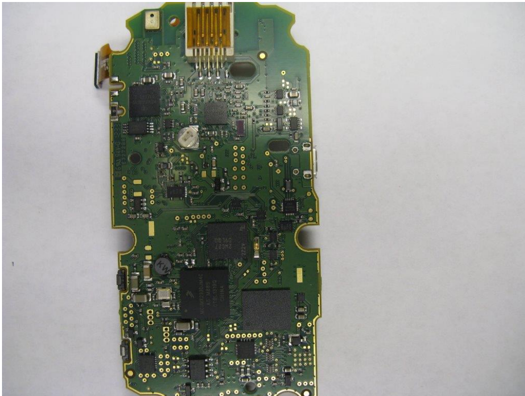
Bottom View of Mother Board
