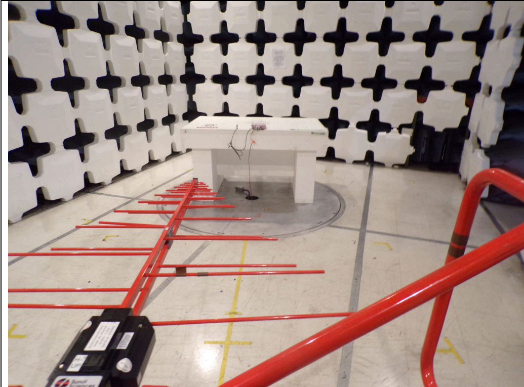
30MHz-1GHz
