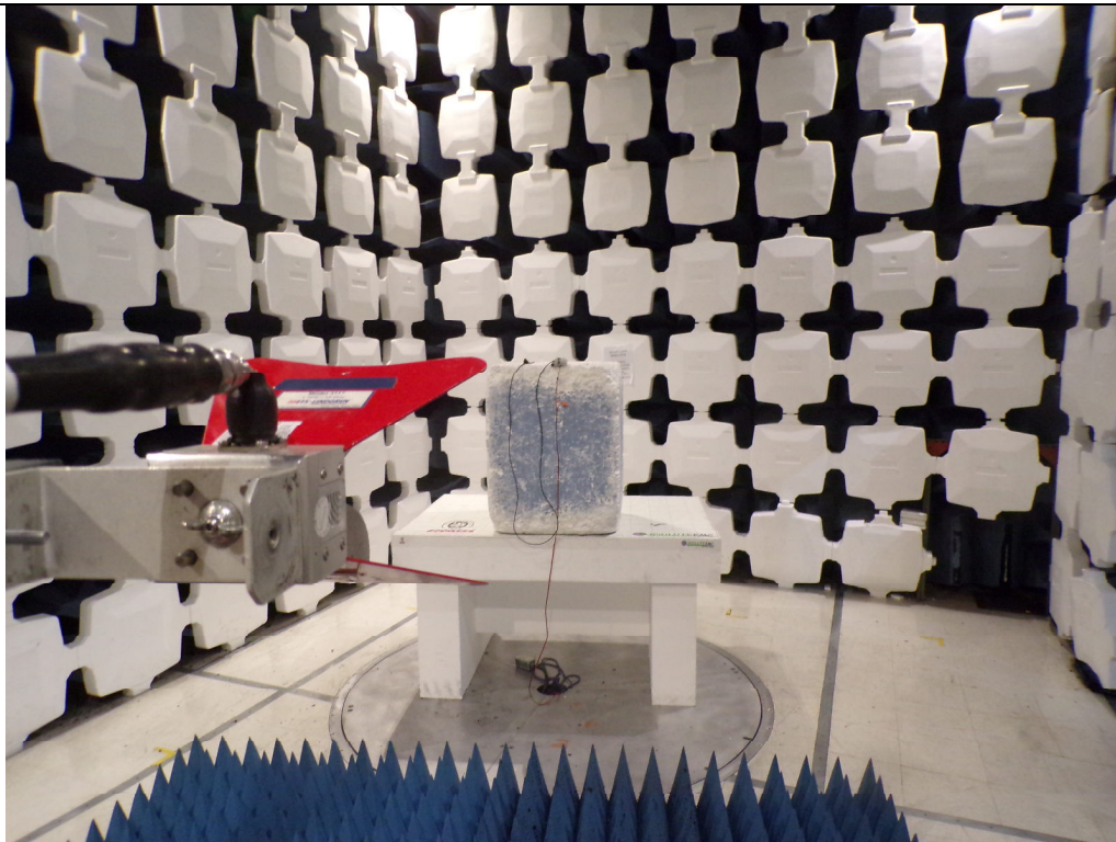
1GHz-6GHz
