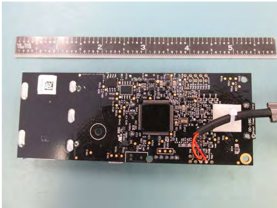
RXW-LIA-900 PCB Back
