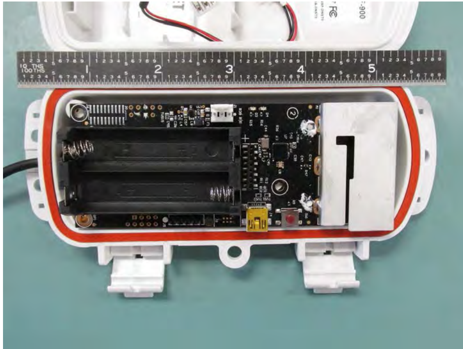
RXW-RGF-900 PCB Front
