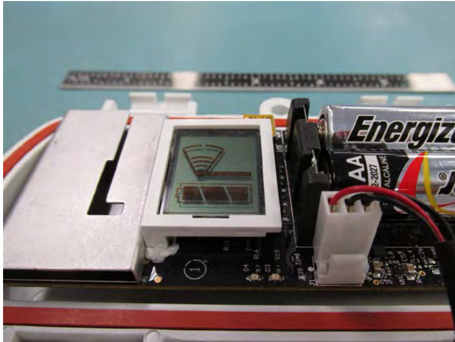
RXW-LIB-900 Radio & LCD
