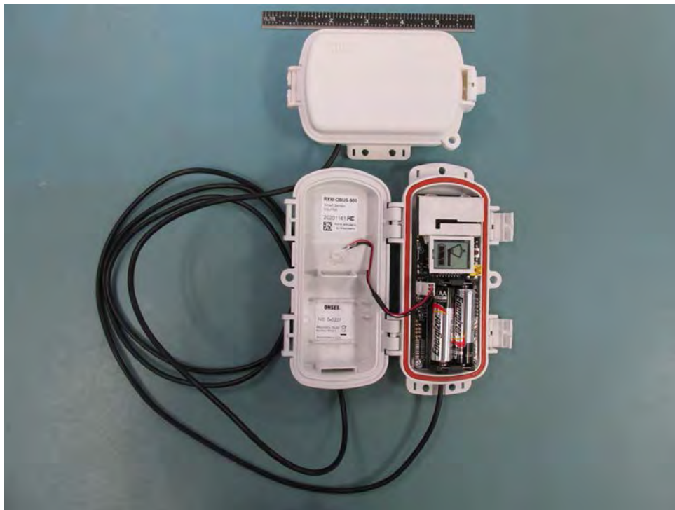
RXW-OBUS-900 Product Case Open
