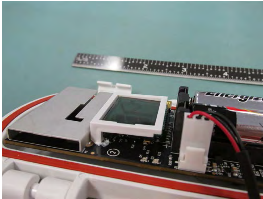
RXW-RGF-900 Radio & LCD
