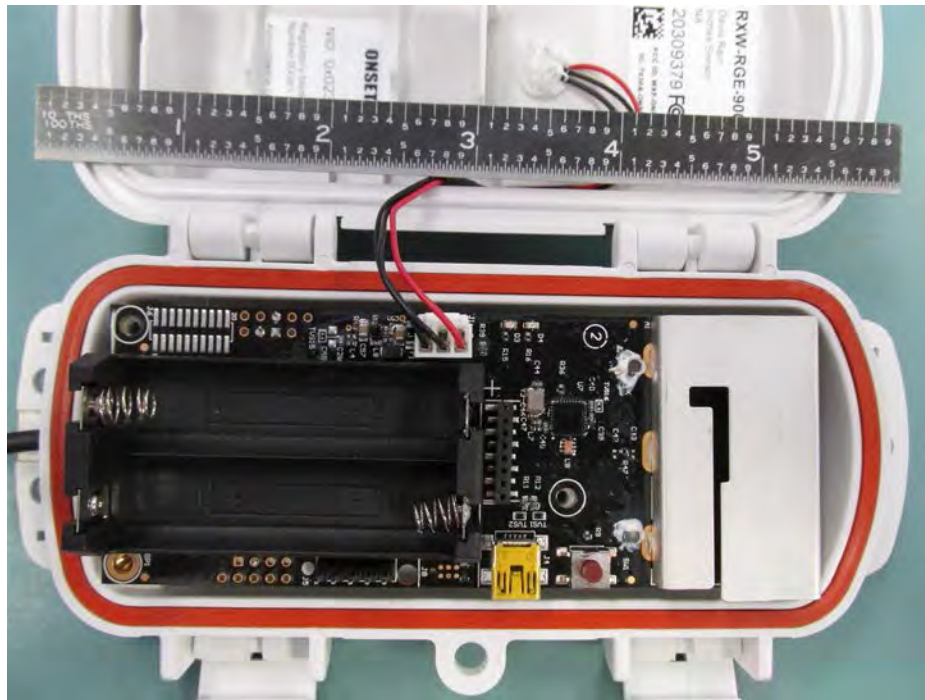
RXW-RGE-900 PCB Front
