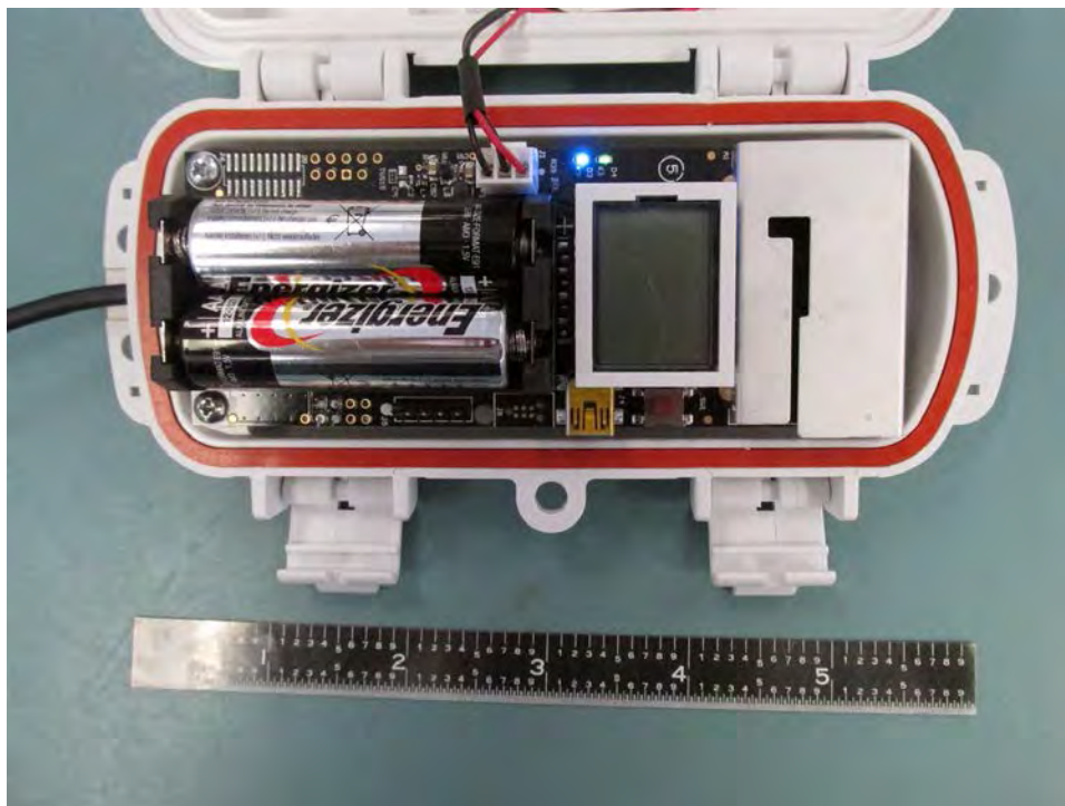
RXW-OBUS-900 PCB in Housing
