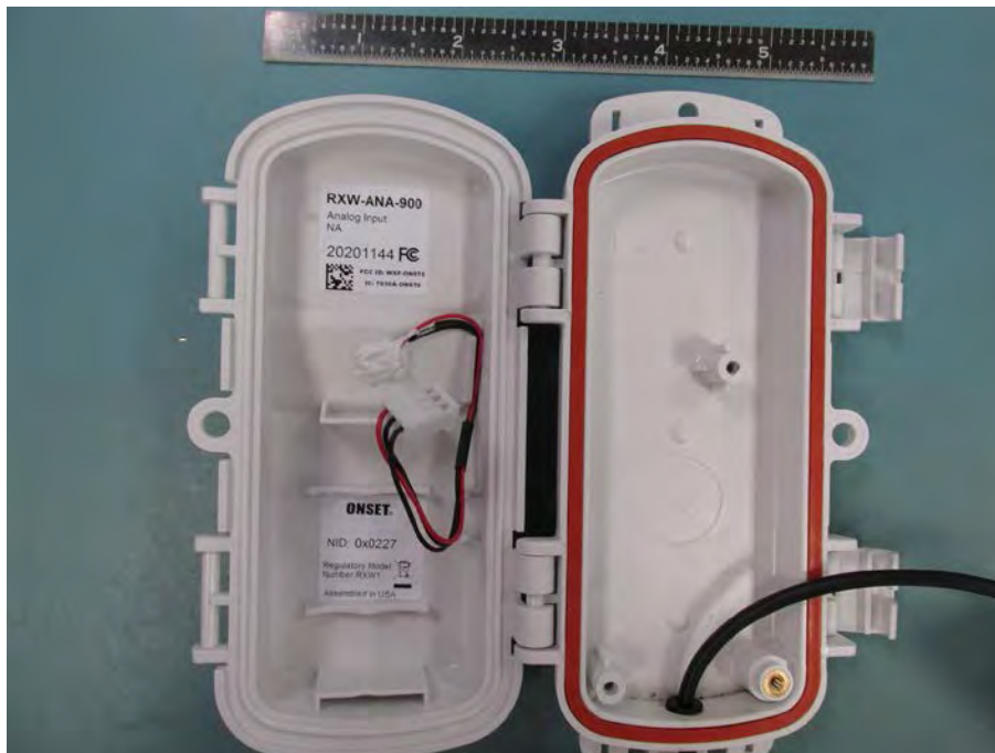
RXW-ANA-900 Inner Housing
