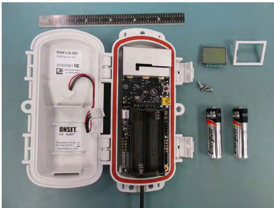
RXW-LIA-900 LCD Removed
