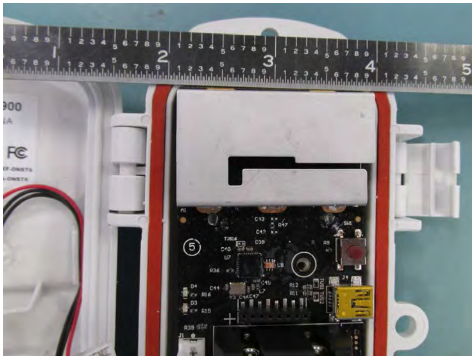
RXW-ANA-900 Radio Circuit
