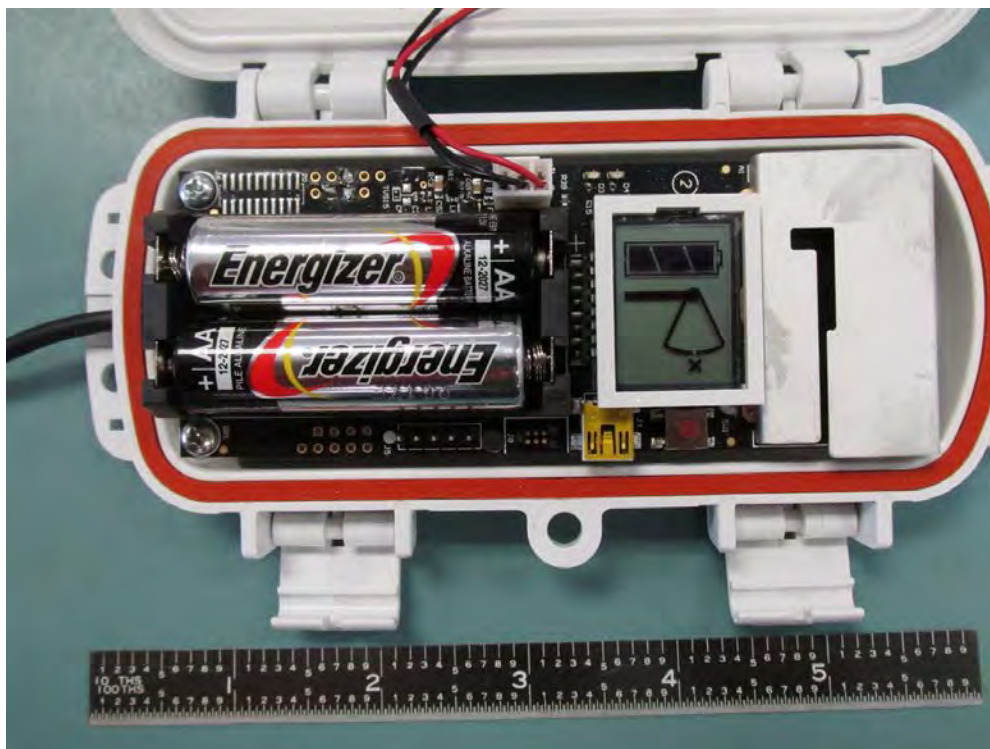
RXW-RGF-900 PCB in Housing
