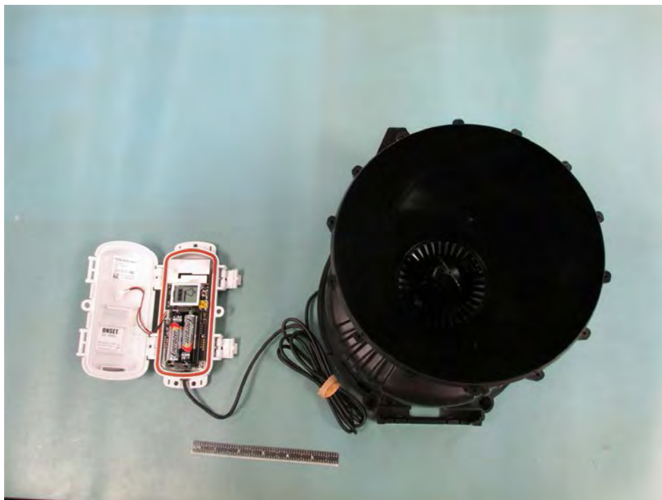
RXW-RGF-900 Product Case Open
