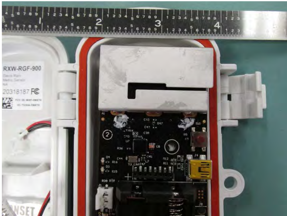
RXW-RGF-900 Radio Circuit
