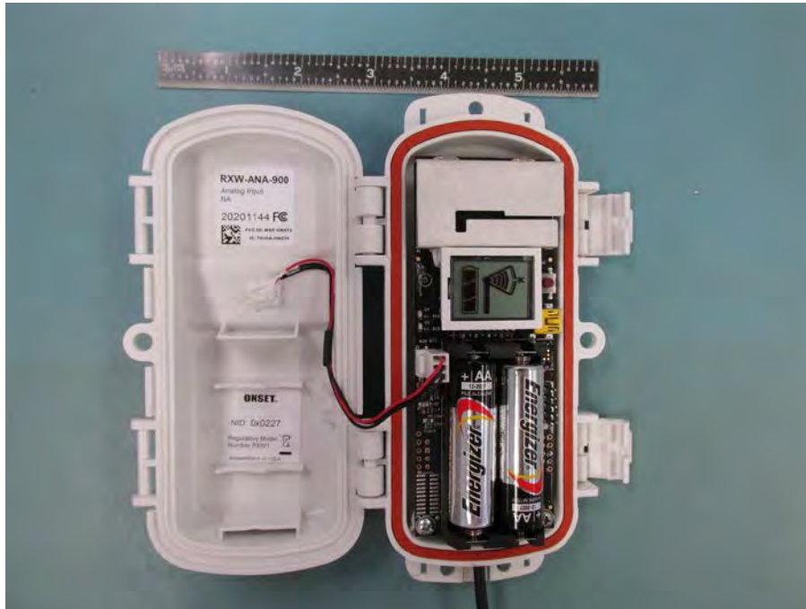
RXW-ANA-900 Housing Open
