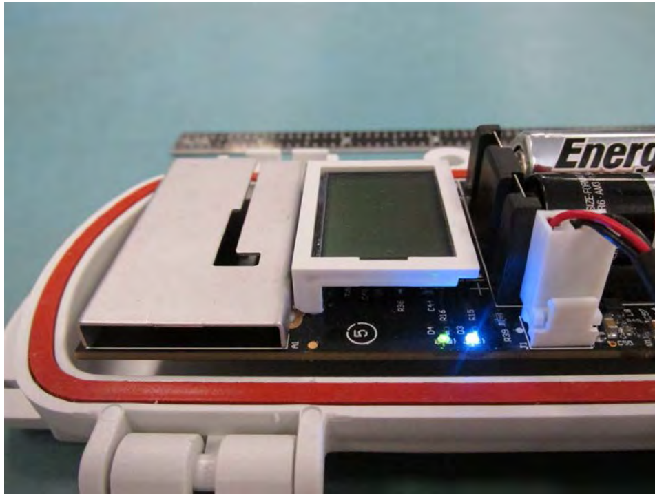
RXW-OBUS-900 Radio & LCD
