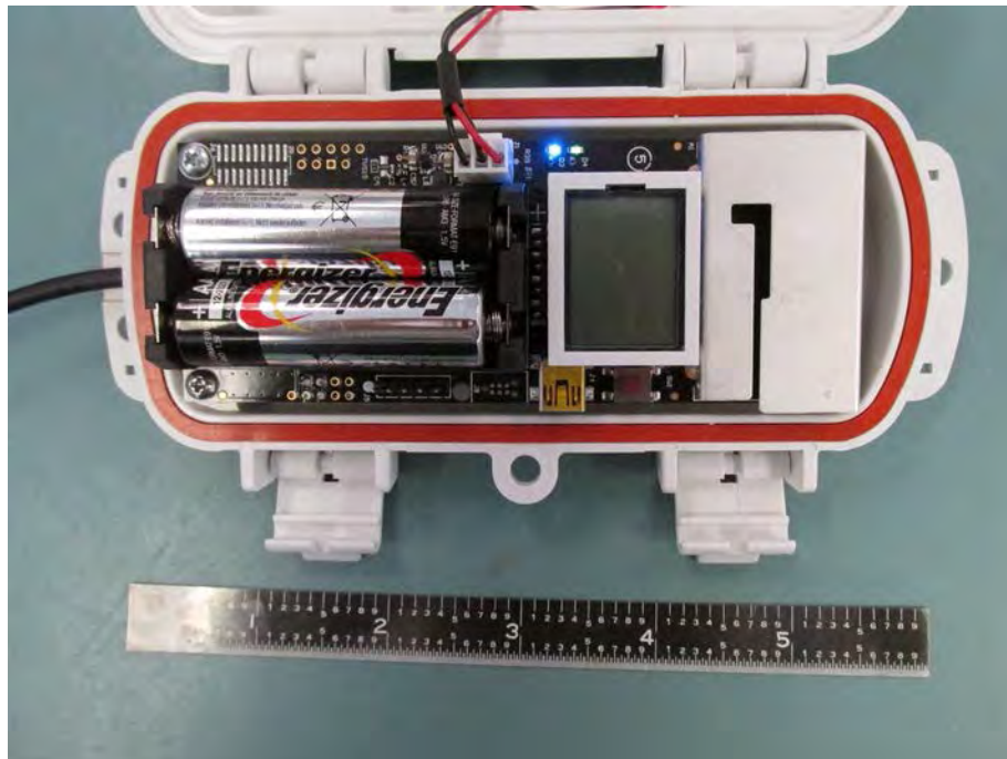
RXW-ANA-900 PCB in Housing
