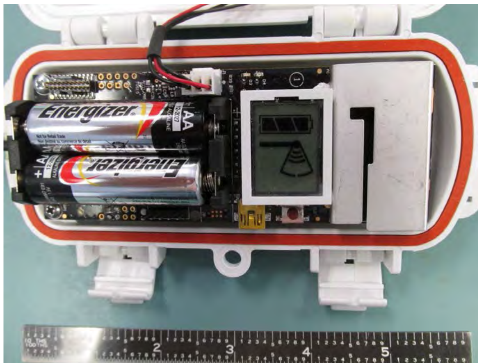
RXW-LIB-900 PCB in Housing
