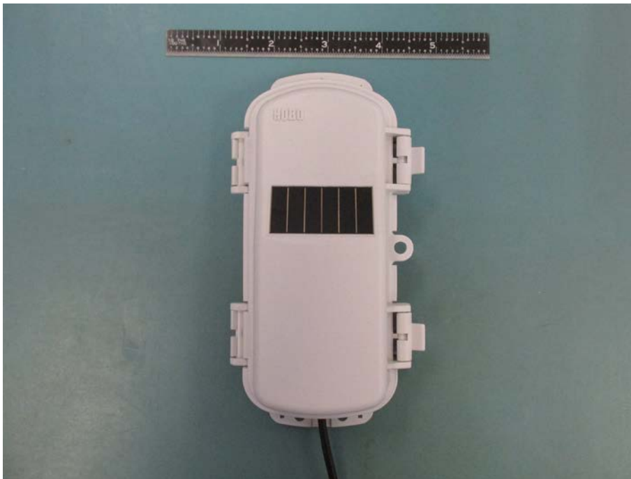
RXW-ANA-900 Housing Front
