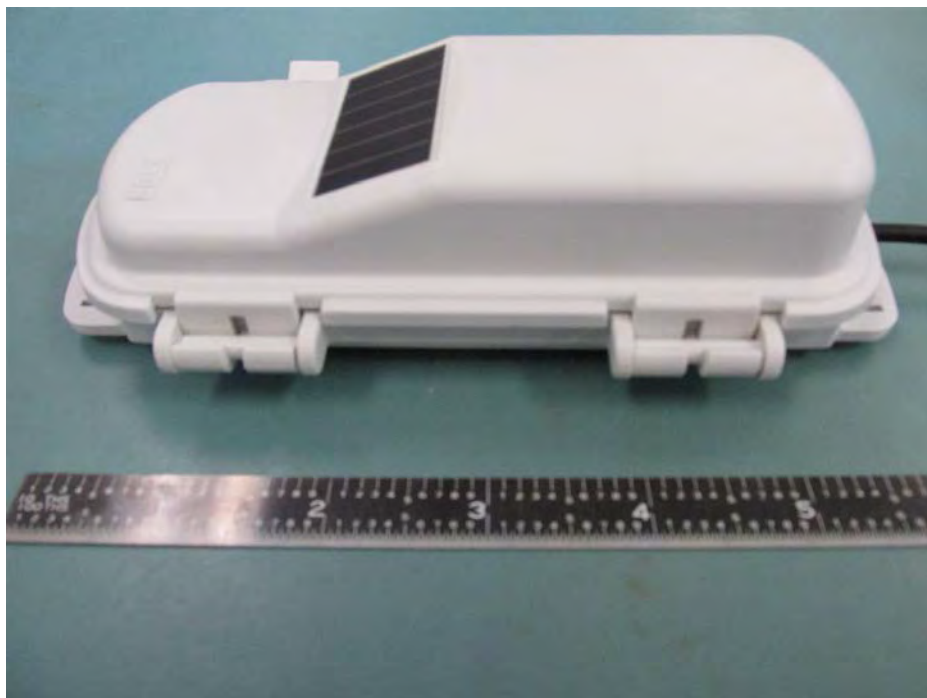
RXW-ANA-900 Housing Left Side
