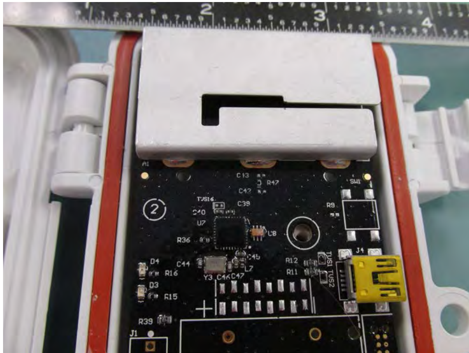
RXMOD-RXW-900 Radio Circuit
