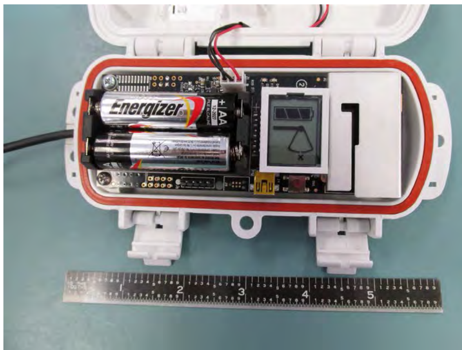
RXW-RGE-900 PCB in Housing
