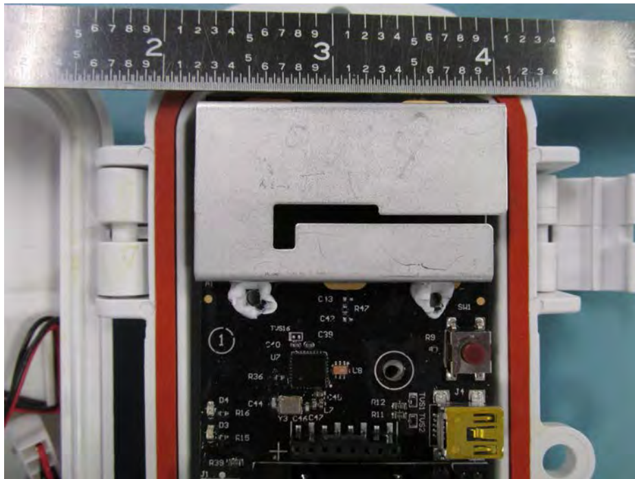
RXW-LIB-900 Radio Circuit
