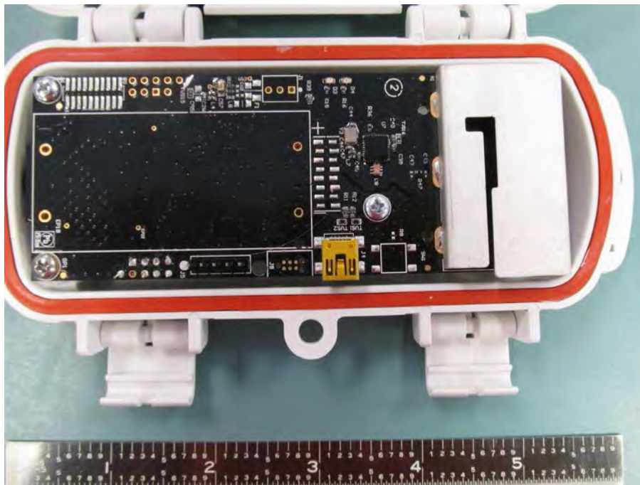
RXMOD-RXW-900 PCB in Housing
