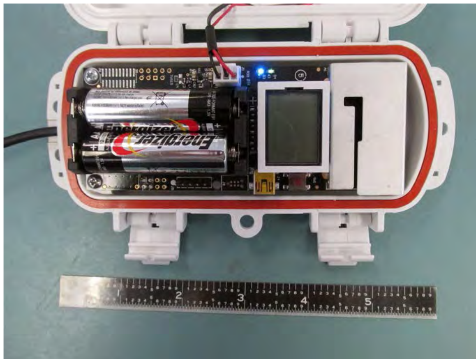
RXW-LIA-900 PCB in Housing
