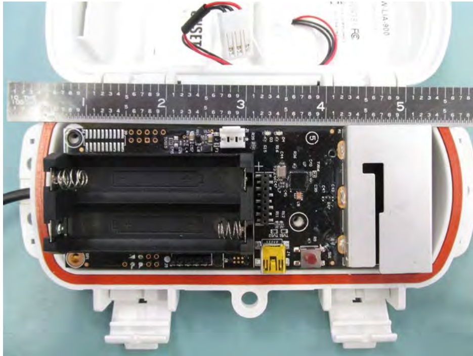
RXW-ANA-900 PCB Front
