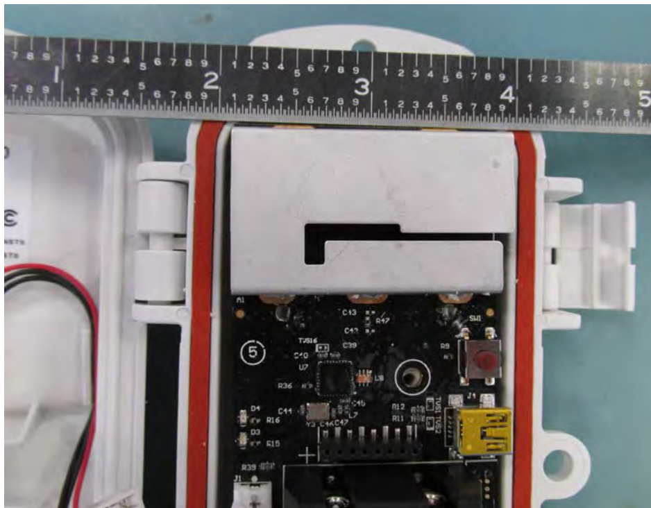
RXW-OBUS-900 Radio Circuit
