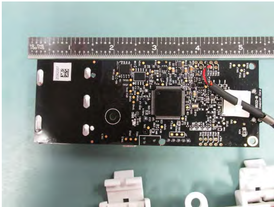
RXW-RGF-900 PCB Back
