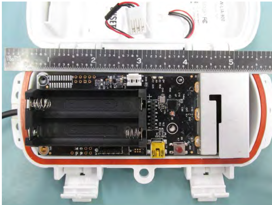
RXW-LIA-900 PCB Front
