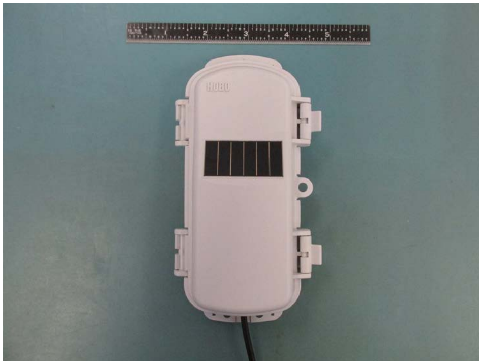
RXW-OBUS-900 Housing Front
