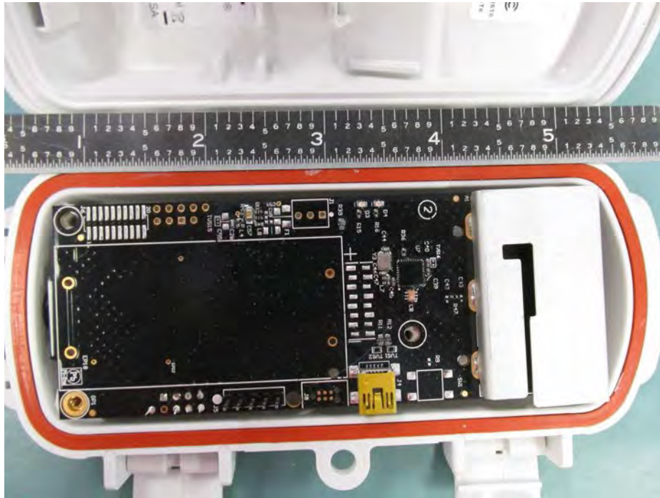
RXMOD-RXW-900 PCB Front
