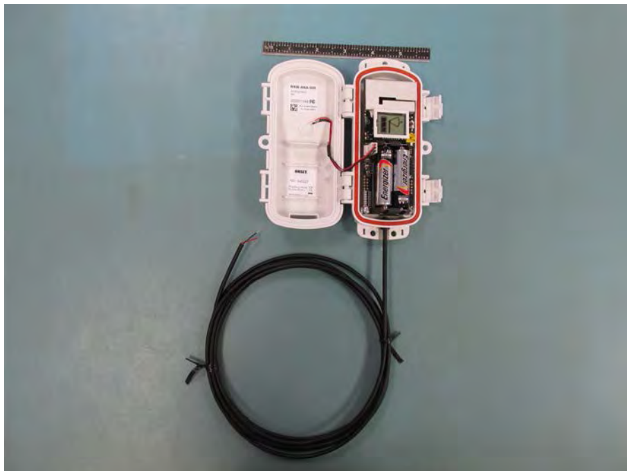
RXW-ANA-900 Product Case Open
