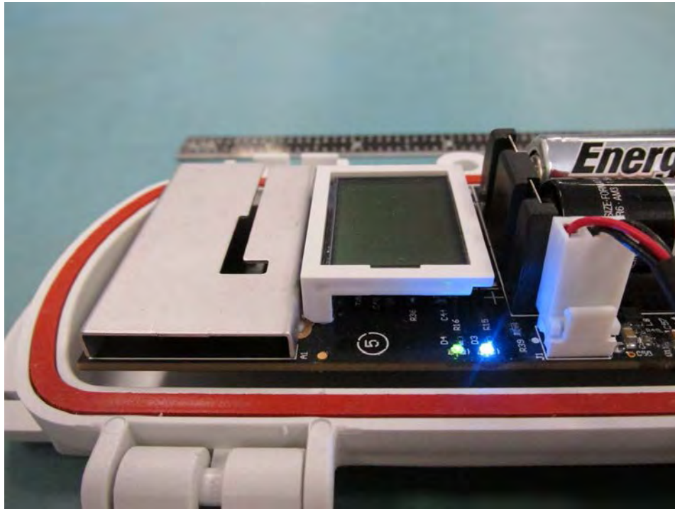
RXW-LIA-900 Radio & LCD
