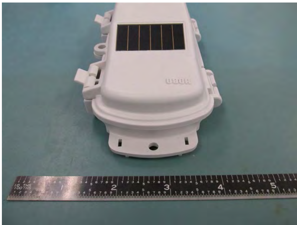
RXW-ANA-900 Housing Top
