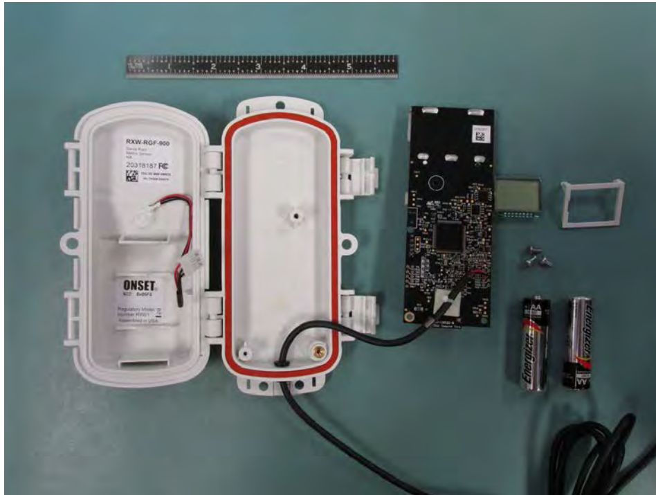
RXW-RGF-900 Exploded View
