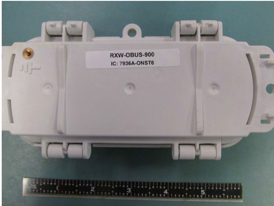
RXW-OBUS-900 Housing Back
