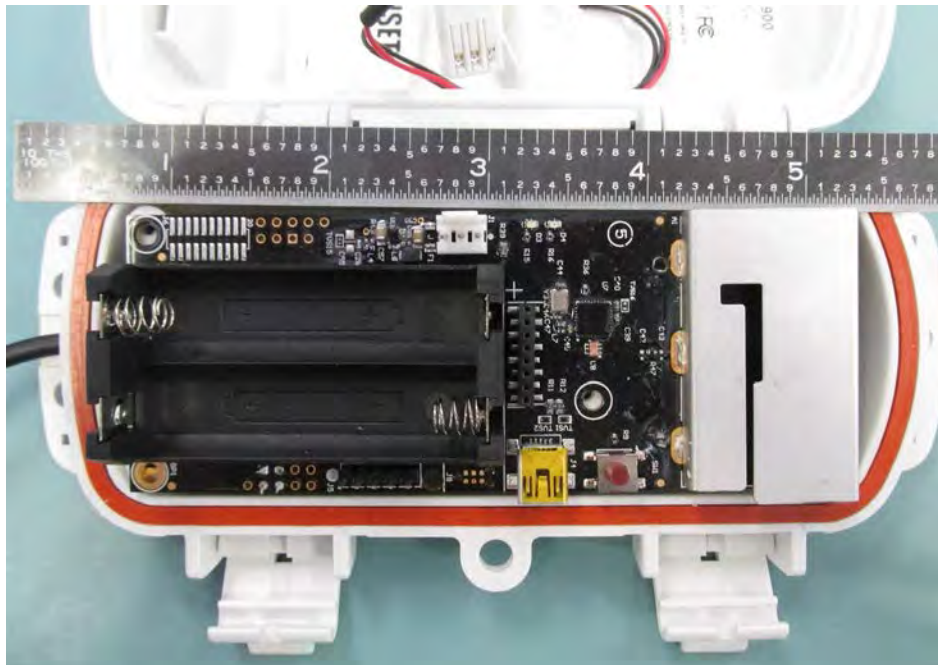
RXW-OBUS-900 PCB Front
