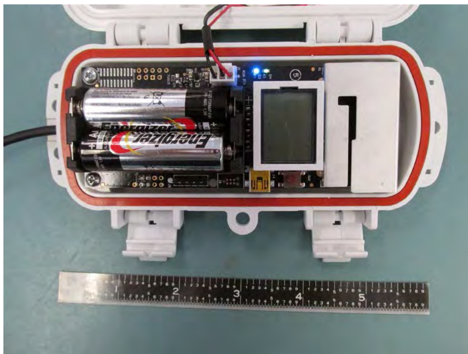
RXW-SPER-900 PCB in Housing
