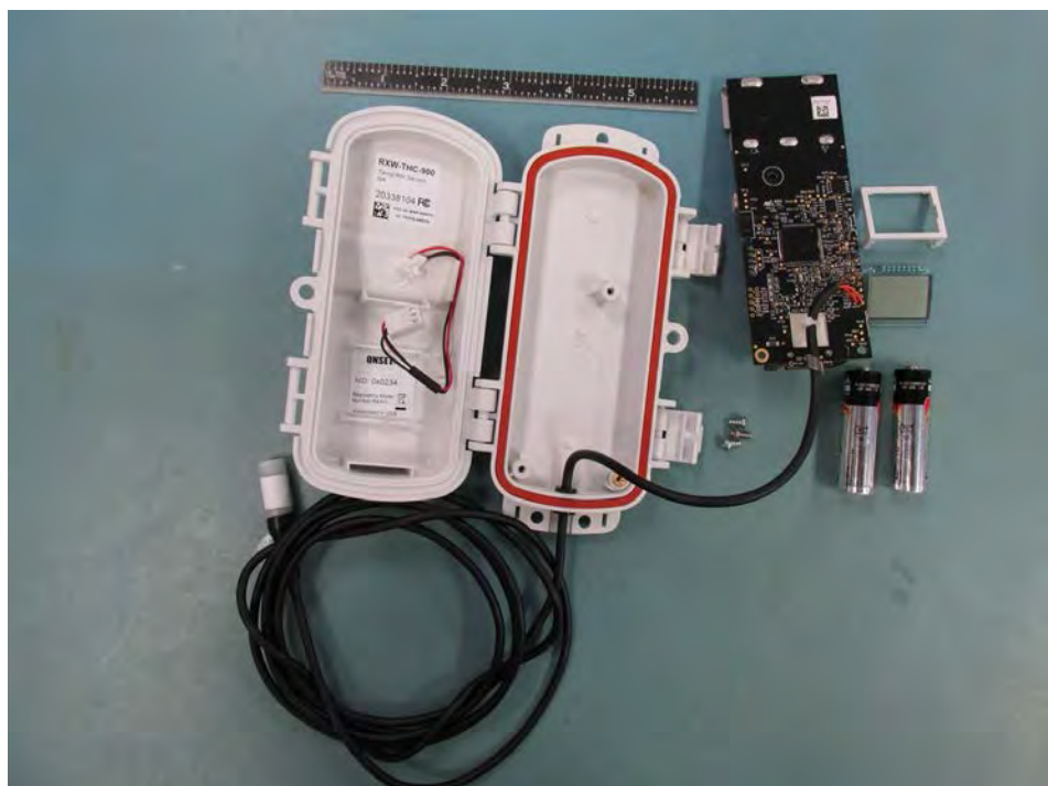
RXW-THC-900 Exploded View with Sensor
