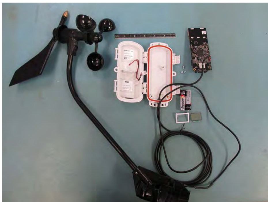
RXW-WCF-900 Exploded View with Sensor
