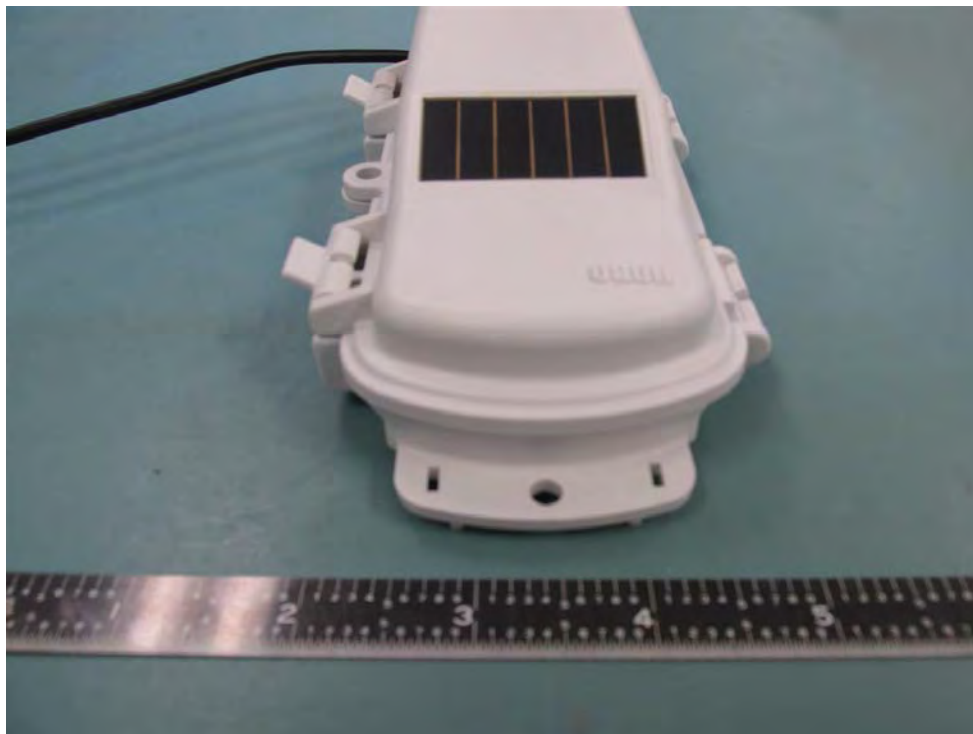
RXW-WCF-900 Housing Top
