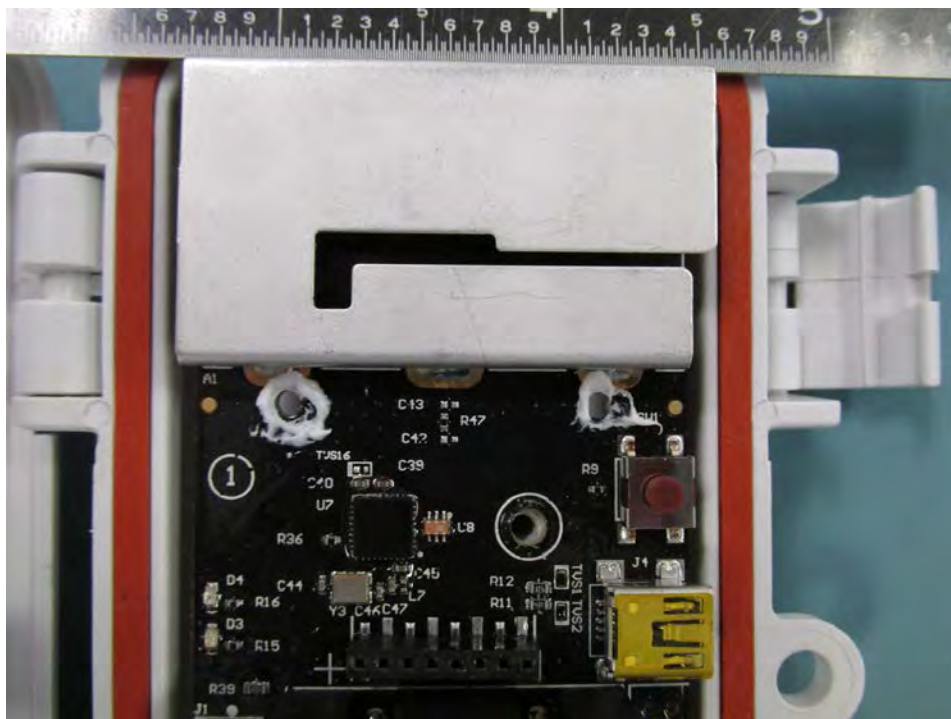
RXW-SMD-900 Radio Circuit
