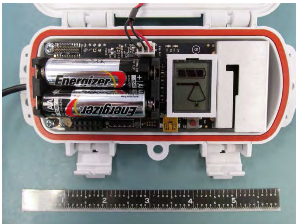
RXW-WCF-900 PCB in Housing
