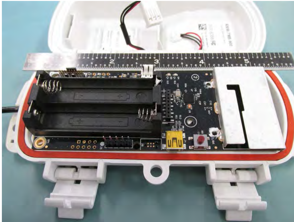
RXW-TMB-900 PCB Front
