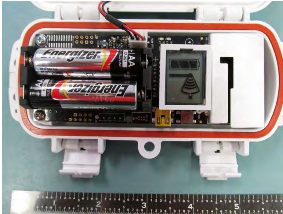
RXW-RPTR-900 PCB in Housing
