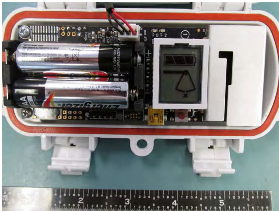
RXW-SMD-900 PCB in Housing
