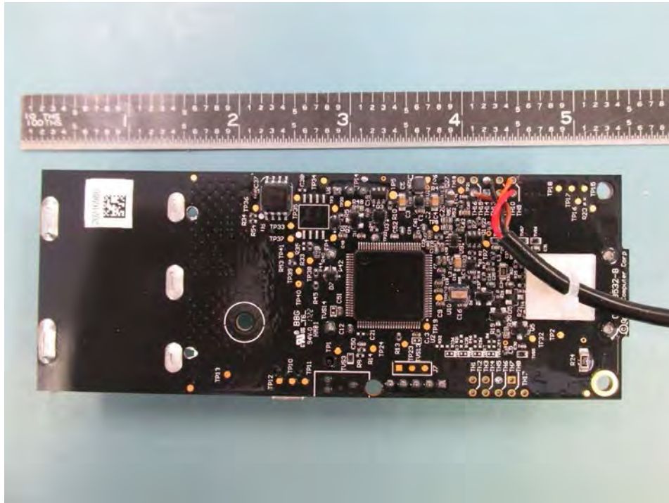
RXW-TMB-900 PCB Back
