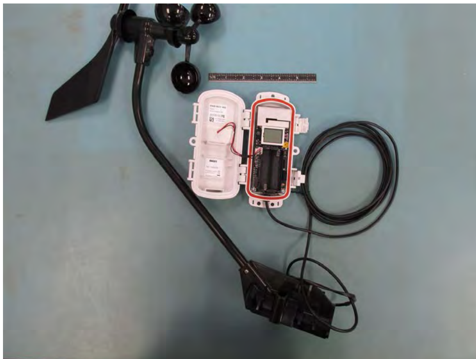
RXW-WCF-900 Product Case Open
