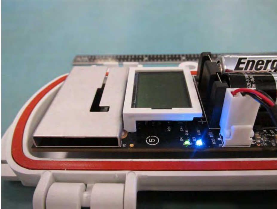
RXW-SPER-900 Radio & LCD
