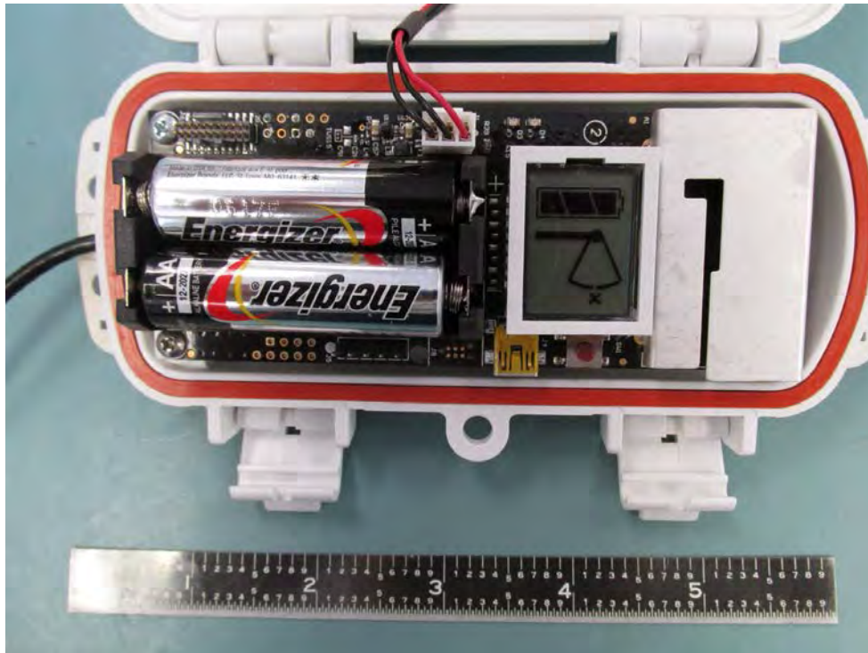
RXW-TMB-900 PCB in Housing
