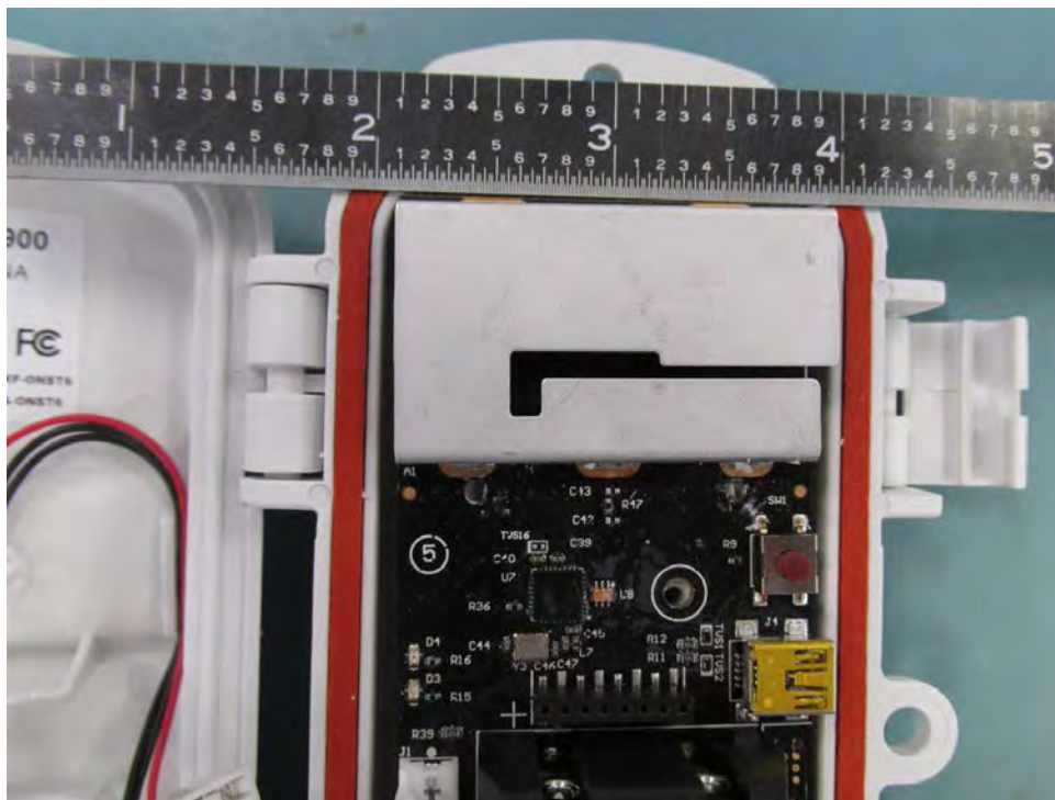
RXW-SPER-900 Radio Circuit
