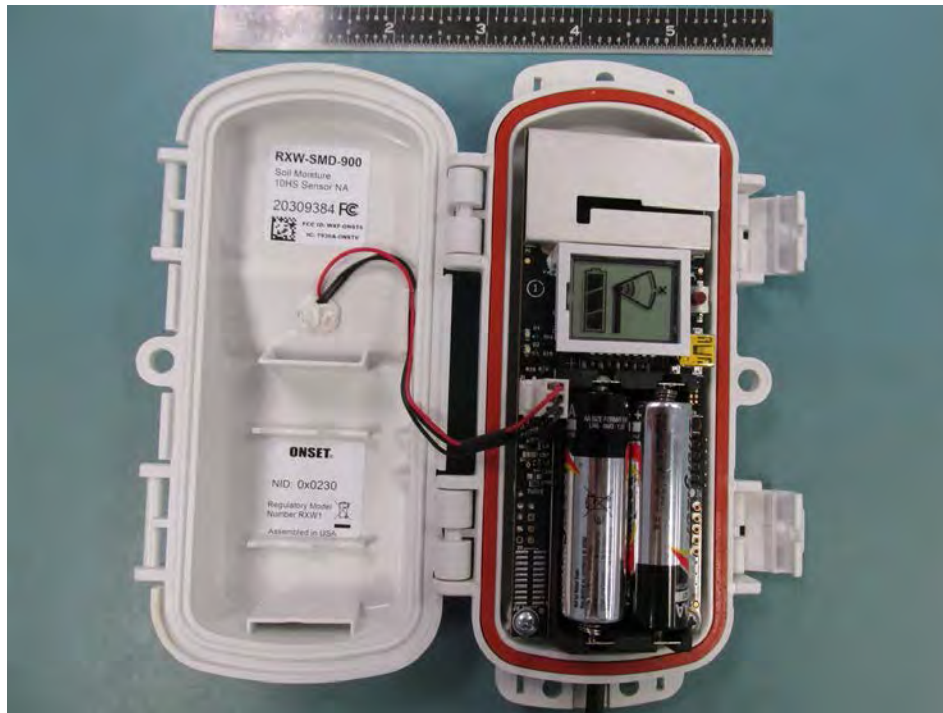
RXW-SMD-900 Housing Open
