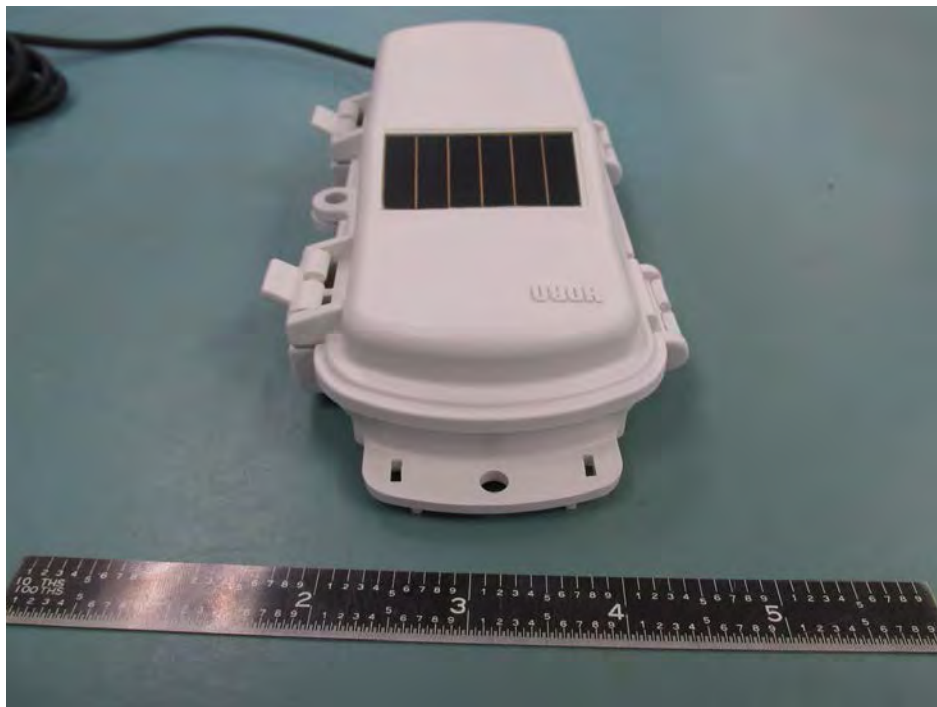
RXW-SMC-900 Housing Top
