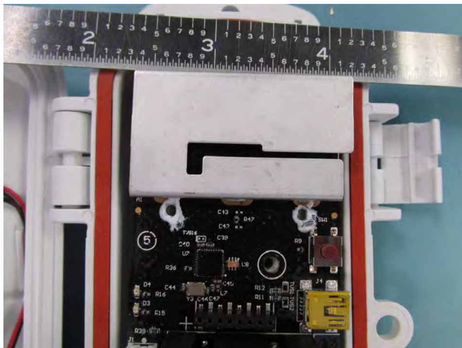
RXW-SMC-900 Radio Circuit
