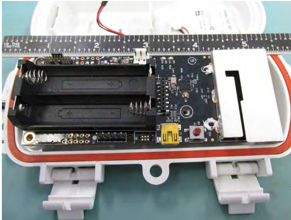
RXW-THC-900 PCB Front
