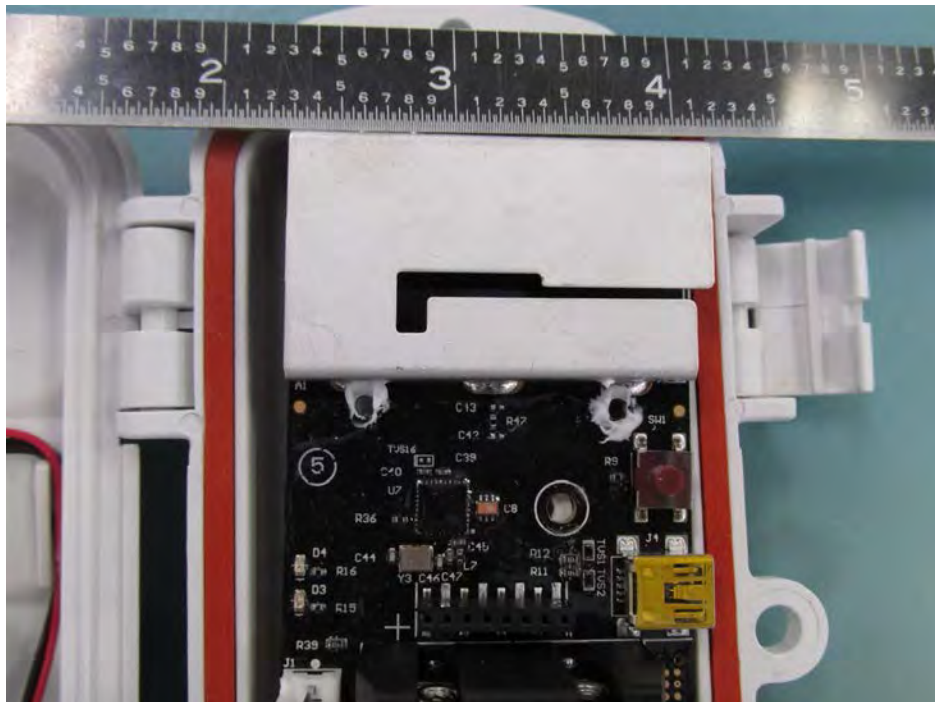
RXW-THC-900 Radio Circuit
