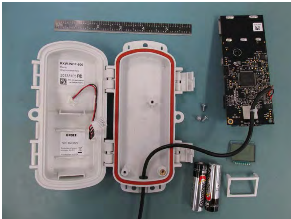
RXW-WCF-900 Exploded View
