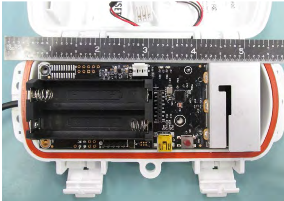
RXW-SPER-900 PCB Front
