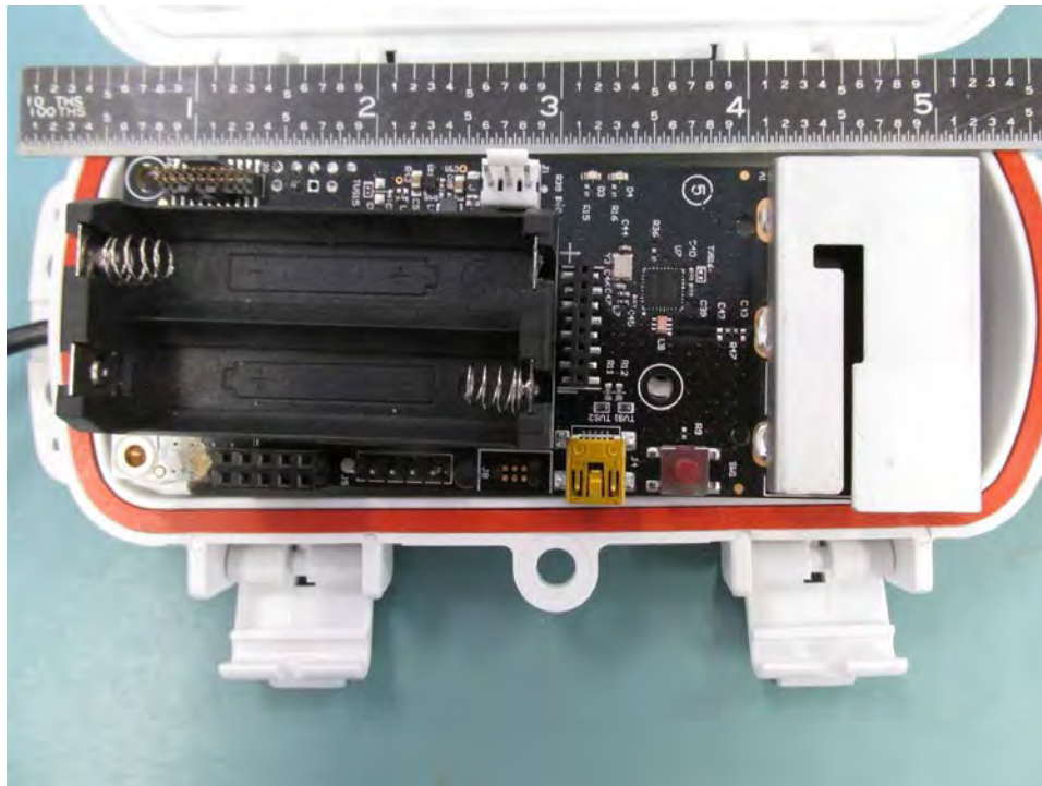
RXW-WCF-900 PCB Front
