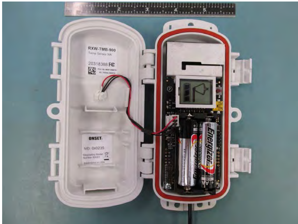
RXW-TMB-900 Housing Open
