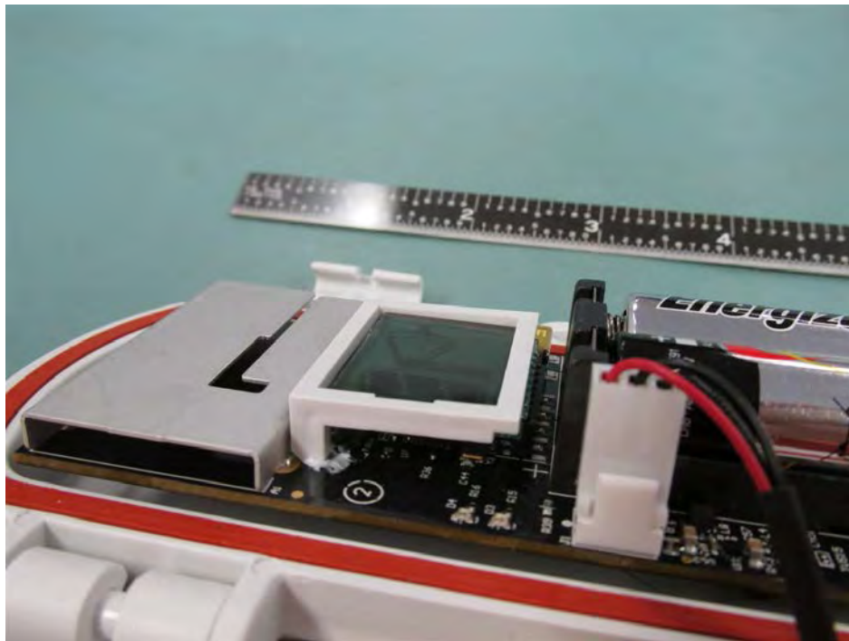
RXW-RPTR-900 Radio & LCD
