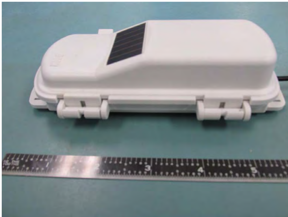
RXW-TMB-900 Housing Left Side
