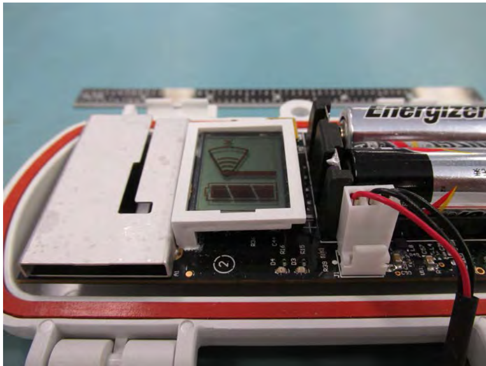
RXW-TMB-900 Radio & LCD
