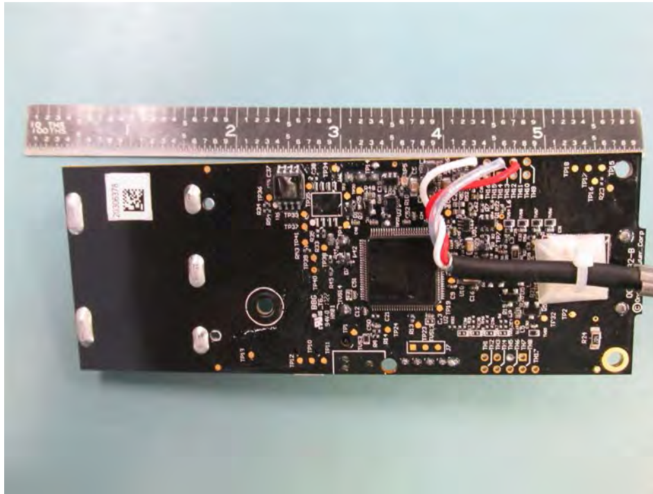
RXW-SMD-900 PCB Back
