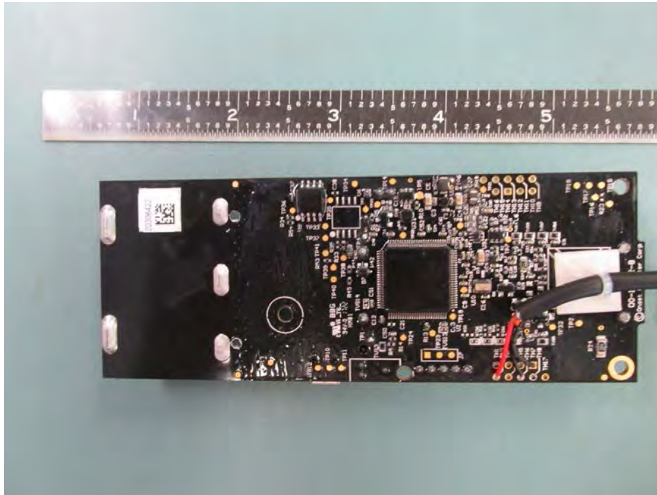
RXW-SPER-900 PCB Back
