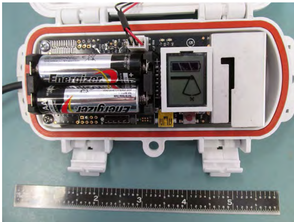
RXW-SMC-900 PCB in Housing
