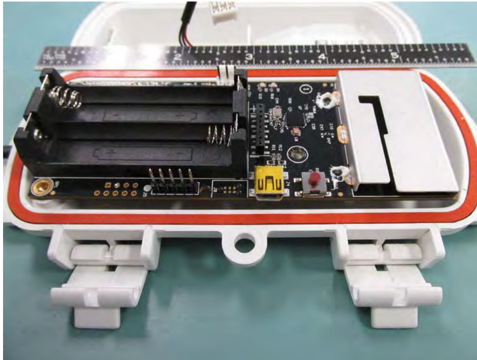
RXW-SMD-900 PCB Front
