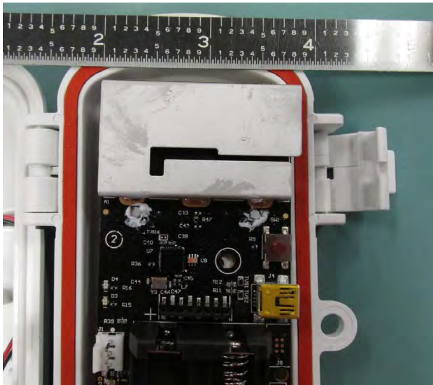
RXW-RPTR-900 Radio Circuit
