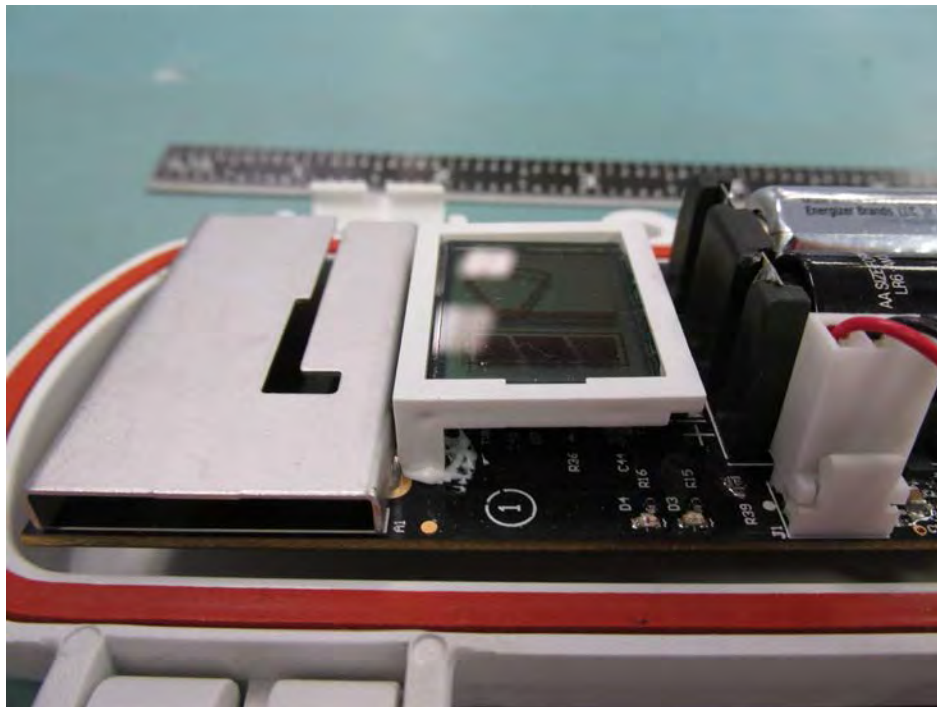
RXW-SMD-900 Radio & LCD
