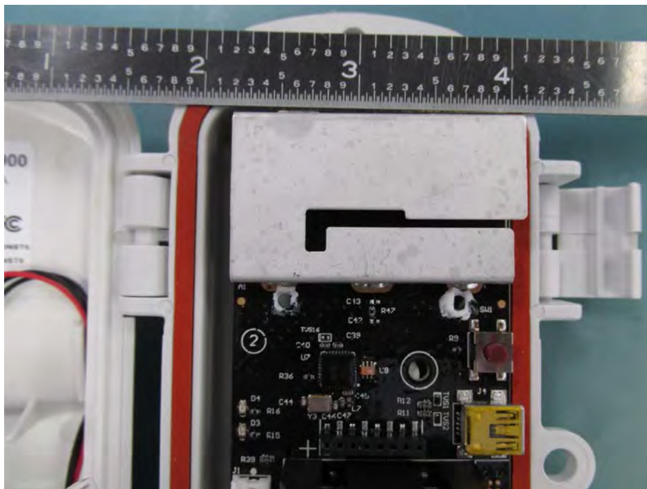
RXW-TMB-900 Radio Circuit
