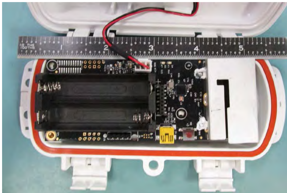
RXW-RPTR-900 PCB Front
