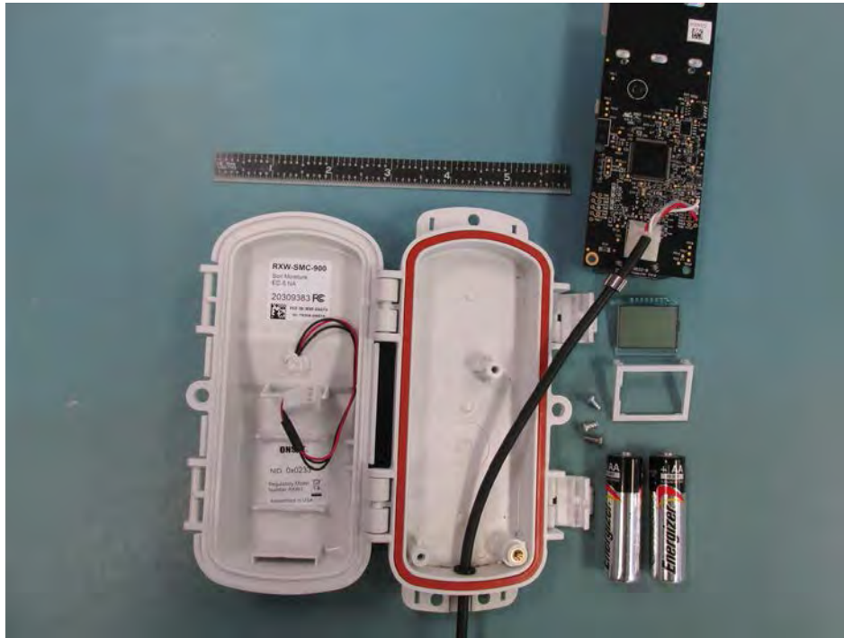
RXW-SMC-900 Exploded View
