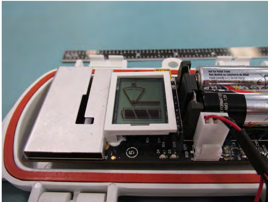
RXW-SMC-900 Radio & LCD
