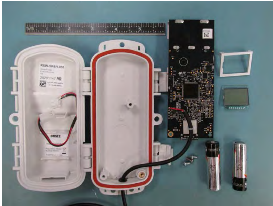
RXW-SPER-900 Exploded View
