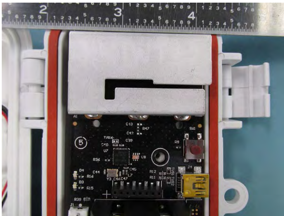
RXW-WCF-900 Radio Circuit
