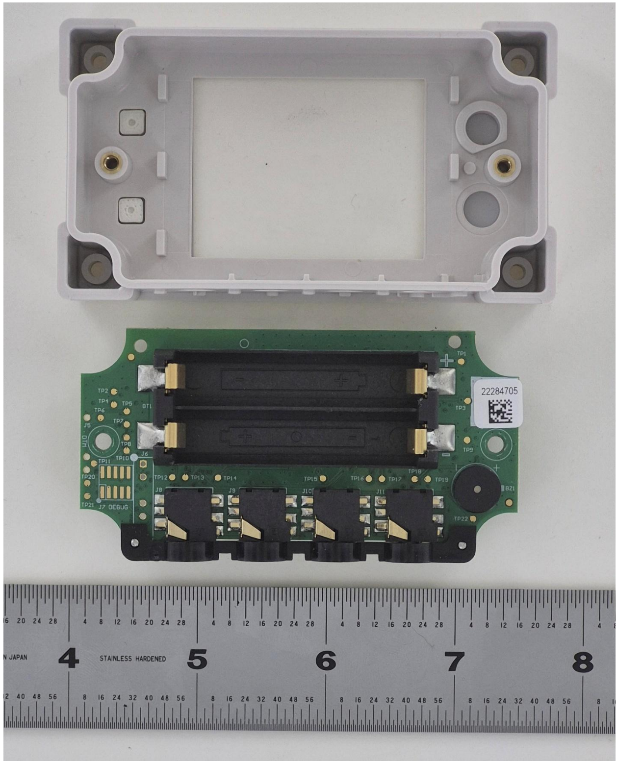
CX460 PCB Back & Housing
