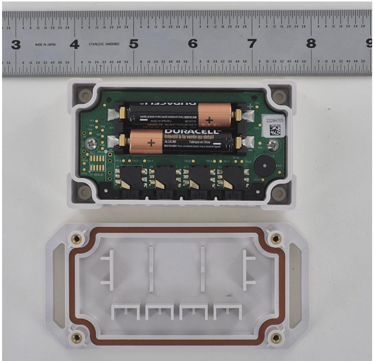
CX460 Battery Door & PCB Back
