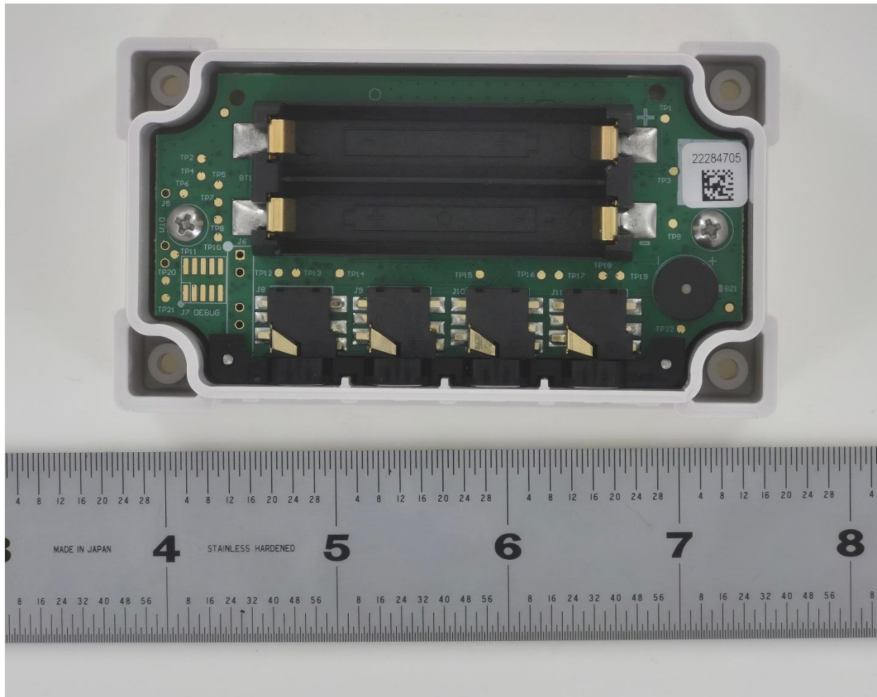
CX460 PCB Back In Housing No Batteries
