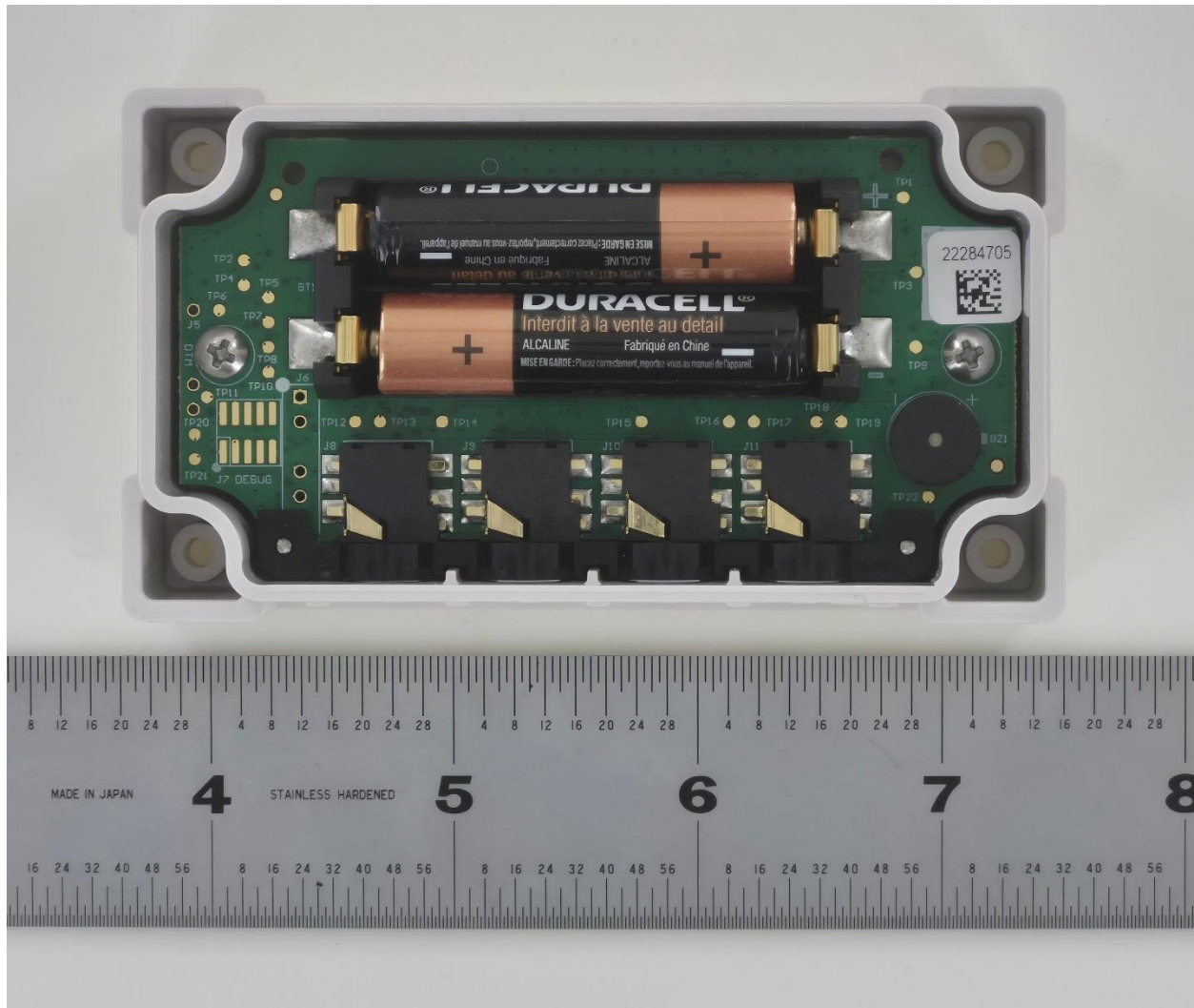
CX460 PCB Back In Housing
