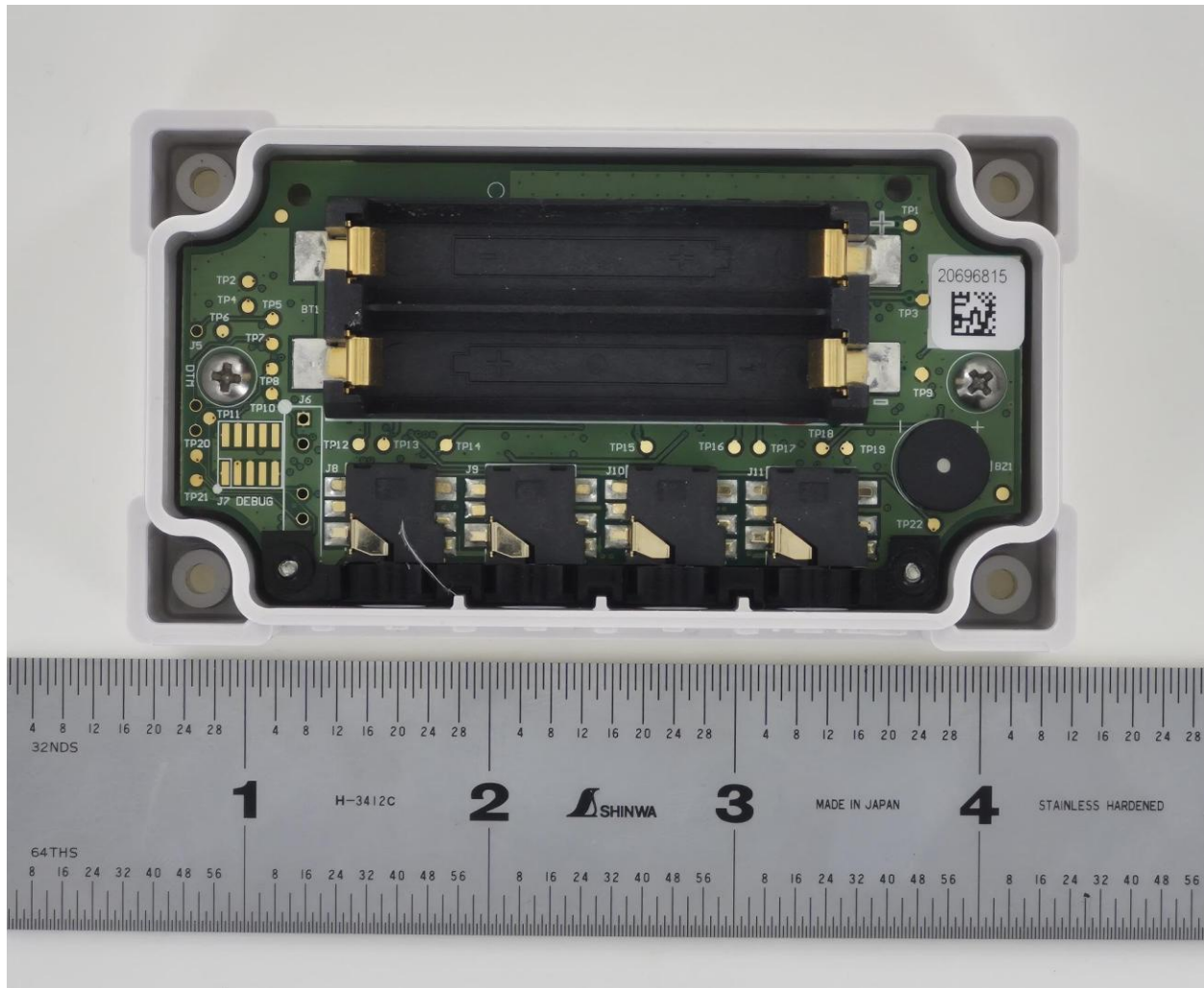
MX1105 PCB Back In Housing No Batteries
