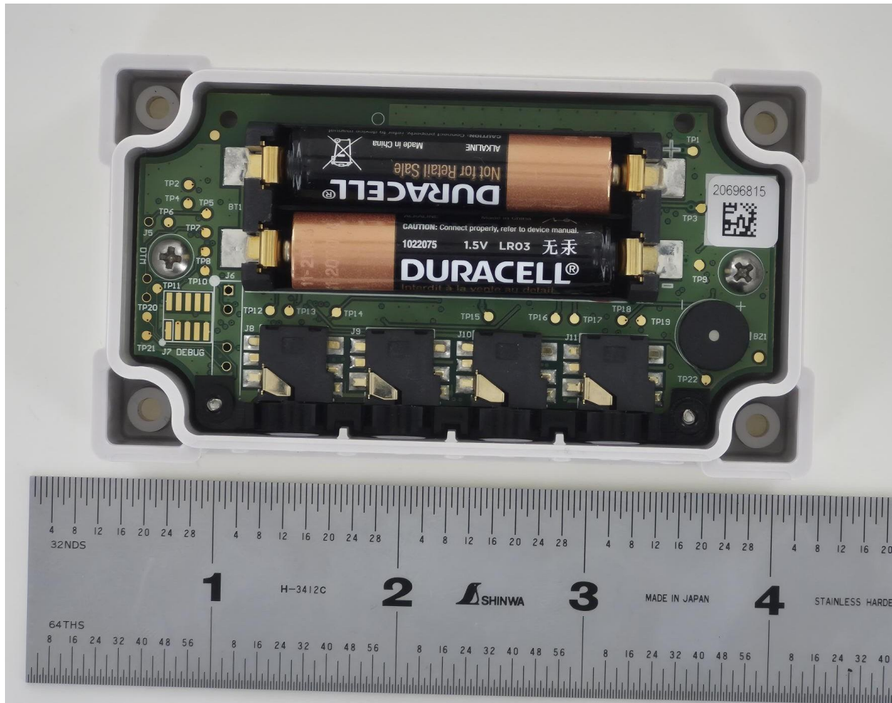
MX1105 PCB Back In Housing
