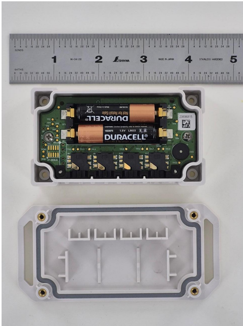
MX1105 Battery Door & PCB Back
