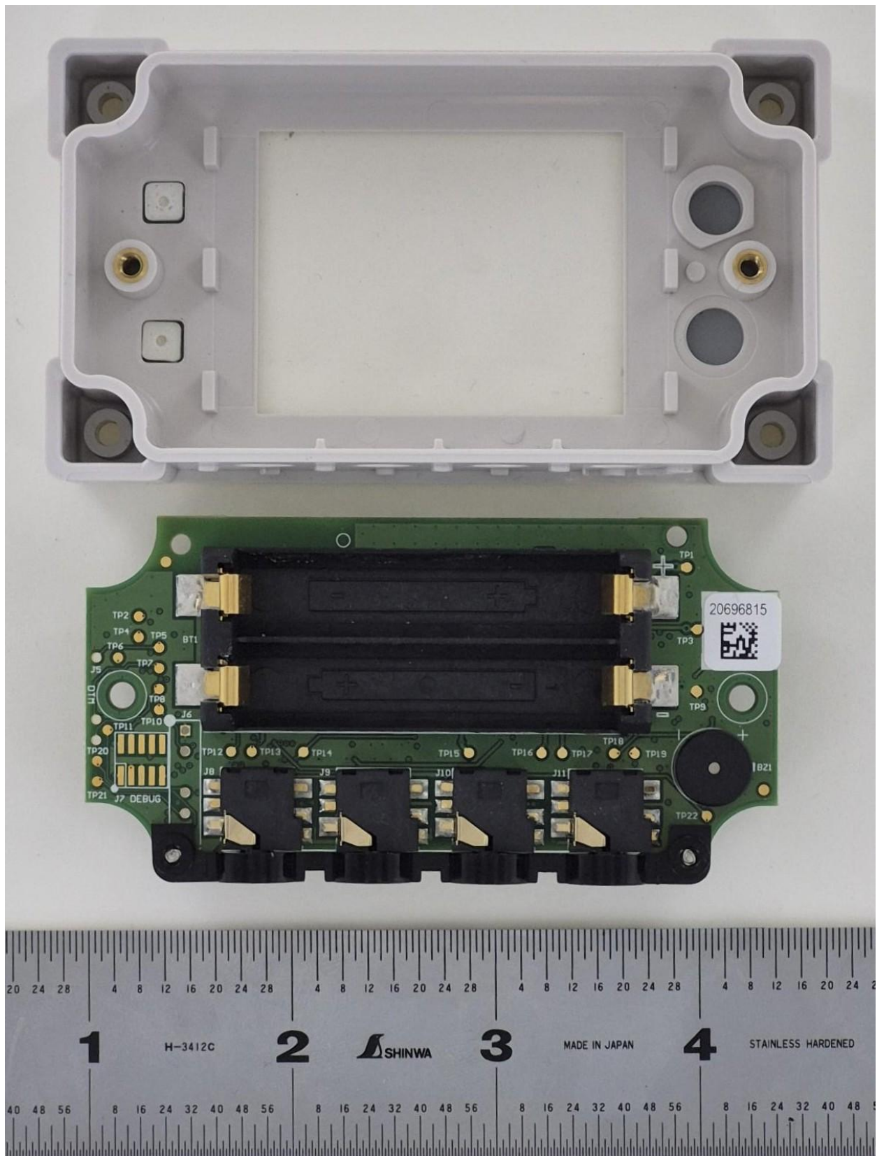
MX1105 PCB Back & Housing
