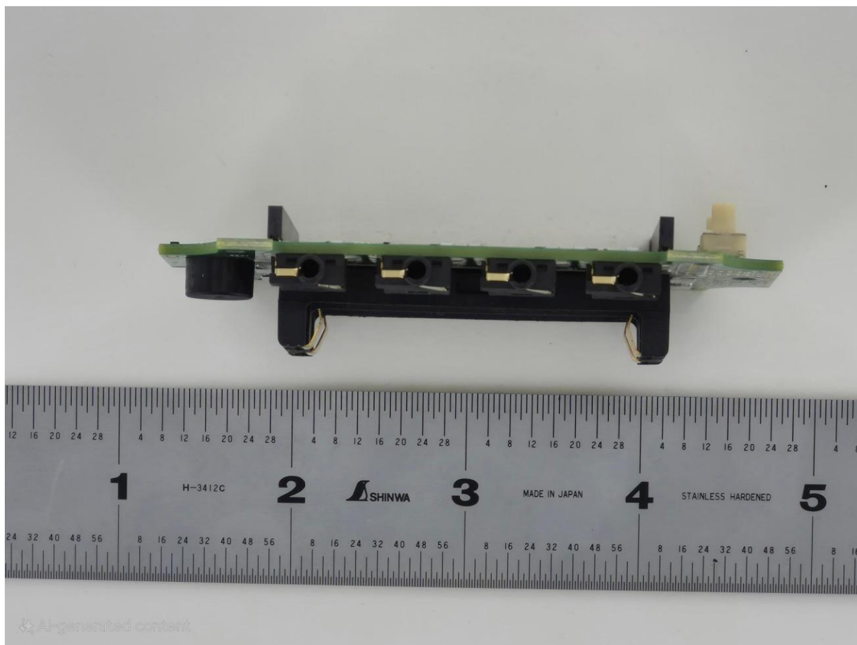
MX1105 PCB Bottom w/ No Connector Shroud
