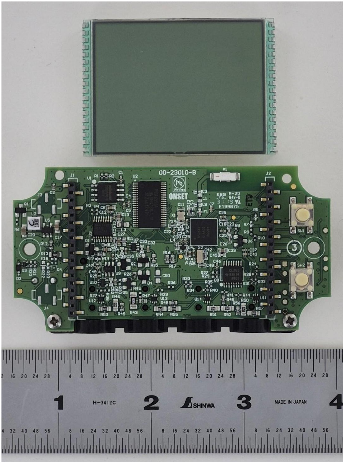
MX1105 PCB Front & LCD Removed
