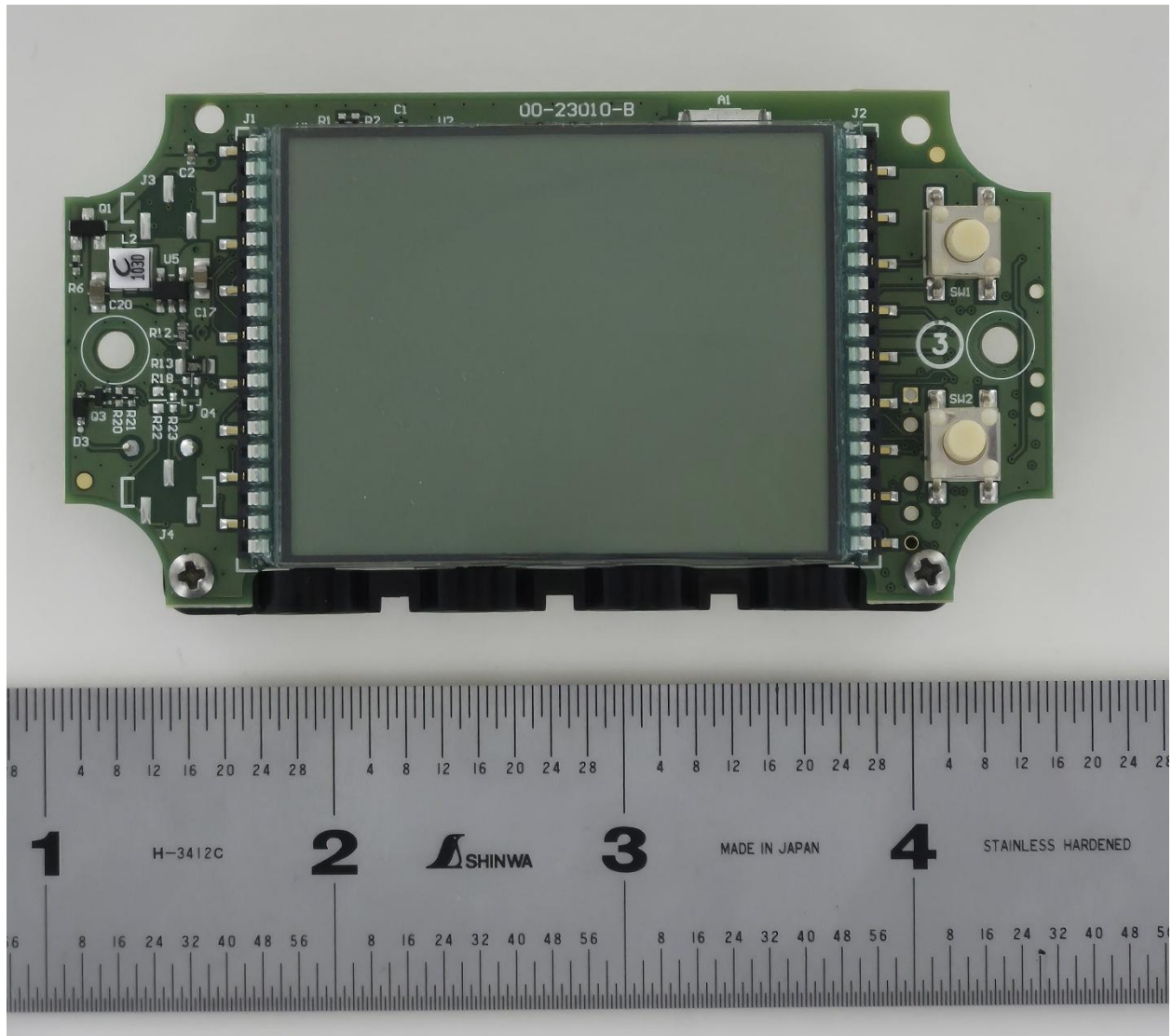
MX1105 PCB Front w/ LCD
