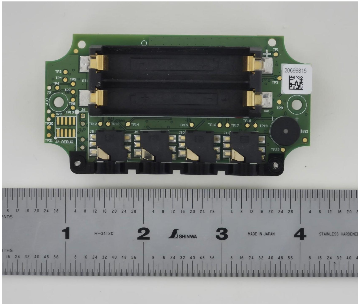
MX1105 PCB Back
