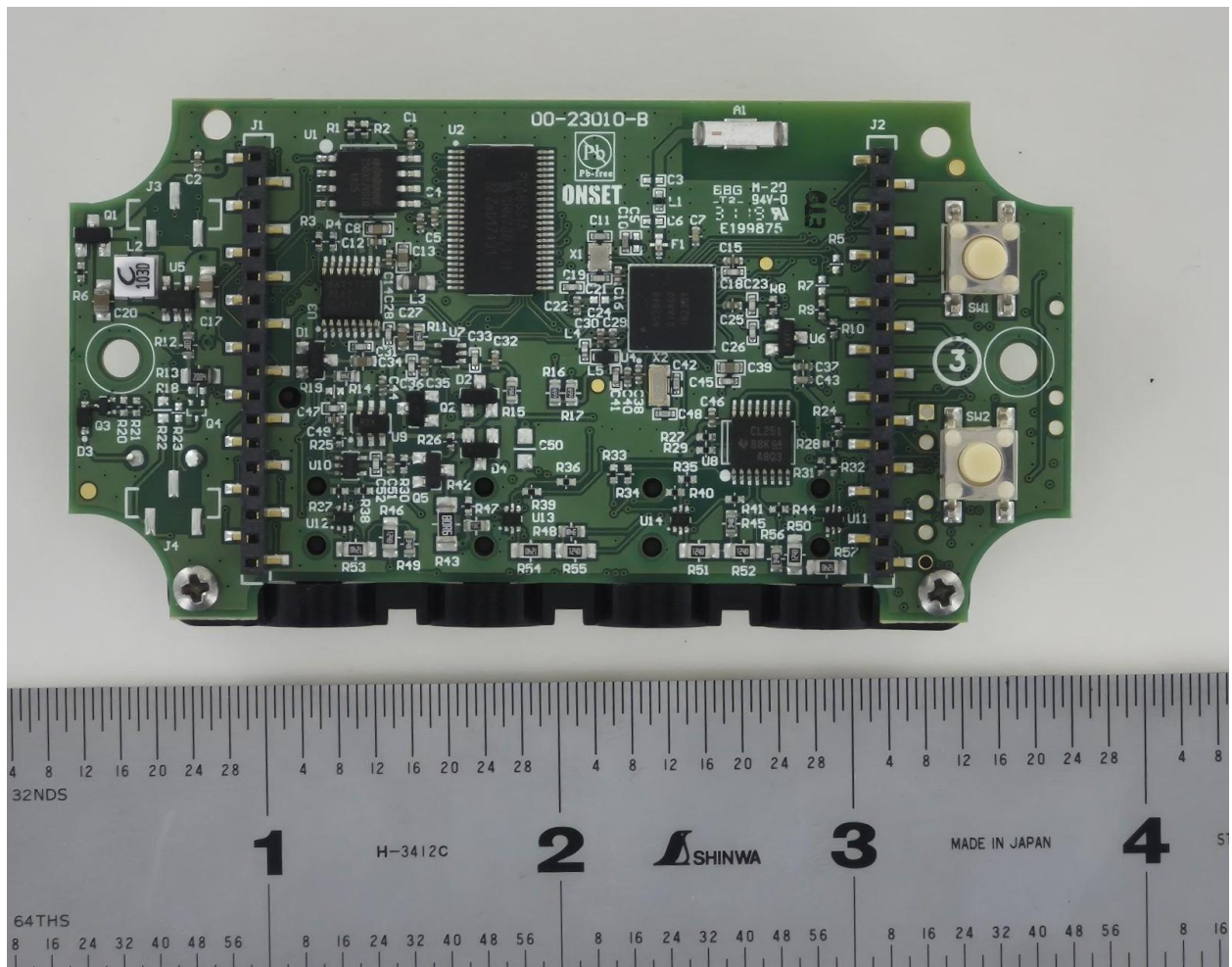
MX1105 PCB Front
