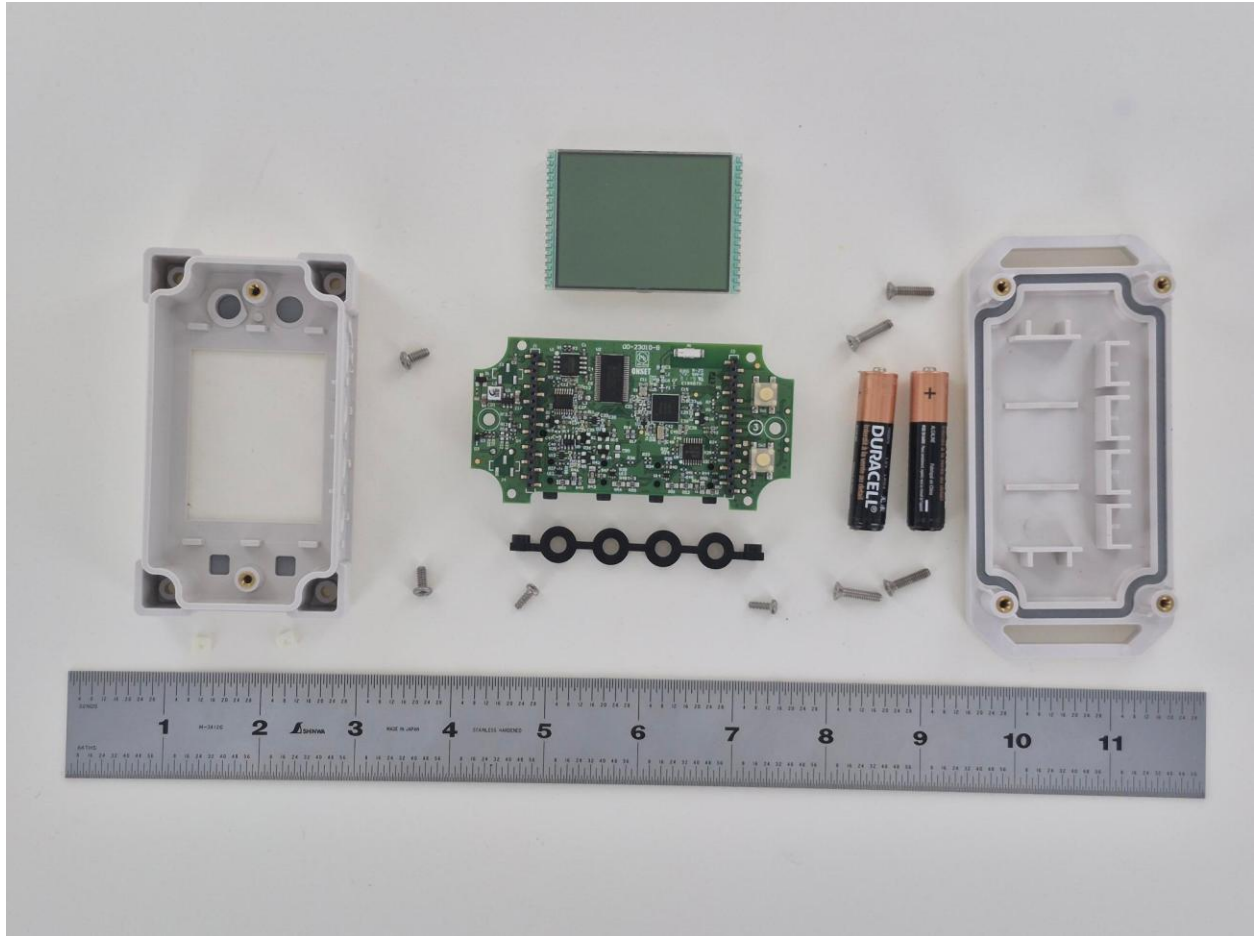
MX1105 Exploded View
