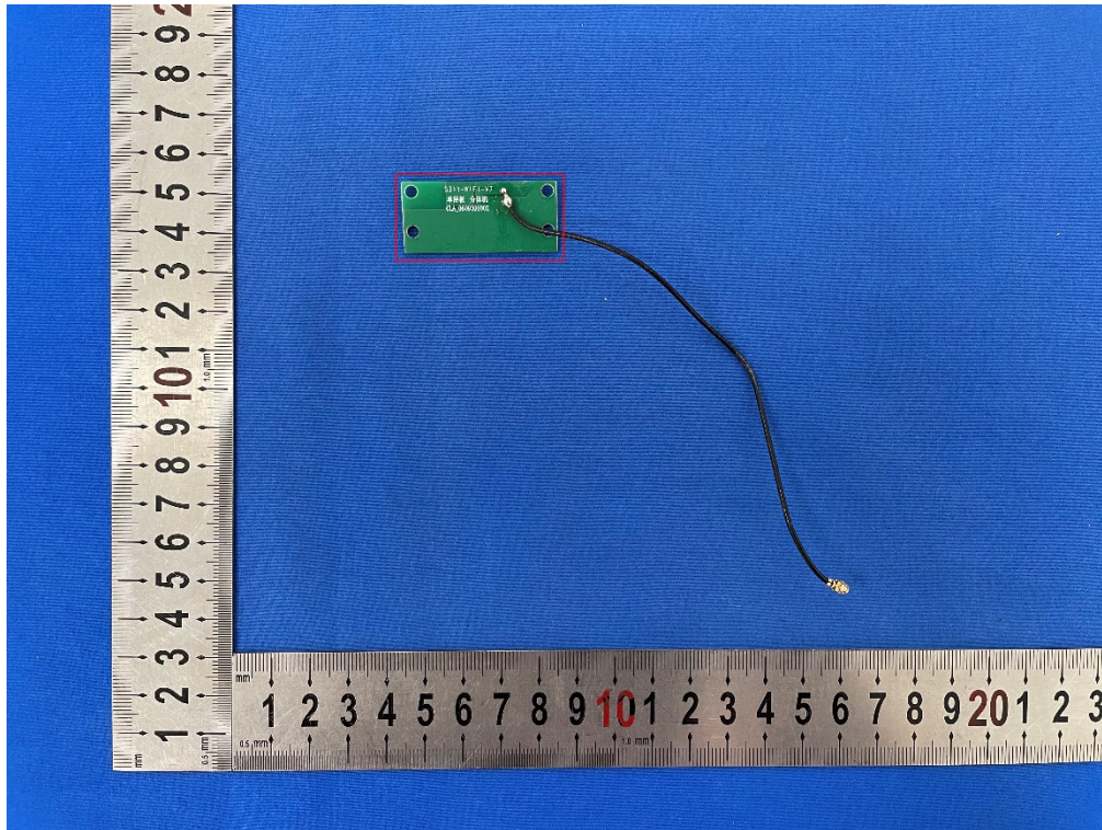
Photo 11: Internal View for BT/BLE/2.4G-WIFI/5G-WIFI Antenna
