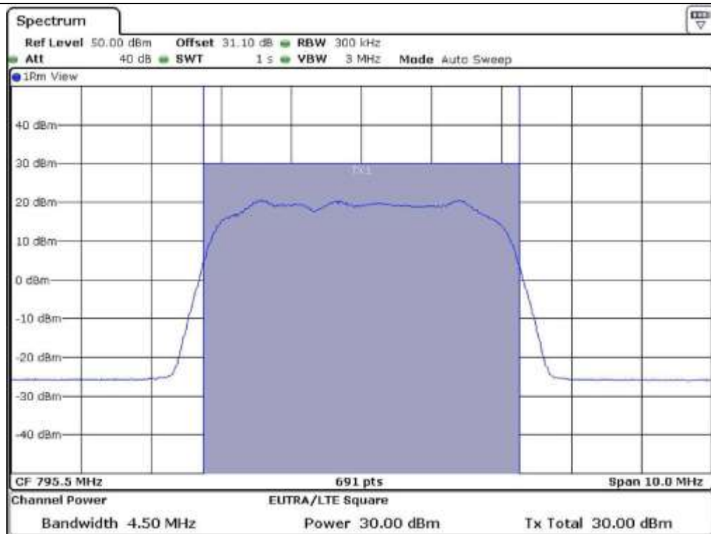
LTE 5 M - High – RF POWER OUTPUT (64 QAM)
