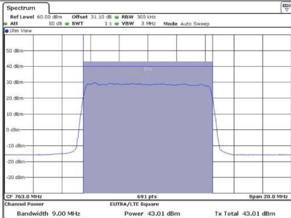
LTE 10 M – RF POWER OUTPUT (64 QAM)
