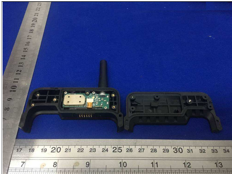
RF Antenna
