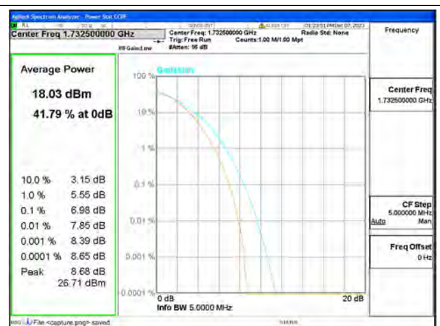
B4 / 3MHz / Mid CH / 256QAM
