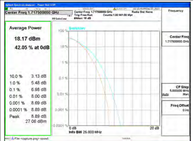
B4 / 15MHz / Low CH / 256QAM
