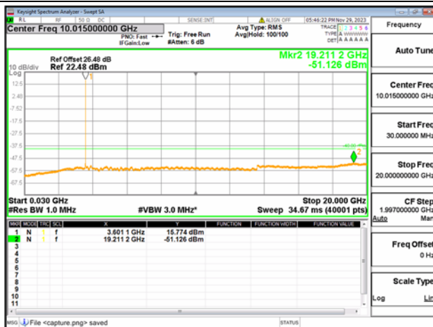
B43(3600-3700)-30M-20G / 10MHz / Low CH / QPSK
