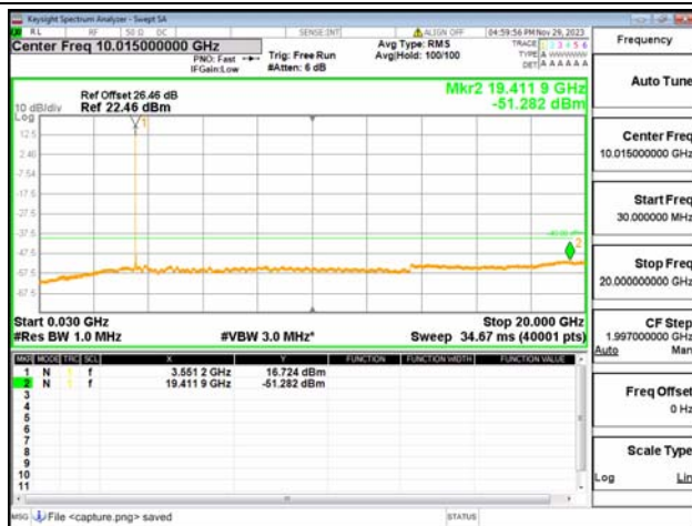
B42(3550-3600)-30M-20G / 10MHz / Low CH / QPSK
