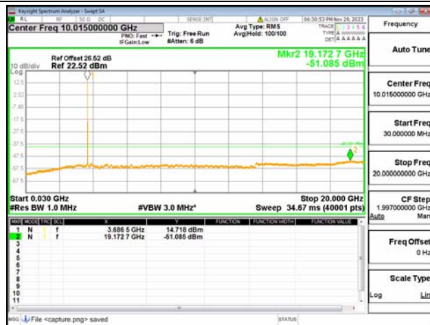
B43(3600-3700)-30M-20G / 15MHz / High CH / QPSK
