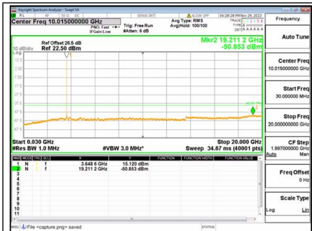
B43(3600-3700)-30M-20G / 5MHz / Mid CH / QPSK
