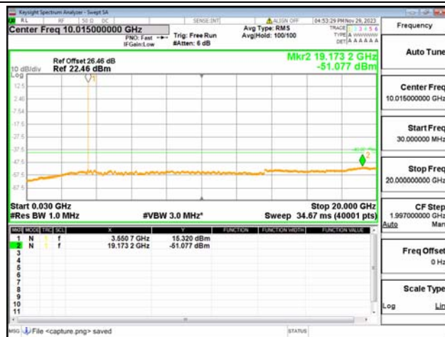
B42(3550-3600)-30M-20G / 5MHz / Low CH / QPSK
