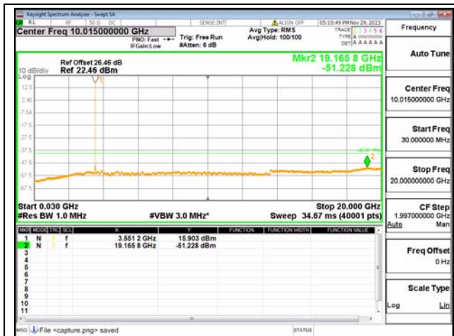
B42(3550-3600)-30M-20G / 15MHz / Low CH / QPSK
