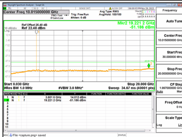
B43(3600-3700)-30M-20G / 20MHz / Low CH / QPSK
