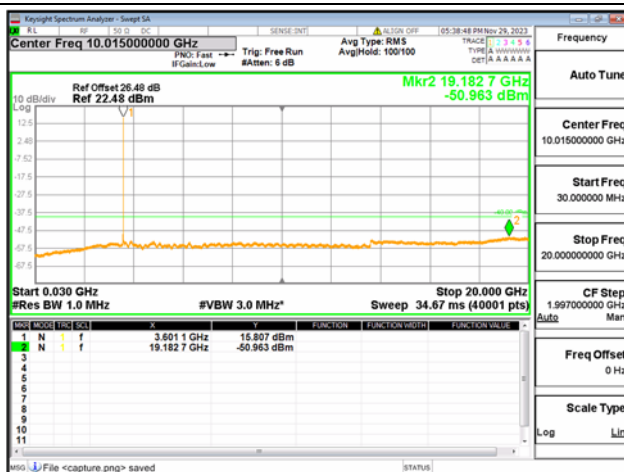
B43(3600-3700)-30M-20G / 5MHz / Low CH / QPSK
