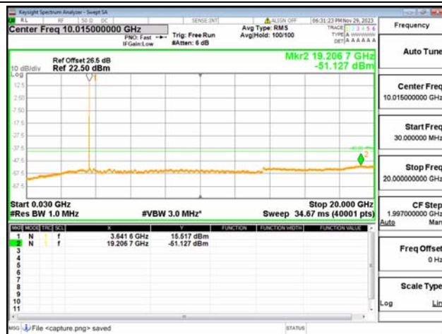
B43(3600-3700)-30M-20G / 20MHz / Mid CH / QPSK
