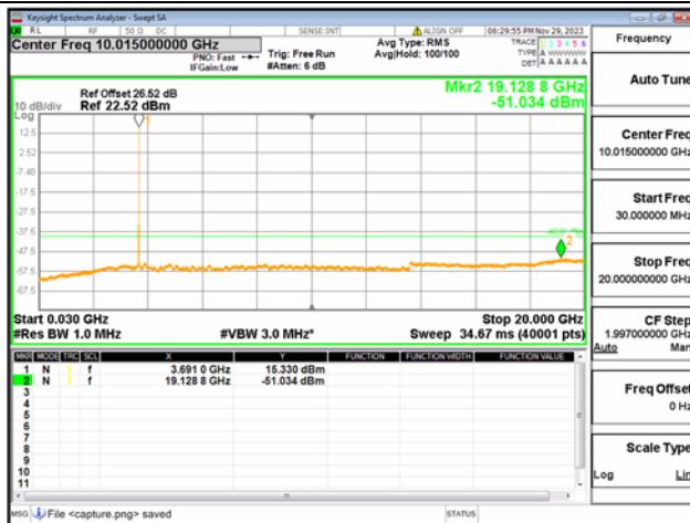
B43(3600-3700)-30M-20G / 10MHz / High CH / QPSK
