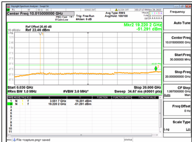
B42(3550-3600)-30M-20G / 20MHz / Low CH / QPSK
