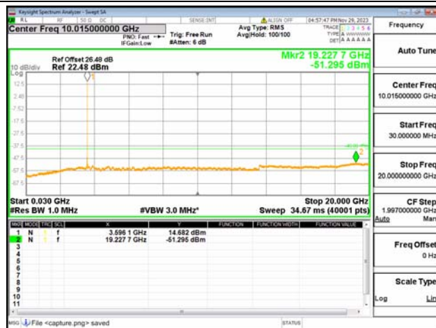
B42(3550-3600)-30M-20G / 5MHz / High CH / QPSK
