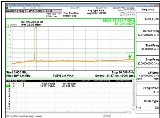
B48-30M-20G / 5MHz / High CH / QPSK
