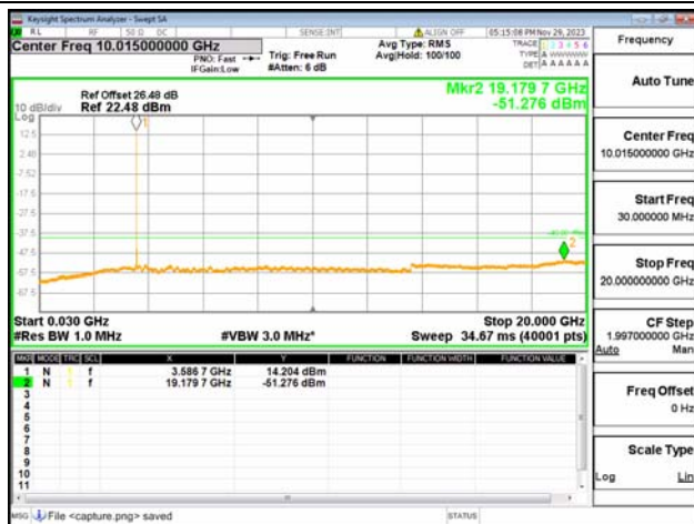
B42(3550-3600)-30M-20G / 15MHz / High CH / QPSK
