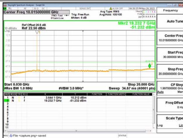
B43(3600-3700)-30M-20G / 15MHz / Mid CH / QPSK
