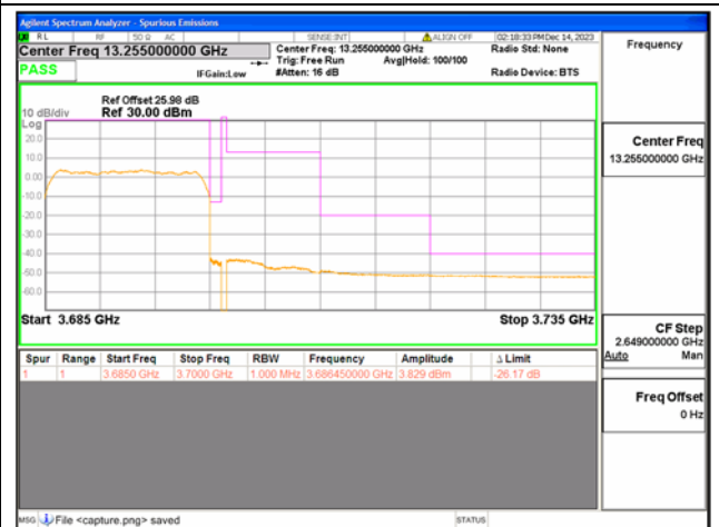
B43(3600-3700) / 15MHz / High CH / QPSK / FULL RB
