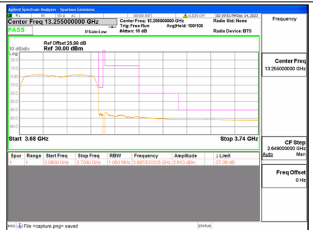
B43(3600-3700) / 20MHz / High CH / QPSK / FULL RB
