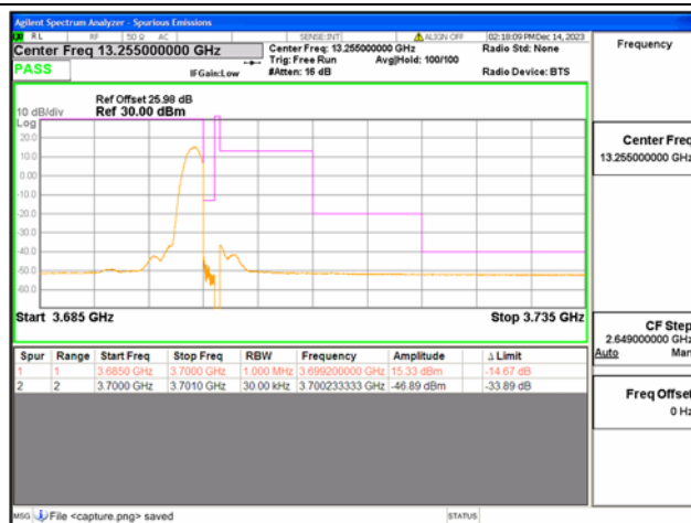
B43(3600-3700) / 15MHz / High CH / QPSK / 1 RB
