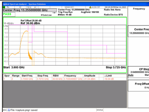
B43(3600-3700) / 5MHz / High CH / QPSK / 1 RB
