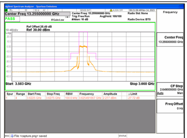
B48 / 5MHz / Mid CH / QPSK / FULL RB
