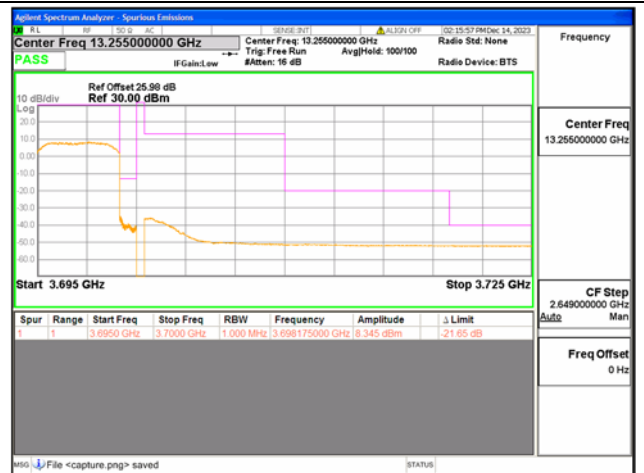
B43(3600-3700) / 5MHz / High CH / QPSK / FULL RB
