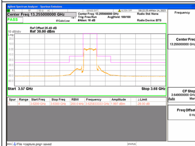
B48 / 10MHz / Mid CH / QPSK / FULL RB
