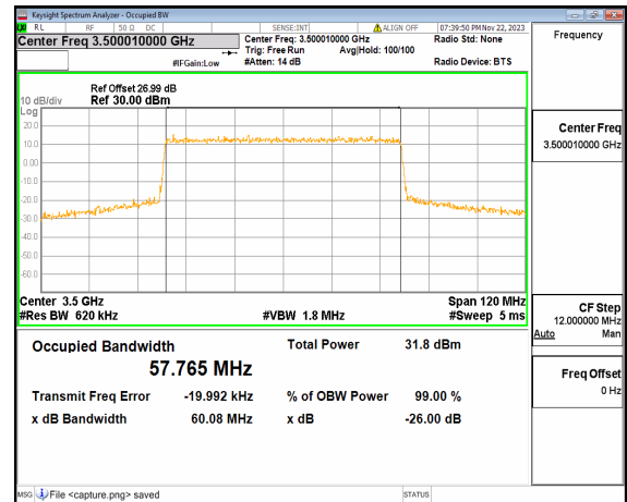
n77(3450-3550MHz) 60M CP-OFDM QPSK Outer_Full Mid
