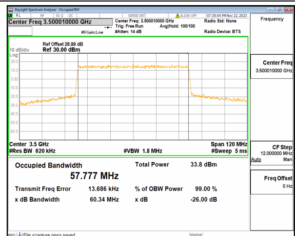
n77(3450-3550MHz) 60M DFT-s-OFDM QPSK Outer_Full Mid
