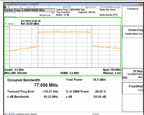
n77(3450-3550MHz) 80M DFT-s-OFDM QPSK Outer_Full Mid
