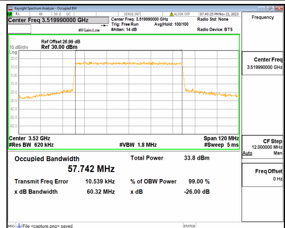
n77(3450-3550MHz) 60M DFT-s-OFDM QPSK Outer_Full High
