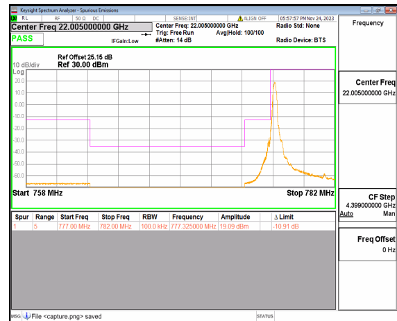
n13 5M DFT-s-OFDM BPSK Edge_1RB_Left Low
