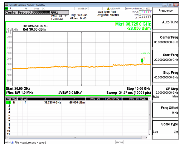
n77(3700-3980MHz) (20GHz-40GHz) 100M DFT-s-OFDM QPSK Edge_1RB_Left Mid
