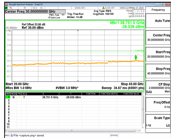
n77(3700-3980MHz) (20GHz-40GHz) 100M DFT-s-OFDM QPSK Edge_1RB Left High
