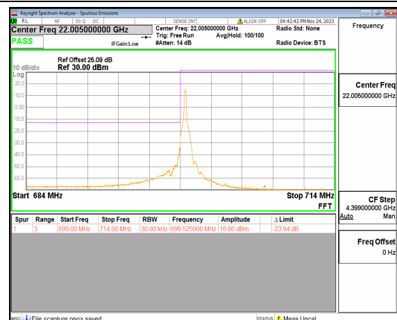
n12 15M DFT-s-OFDM BPSK Edge_1RB_Left Low
