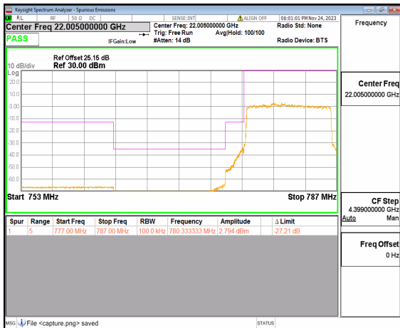
n13 10M DFT-s-OFDM BPSK Outer_Full Low
