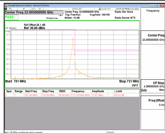
n12 15M DFT-s-OFDM QPSK Edge_1RB_Right High
