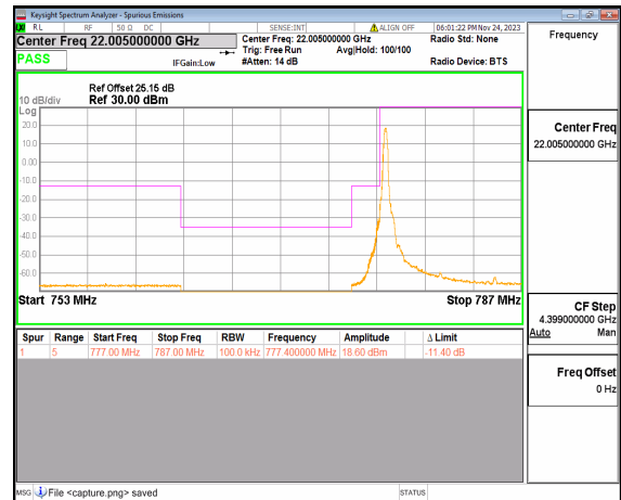
n13 10M DFT-s-OFDM BPSK Edge_1RB_Left Low
