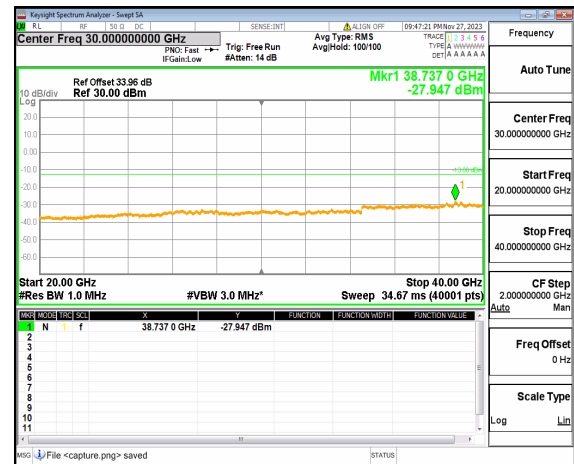
n77(3700-3980MHz) (20GHz-40GHz) 100M DFT-s-OFDM QPSK Edge_1RB_Right Mid
