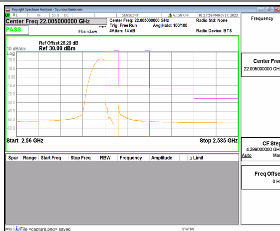
n7 10M DFT-s-OFDM BPSK Edge_1RB_Right High
