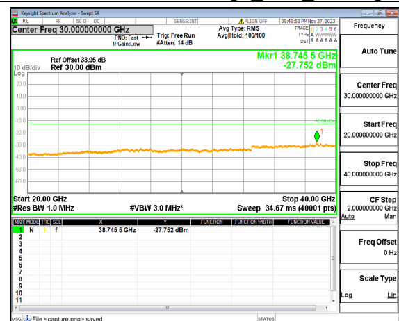
n77(3700-3980MHz) (20GHz-40GHz) 100M DFT-s-OFDM BPSK Edge_1RB_Right High
