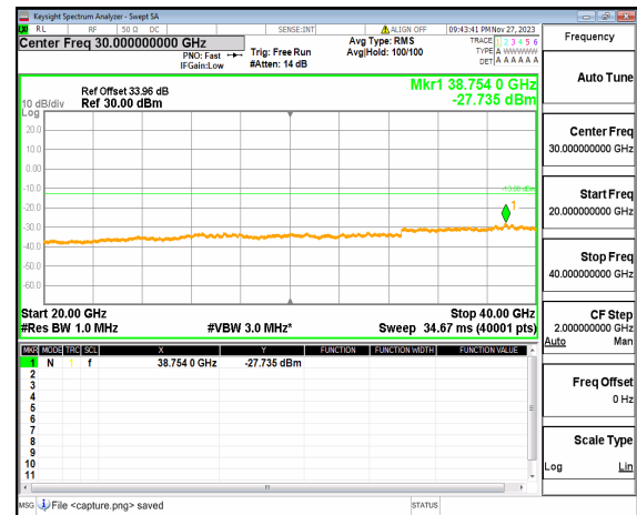
n77(3700-3980MHz) (20GHz-40GHz) 100M DFT-s-OFDM BPSK Edge_1RB_Left Mid
