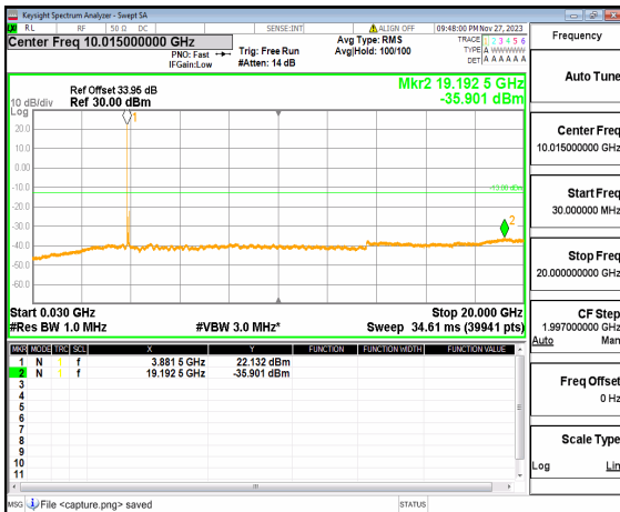
n77(3700-3980MHz) (30MHz-20GHz) 100M DFT-s-OFDM BPSK Edge_1RB_Left High
