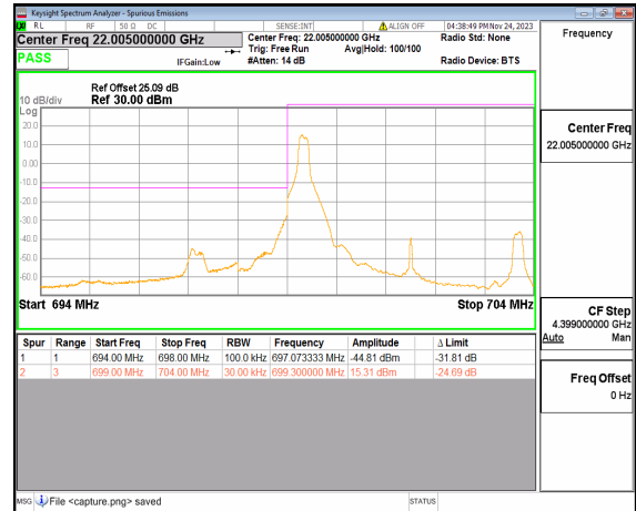
n12 5M DFT-s-OFDM BPSK Edge_1RB_Left Low
