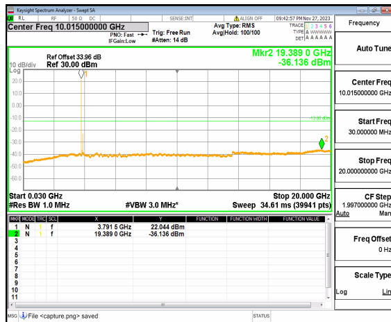
n77(3700-3980MHz) (30MHz-20GHz) 100M DFT-s-OFDM BPSK Edge_1RB_Left Mid
