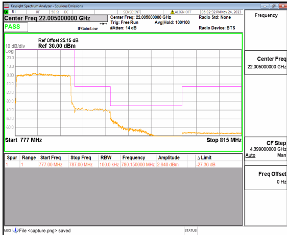
n13 10M DFT-s-OFDM BPSK Outer_Full High
