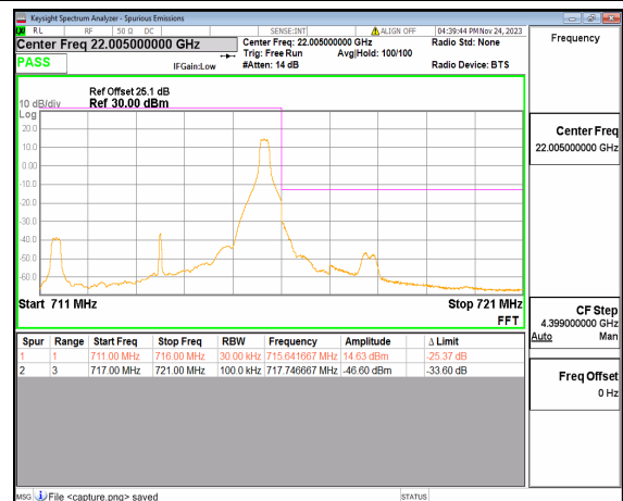
n12 5M DFT-s-OFDM BPSK Edge_1RB_Right High
