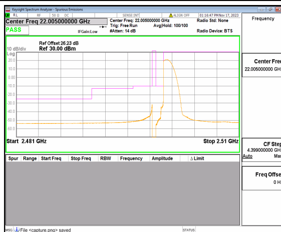
n7 10M DFT-s-OFDM BPSK Edge_1RB_Left Low
