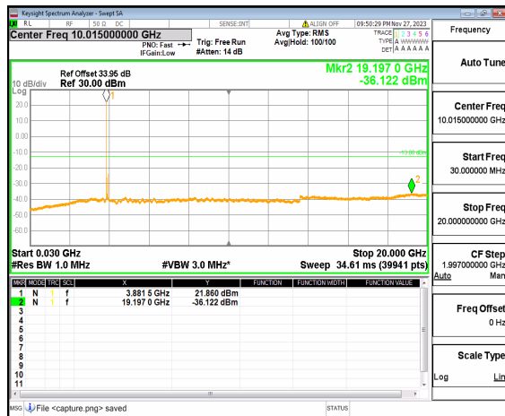
n77(3700-3980MHz) (30MHz-20GHz) 100M DFT-s-OFDM QPSK Edge_1RB Left High
