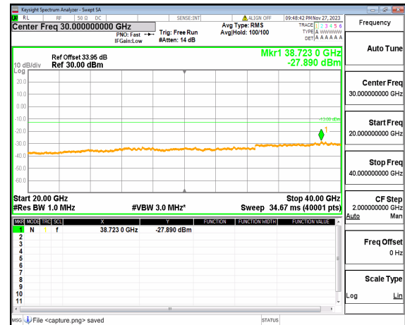
n77(3700-3980MHz) (20GHz-40GHz) 100M DFT-s-OFDM BPSK Edge_1RB_Left High
