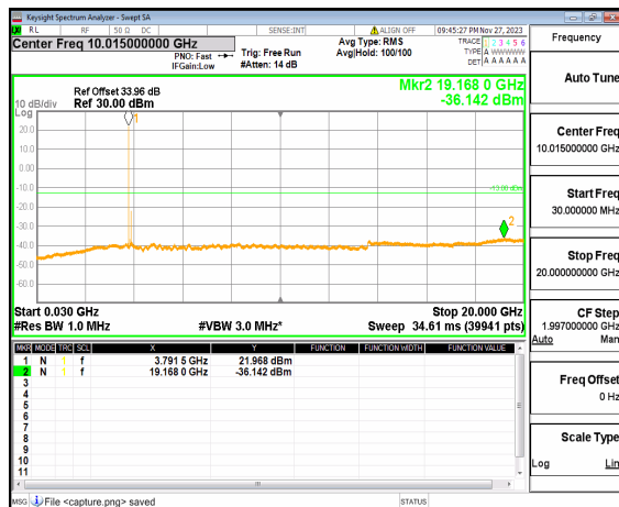
n77(3700-3980MHz) (30MHz-20GHz) 100M DFT-s-OFDM QPSK Edge_1RB_Left Mid
