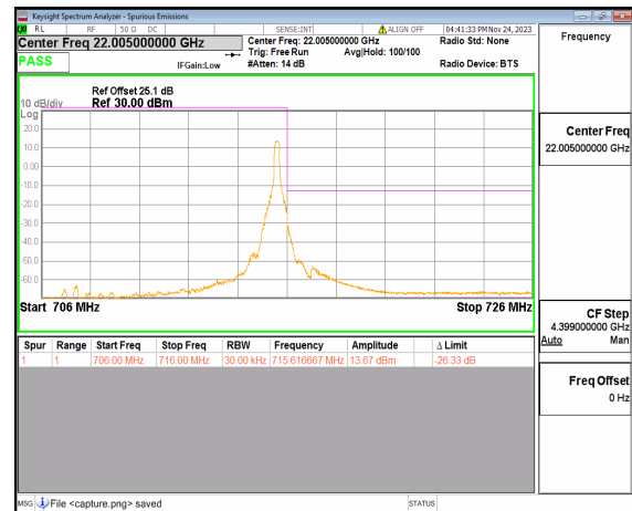
n12 10M DFT-s-OFDM BPSK Edge_1RB_Right High
