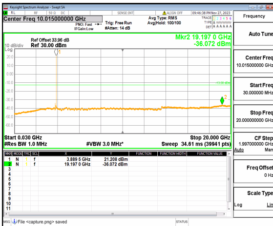
n77(3700-3980MHz) (30MHz-20GHz) 100M DFT-s-OFDM QPSK Edge_1RB_Right Mid
