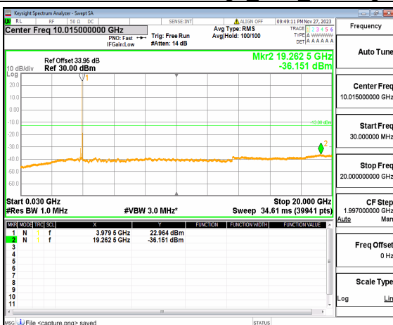
n77(3700-3980MHz) (30MHz-20GHz) 100M DFT-s-OFDM BPSK Edge_1RB_Right High
