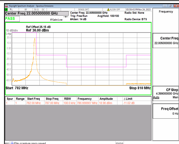
n13 5M DFT-s-OFDM BPSK Edge_1RB_Right High
