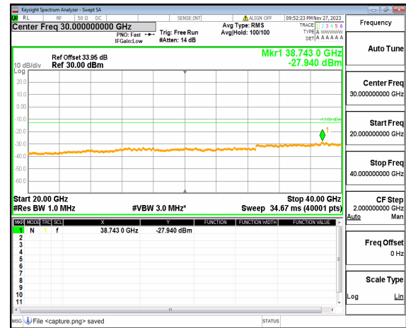
n77(3700-3980MHz) (20GHz-40GHz) 100M DFT-s-OFDM QPSK Edge_1RB Right High
