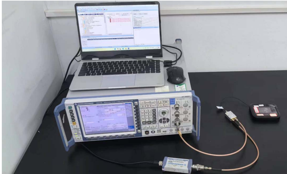
Test Setup
