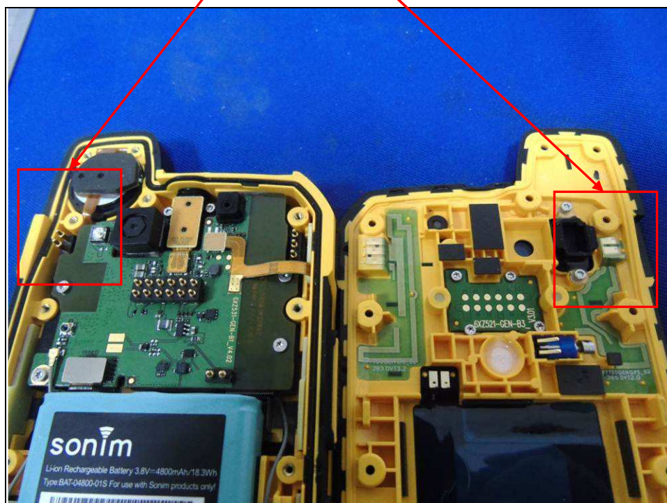
UMTS Band V/LTE B5/GPS (RX) Antenna
