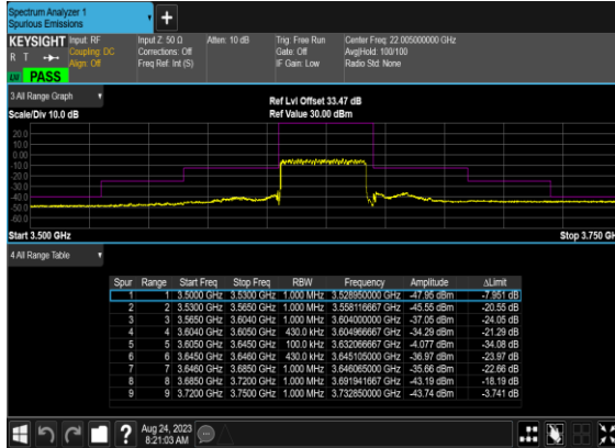
N48(40M)_DFT-s- OFDM_BPSK_Outer_Full_Mid_CH
