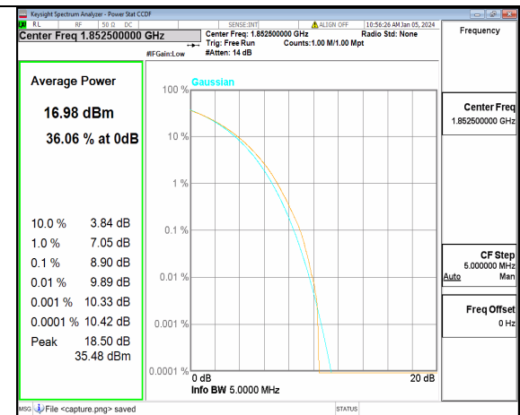
n2 5M CP-OFDM 256QAM Outer_Full Low
