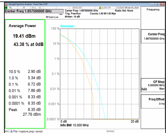
n2 15M DFT-s-OFDM 256QAM Outer_Full Low
