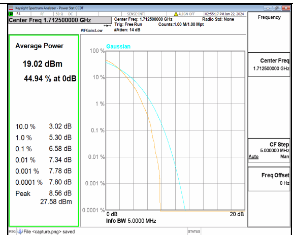
n66 5M DFT-s-OFDM 256QAM Outer_Full Low
