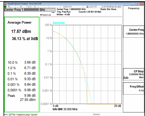
n2 20M CP-OFDM 256QAM Outer_Full Mid
