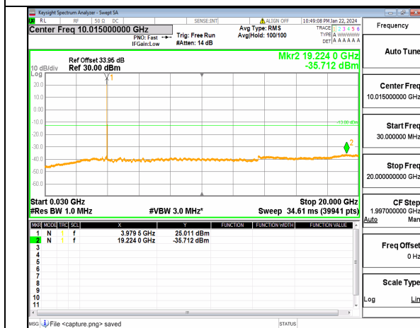
n77(3700-3980MHz) (30MHz-20GHz) 20M DFT-s-OFDM BPSK Inner_1RB_Right High
