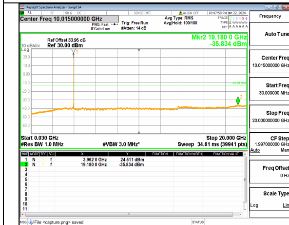
n77(3700-3980MHz) (30MHz-20GHz) 20M DFT-s-OFDM BPSK Inner_1RB_Left High
