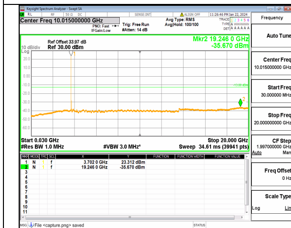
n77(3700-3980MHz) (30MHz-20GHz) 60M DFT-s-OFDM BPSK Inner_1RB_Left Low
