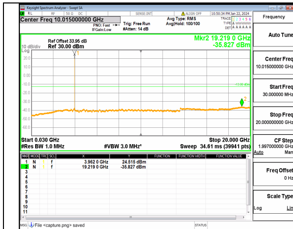
n77(3700-3980MHz) (30MHz-20GHz) 20M DFT-s-OFDM QPSK Inner_1RB_Left High
