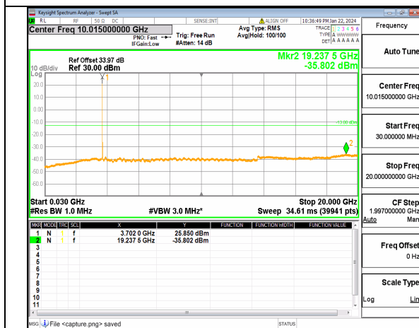
n77(3700-3980MHz) (30MHz-20GHz) 20M DFT-s-OFDM BPSK Inner_1RB_Left Low
