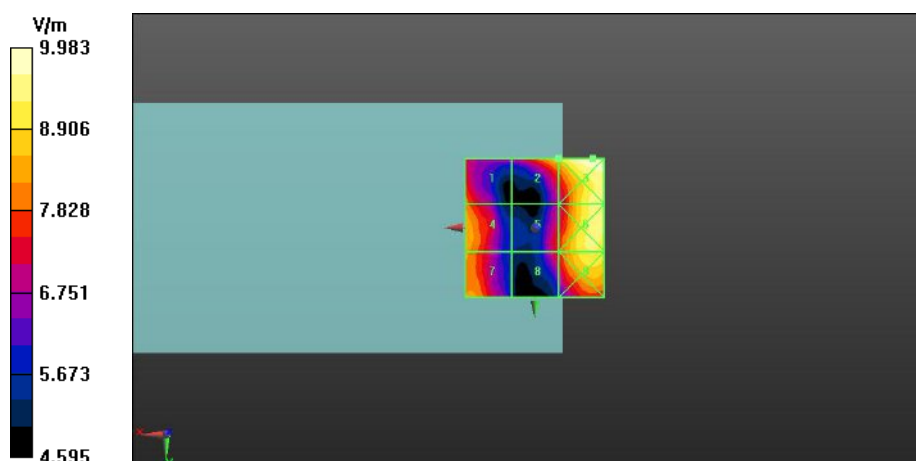
Fig A.9 HAC RF E-Field LTE Band 38
