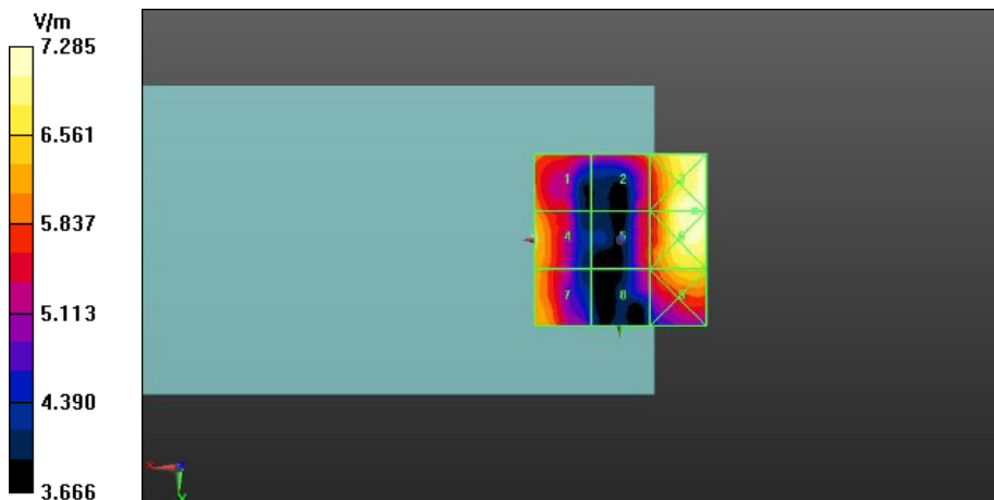
Fig A.14 HAC RF E-Field LTE Band 41
