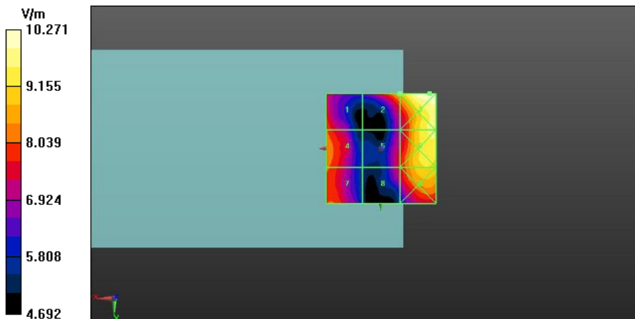
Fig A.8 HAC RF E-Field LTE Band 38
