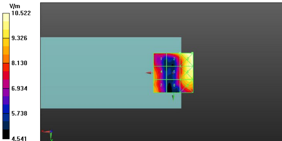
Fig A.13 HAC RF E-Field LTE Band 41
