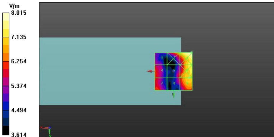
Fig A.11 HAC RF E-Field LTE Band 41
