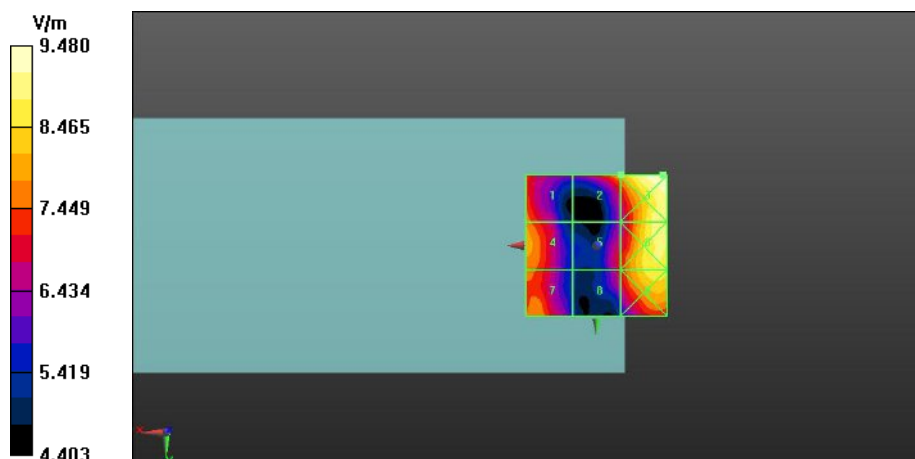
Fig A.7 HAC RF E-Field LTE Band 38
