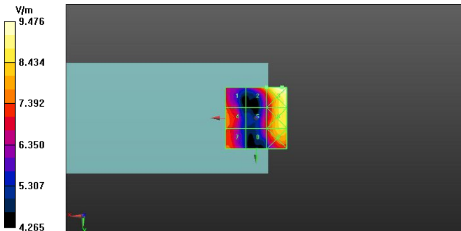
Fig A.12 HAC RF E-Field LTE Band 41
