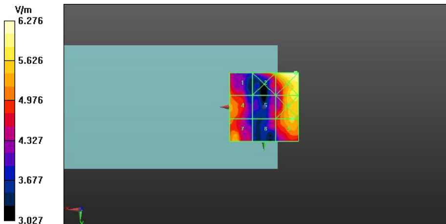
Fig A.10 HAC RF E-Field LTE Band 41
