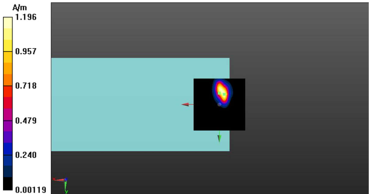
Fig A.14 T-Coil LTE-Band 26-Z
