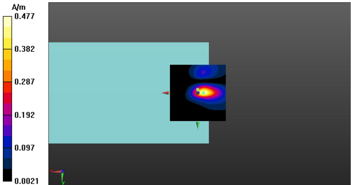
Fig A.16 T-Coil LTE-Band 38-Y
