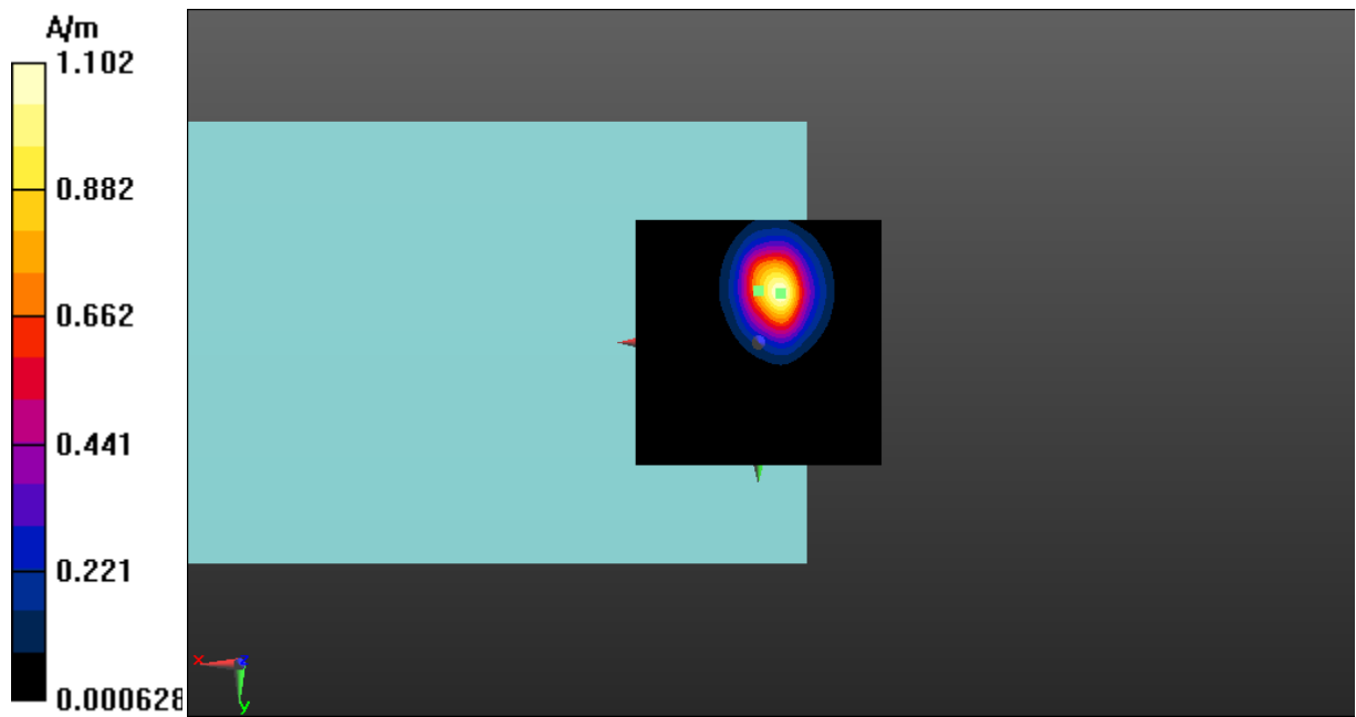
Fig A.17 T-Coil LTE-Band 41-Z
