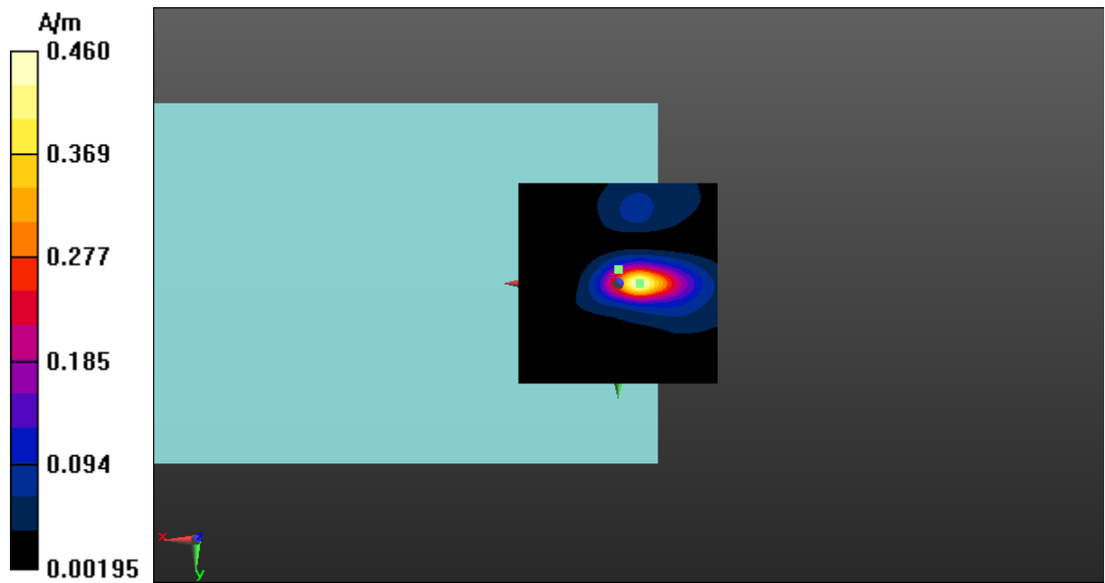
Fig A.15 T-Coil LTE-Band 66-Y
