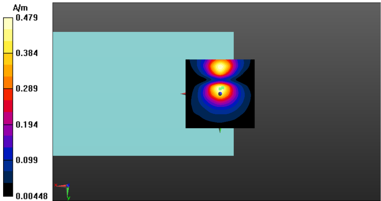
Fig A.12 T-Coil LTE-Band 14-Y
