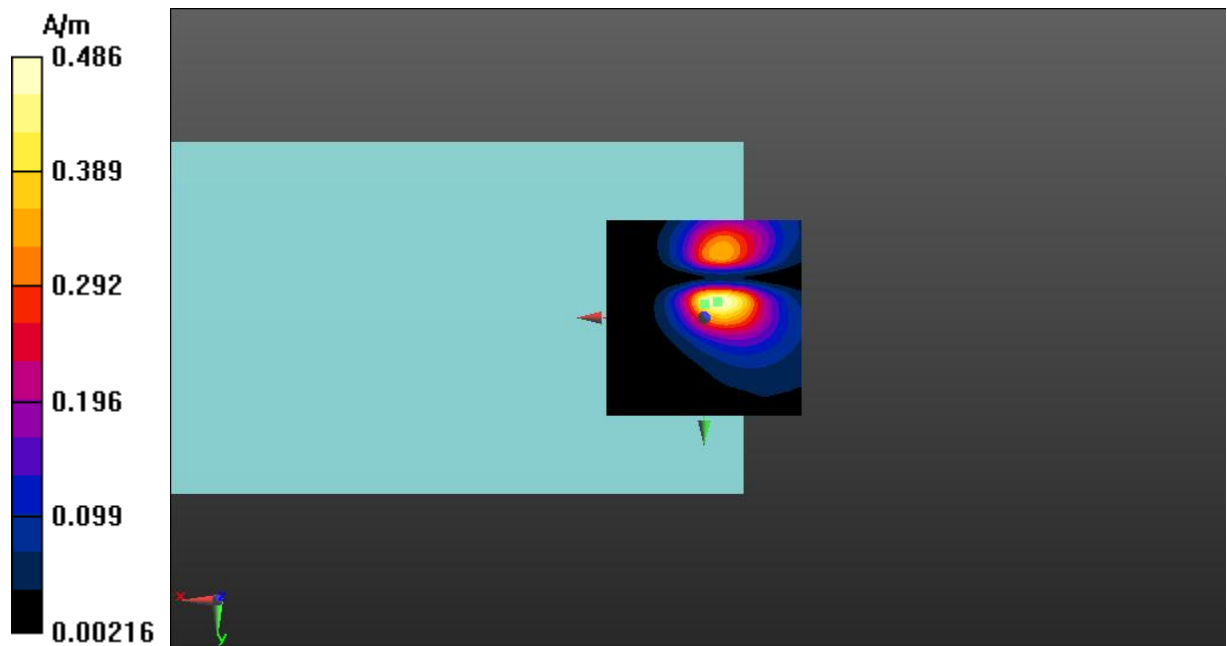
Fig A.17 T-Coil LTE-Band 41-Y
