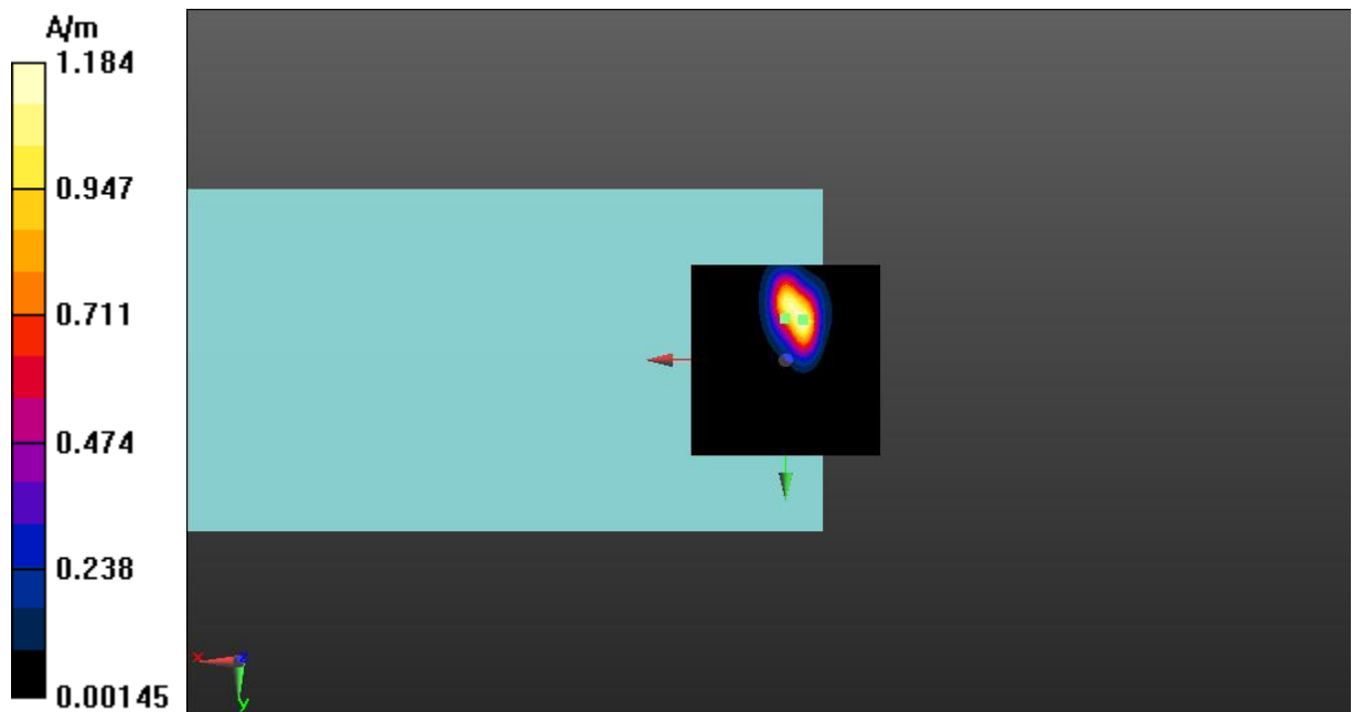
Fig A.13 T-Coil LTE-Band 25-Z
