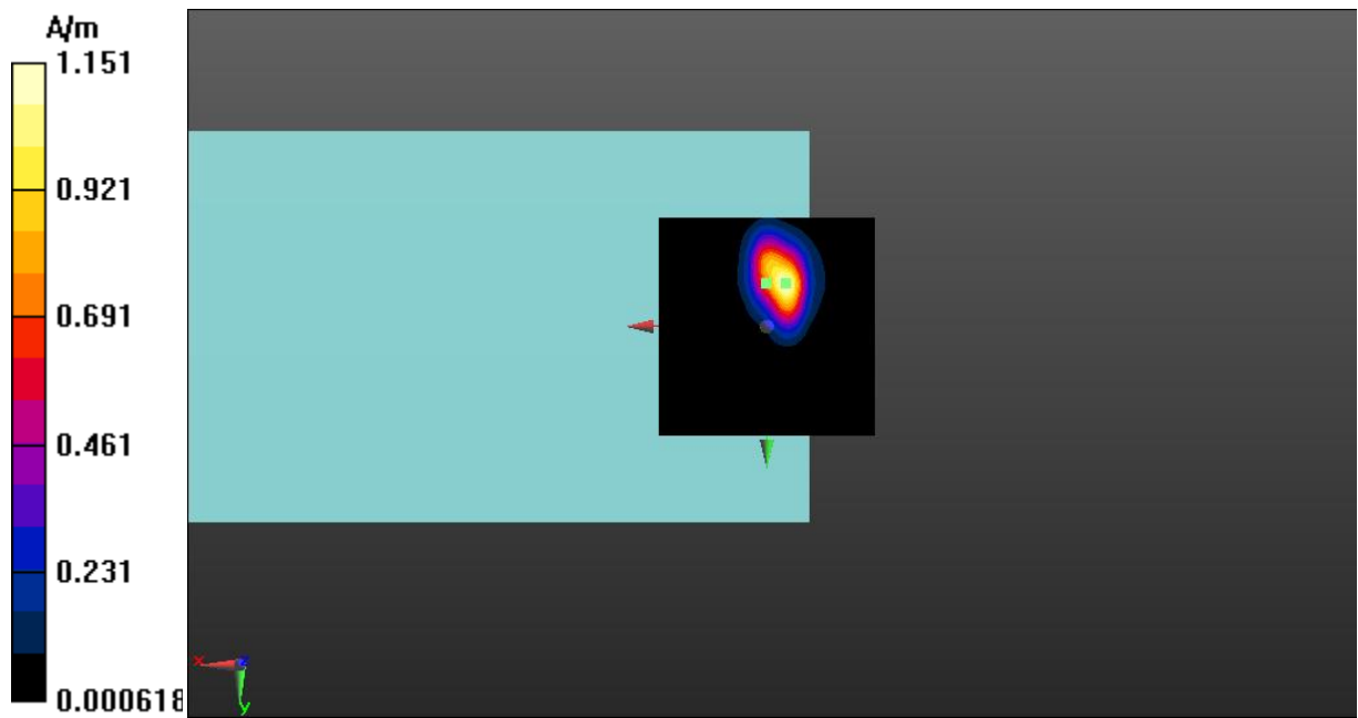
Fig A.16 T-Coil LTE-Band 38-Z
