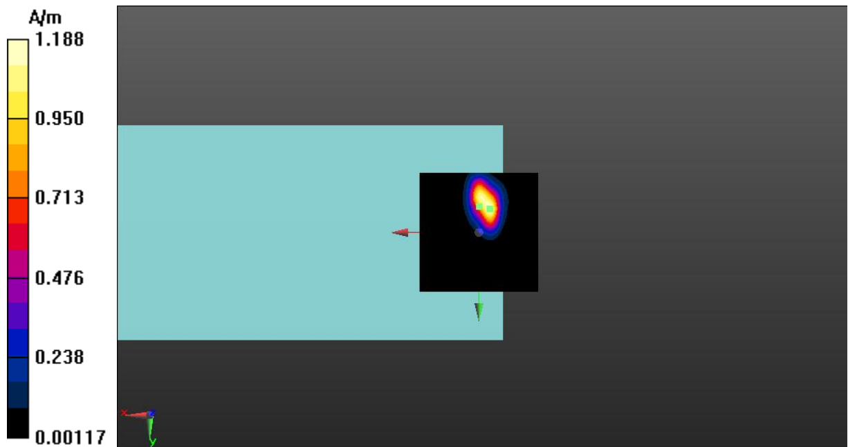
Fig A.15 T-Coil LTE-Band 66-Z
