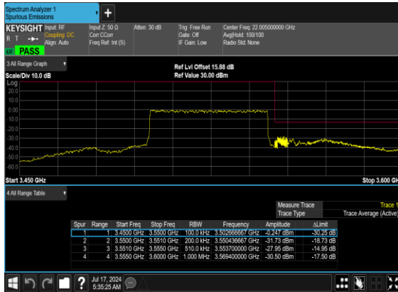
B2_N77(50M)_DFT-s- OFDM_BPSK_Outer_Full_High_CH
