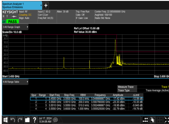
B2_N77(50M)_DFT-s- OFDM_BPSK_Edge_1RB_Right_High_CH
