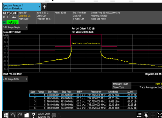
N14(5M)_DFT-s- OFDM_QPSK_Outer_Full_Low_CH
