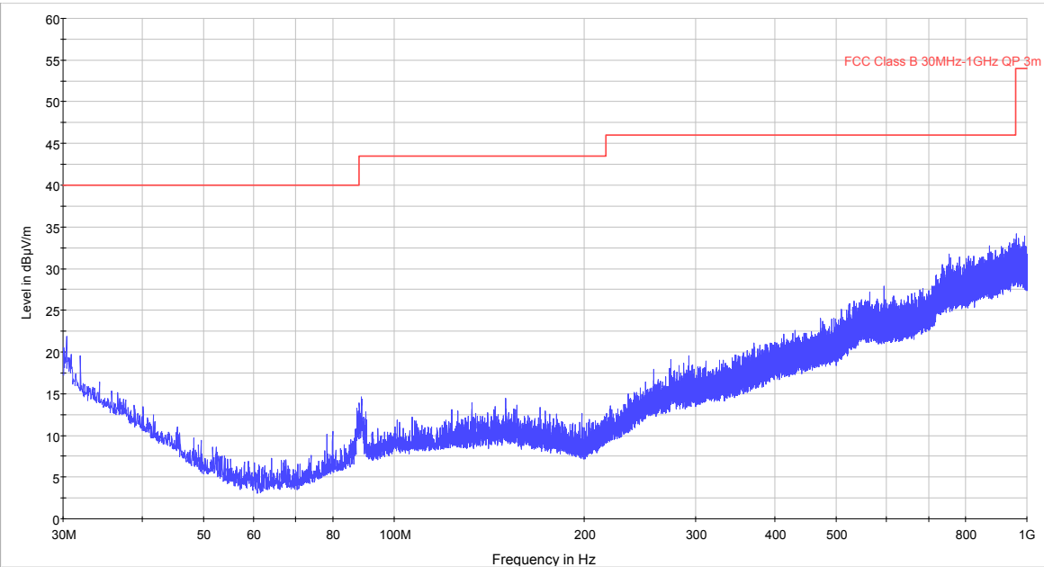
Unintentional Radiated Spurious emissions 30 MHz to 1 GHz
