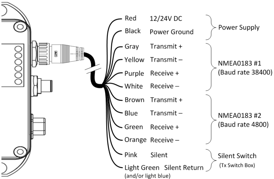
Figure 12 Wiring Instructions
