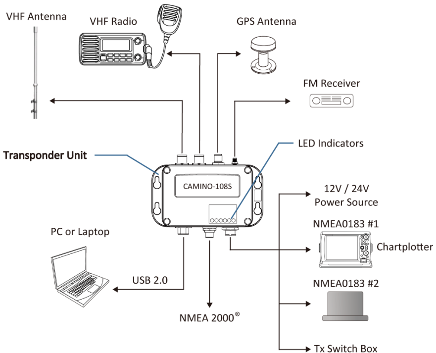
Figure 2 Connection Diagram
