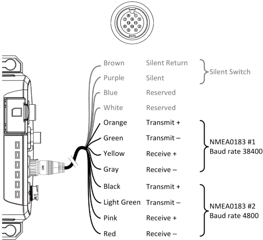
Figure 8 NMEA 0183 Connection
