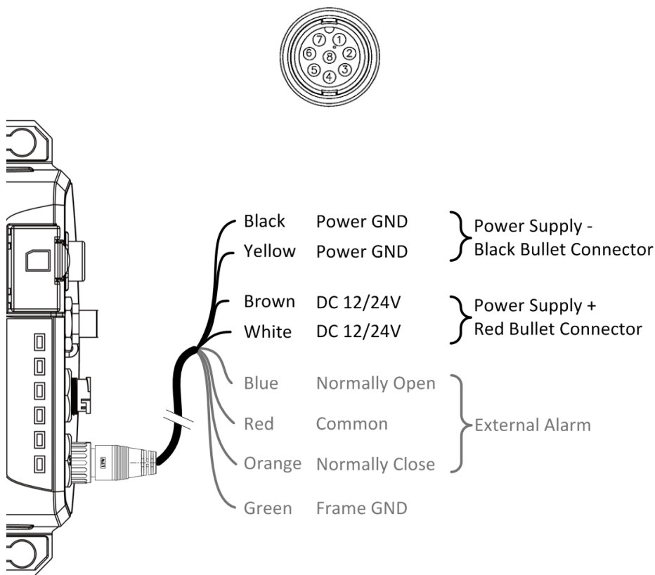
Figure 9 Power and Alarm Connection
