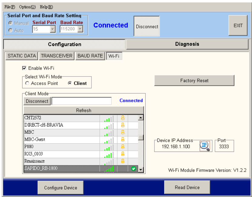
Figure 16 Client Mode
