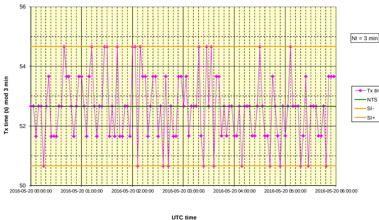
2016-05-20 - AMEC B600 - Test 10.5.2.1 Reporting interval 3 min
