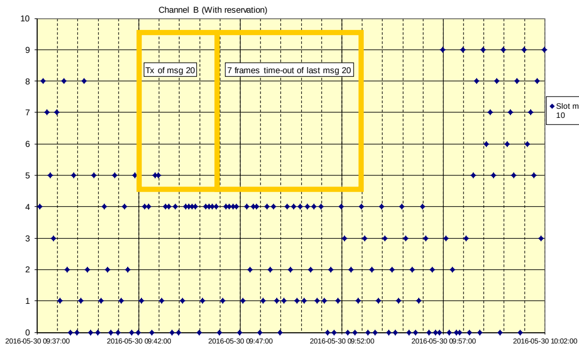
2016-05-30 - AMEC B600 - 12.6.7 Base station reservation, distance < 120 NM
