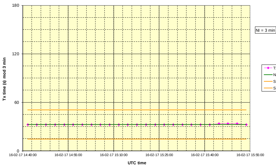
2017-02-16- Me - AMEC B600 - Test 13.6.1 Reporting interval of message 27
