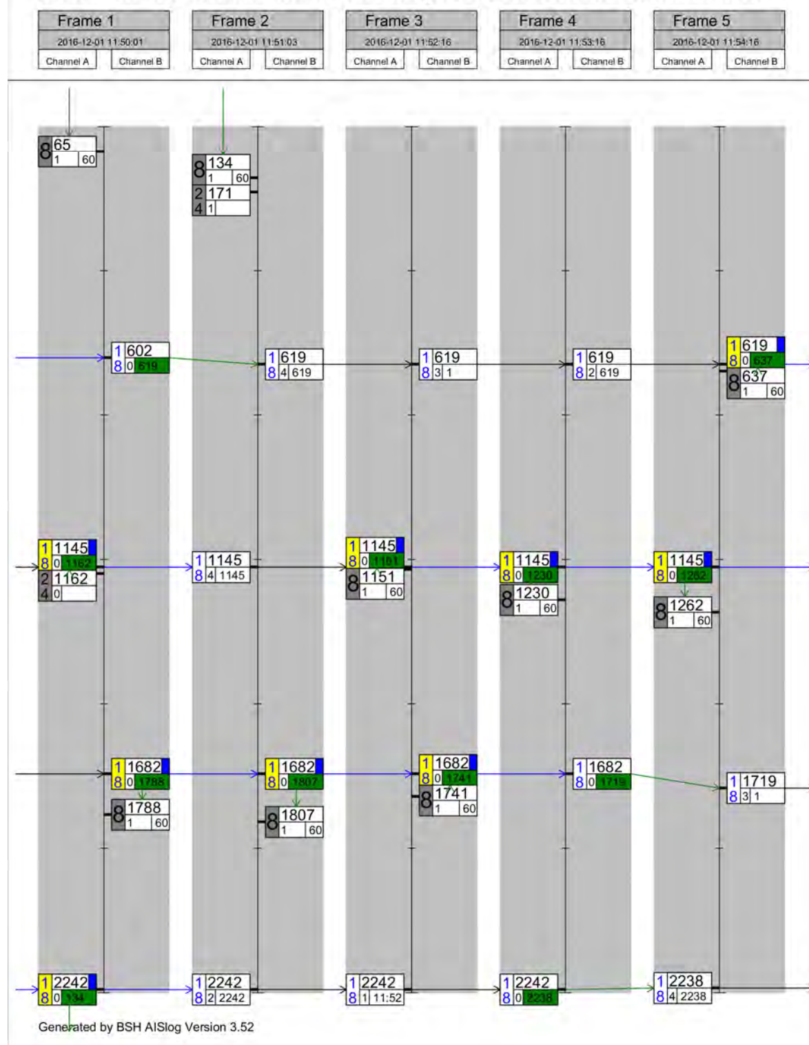
2016-12-01 - AMEC B600 - Test 10.2.2.6 Single ITDMA and RATDMA transmissions
