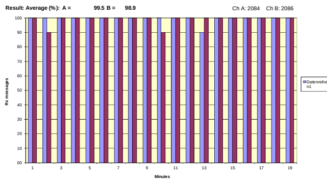
2016-07-01 - AMEC B600 - Test 10.2.1.5 Receive in slots after own Tx
