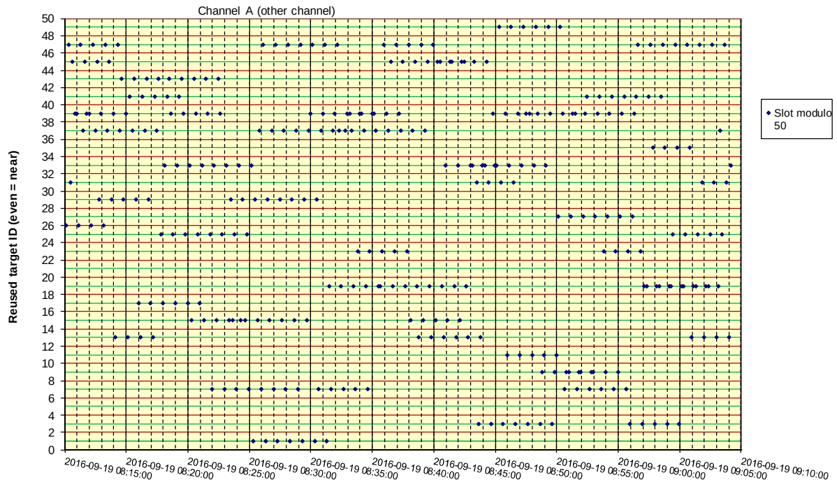
2016-09-19 - AMEC B600 - 13.5c Slot reuse
