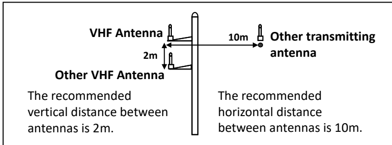
VHF Antenna Locations
