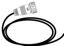
12pin cable with power, dual NMEA0183, silent mode, 1m, 26AWG
