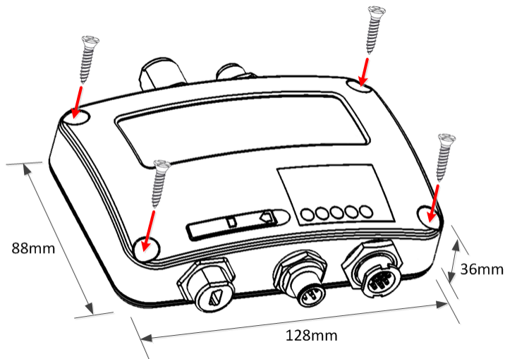
Figure 1 Mounting the transponder
