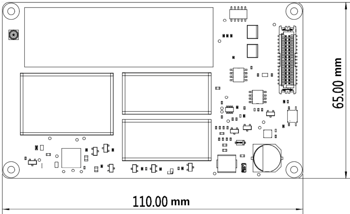
Figure 6-2-4 Top View
