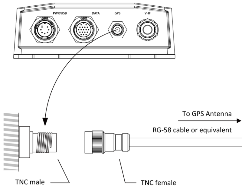
Figure 2-3-1-1 GPS Antenna Installation
