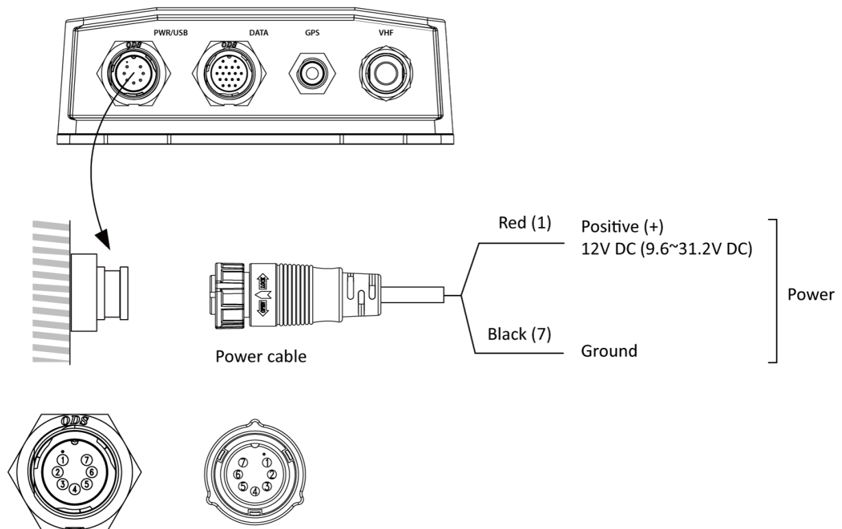
Figure 2-3-2-1 Power Connector
