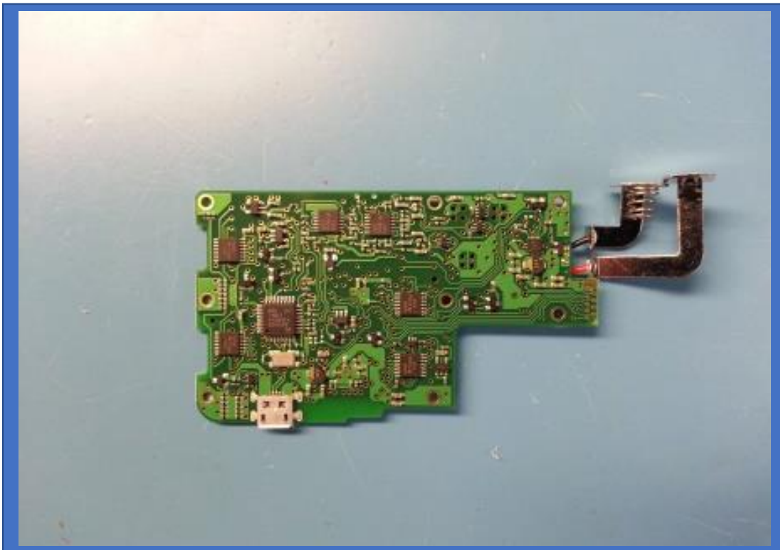
Figure 1.1-3: Rear view photo
