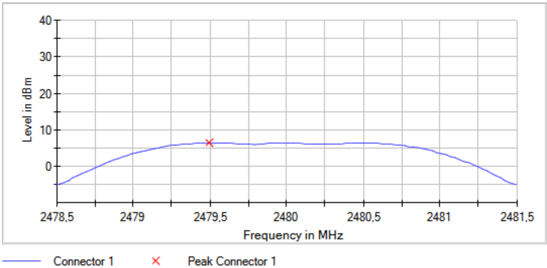
Peak Power
