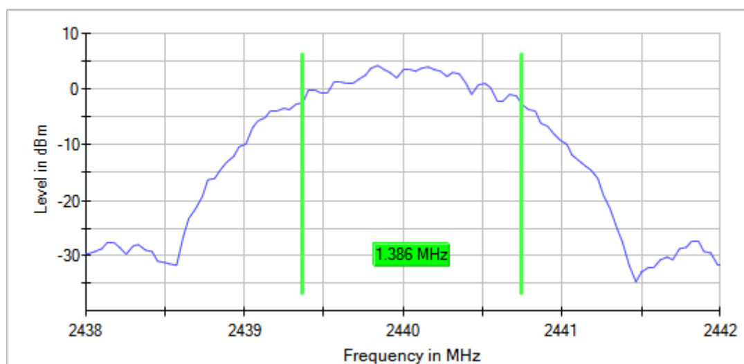
6 dB Bandwidth
