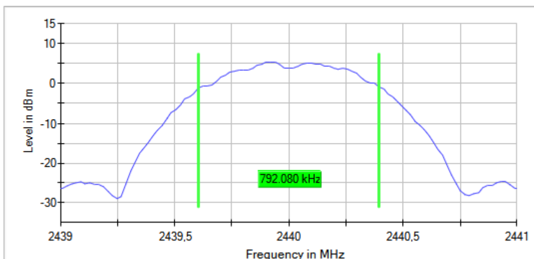
6 dB Bandwidth
