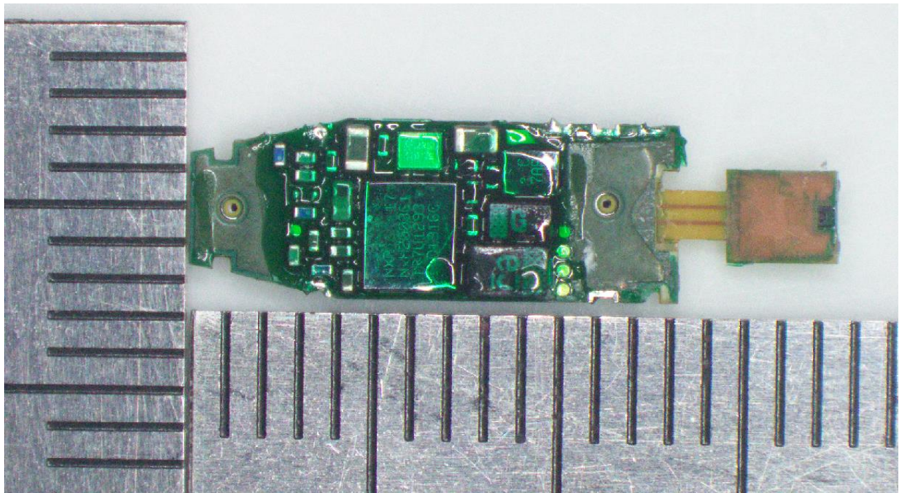
PCB BOTTOM SIDE VIEW
