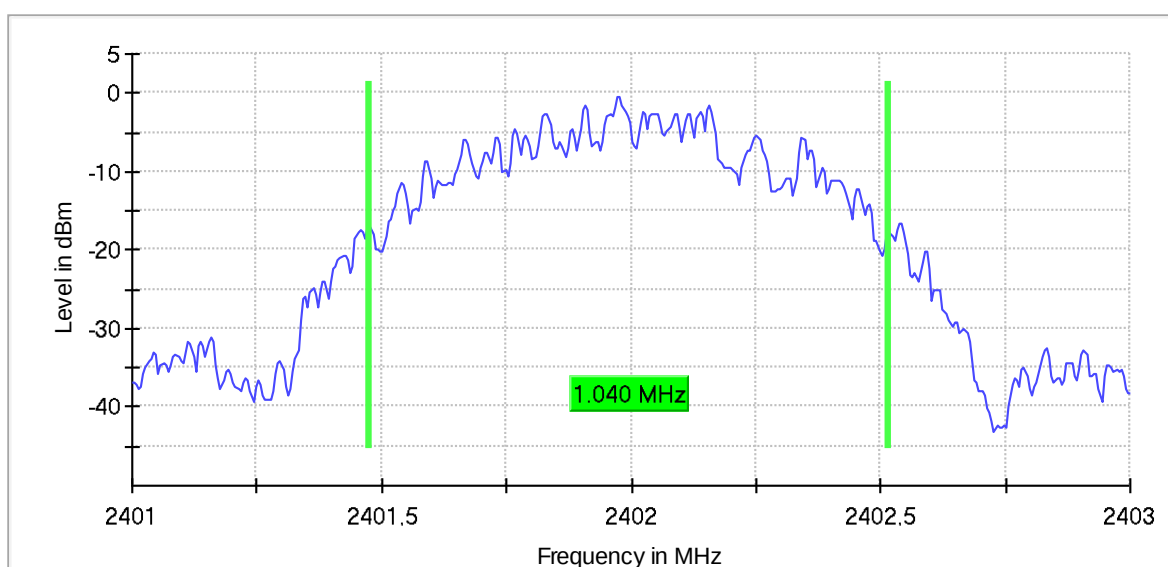
99 % Bandwidth
