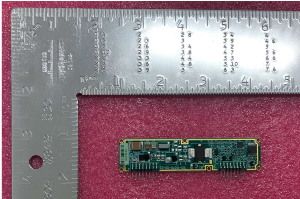
AIRLINK ACSES: Power Amplifier Module (PAM) without Shield– Top
