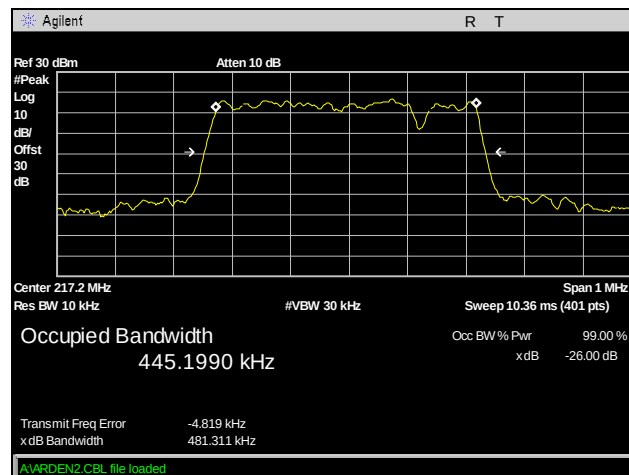
Plot 2. Occupied Bandwidth, Channel 217.25 MHz, 64QAM, BW 500 kHz
