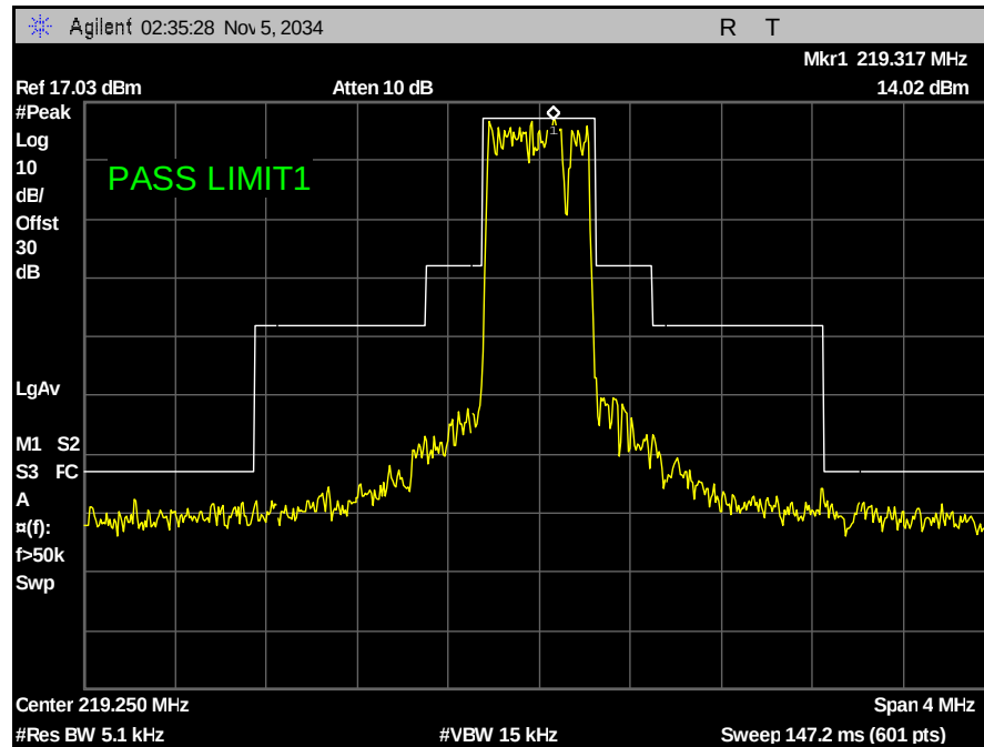
Plot 21. Emission Mask, Channel 219.25 MHz, 64QAM, BW 500 kHz
