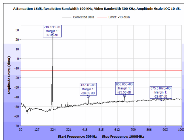
Plot 18. Transmitter Radiated Unwanted Emissions, 218.75 MHz, 30 MHz – 1 GHz
