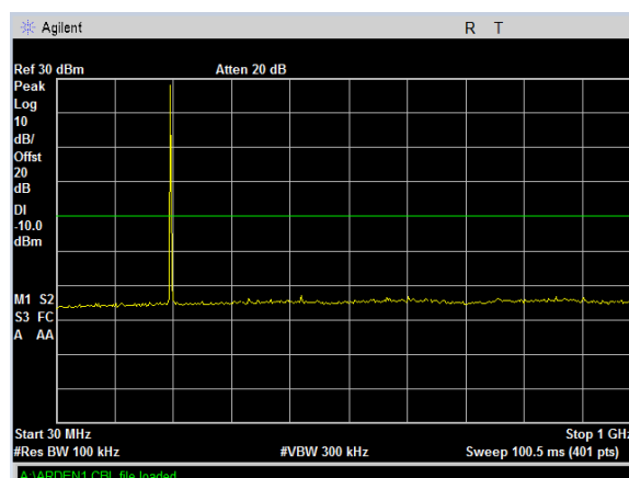
Plot 12. Transmitter Conducted Unwanted Emissions, Channel 218.75M, mode 64QAM, BW 500 kHz, 30 MHz to 1 GHz
