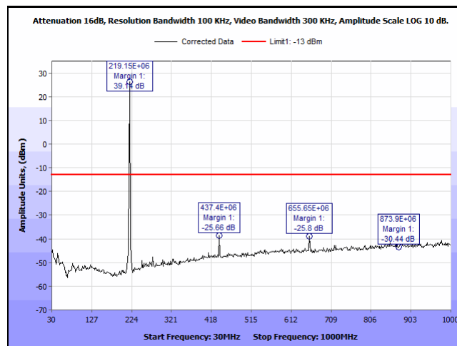
Plot 17. Transmitter Radiated Unwanted Emissions, 218.5 MHz, 30 MHz – 1 GHz
