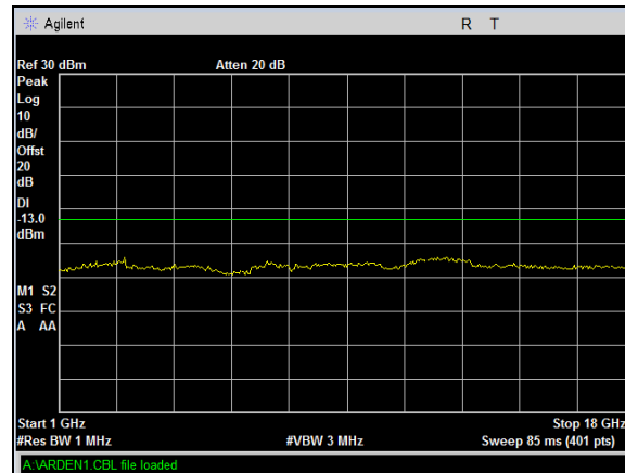
Plot 7. Transmitter Conducted Unwanted Emissions, Channel 218.25M, mode 64QAM, BW 500 kHz, 1 GHz to 18 GHz
