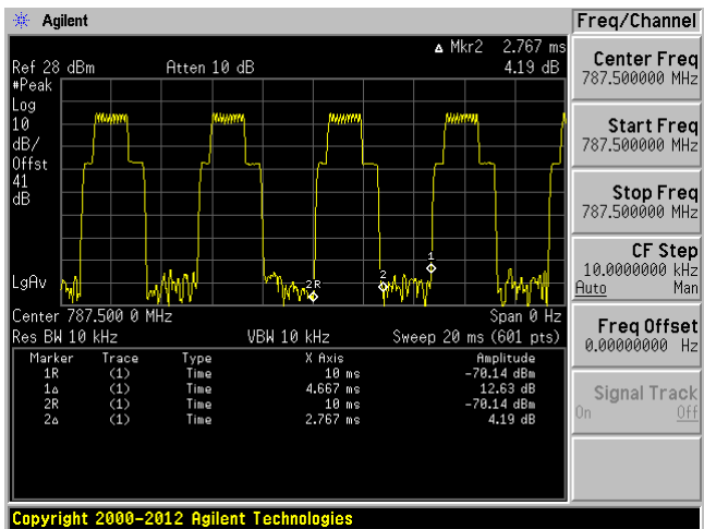
787.5 MHz BPSK
