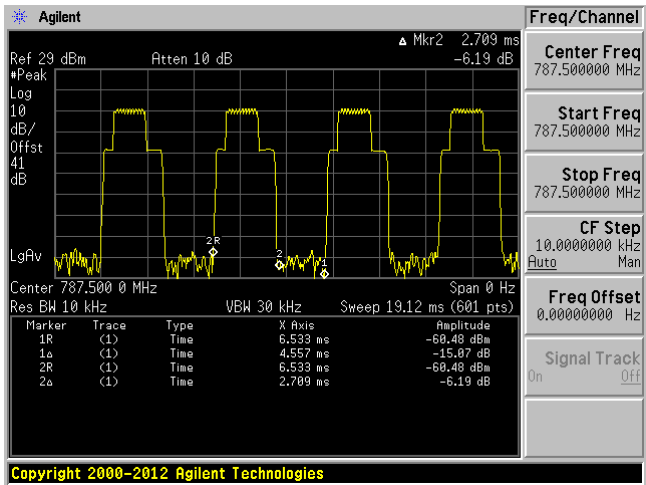
787.5 MHz 64QAM
