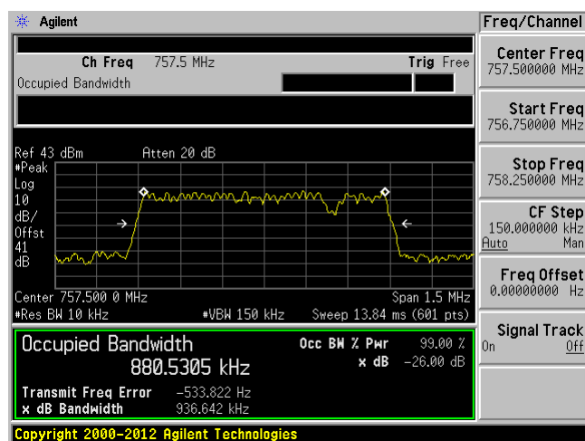
757.5 MHz 64QAM
