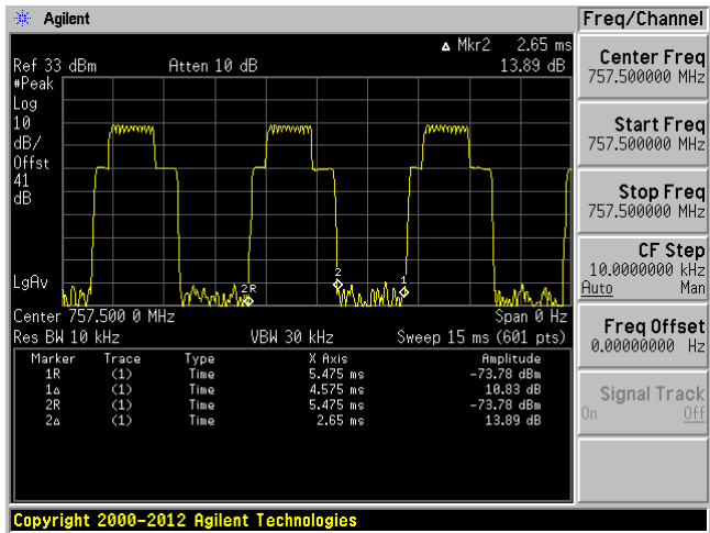
757.5 MHz 64QAM
