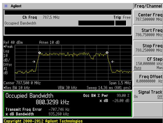
787.5 MHz 64QAM
