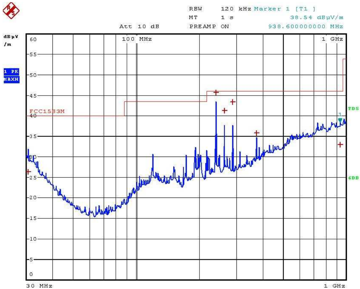
Graph 61 Radiated Emissions Test Results – Mode 4: Transmit Mode (Data Stream) – Ch11 – Horizontal.
