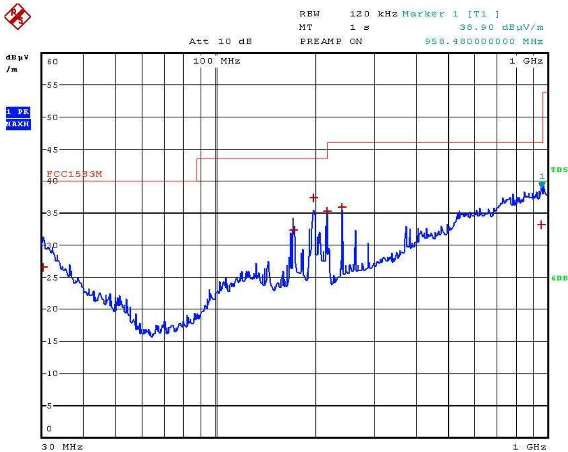
Graph 22 Radiated Emissions Test Results – Mode 2 – Receive Ch18 – Vertical – 30 to 1GHz.
