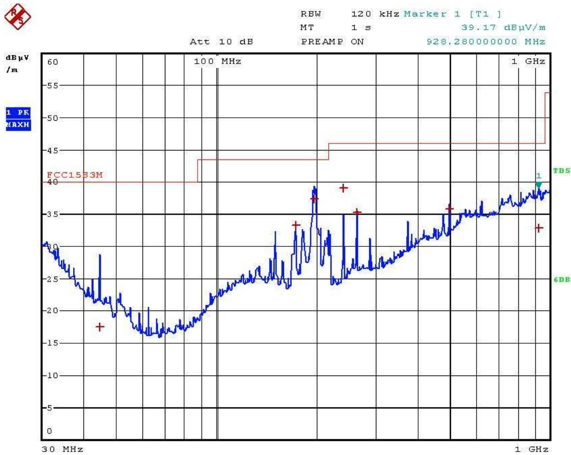
Graph 2 Radiated Emissions Test Results – Mode 1 – Receive Ch11 – Vertical.
