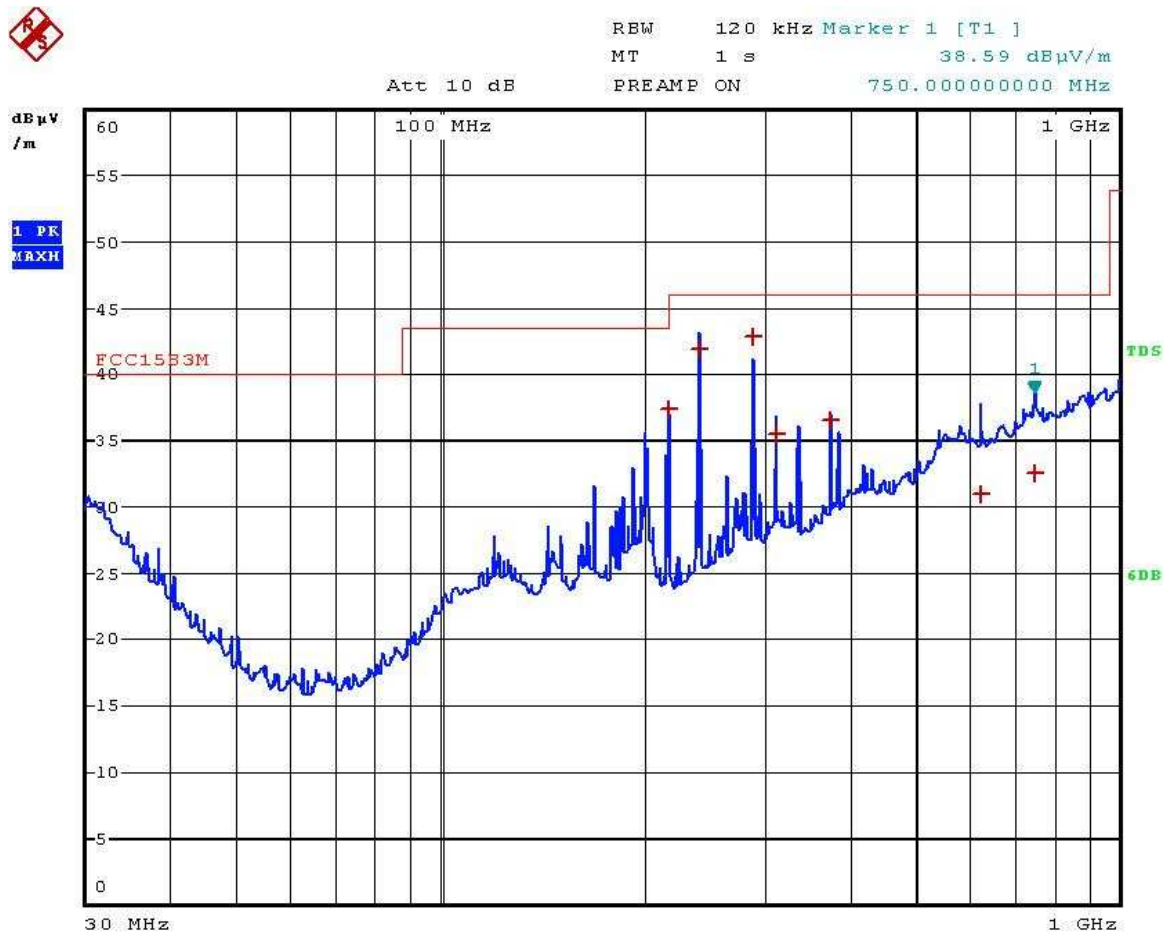
Graph 101 Radiated Emissions Test Results – Mode 6: Transmit Mode (Data Stream) – Ch26 – Horizontal.
