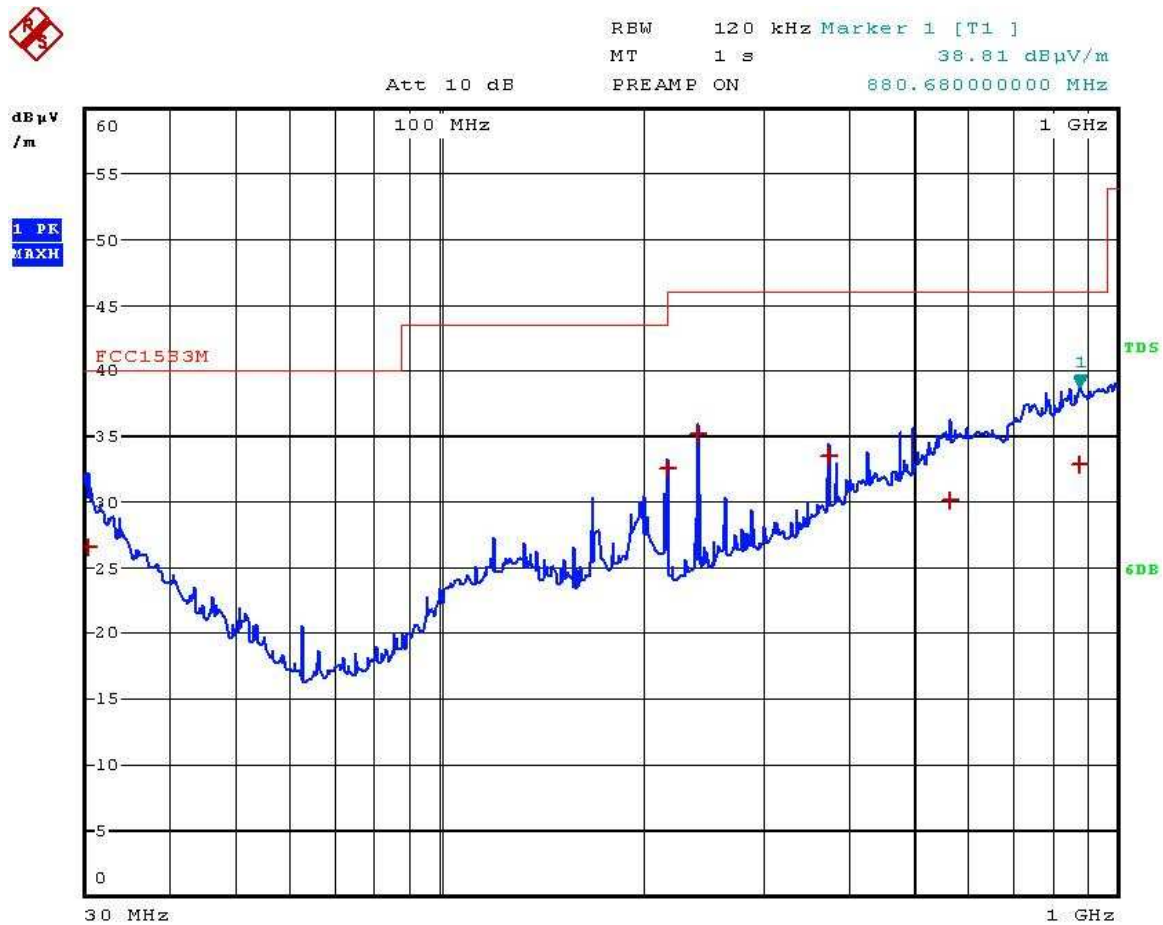
Graph 42 Radiated Emissions Test Results – Mode 3 – Receive Ch26 – Vertical.
