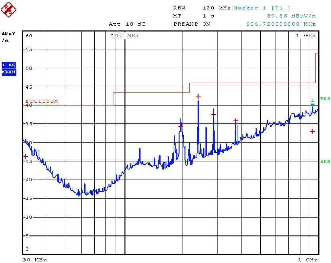
Graph 21 Radiated Emissions Test Results – Mode 2 – Receive Ch18 – Horizontal – 30 to 1GHz.
