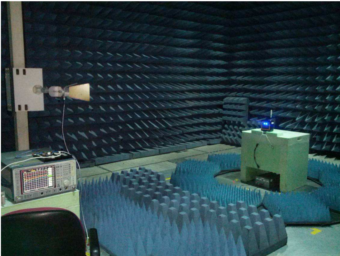
Radiated Emissions >1GHz
