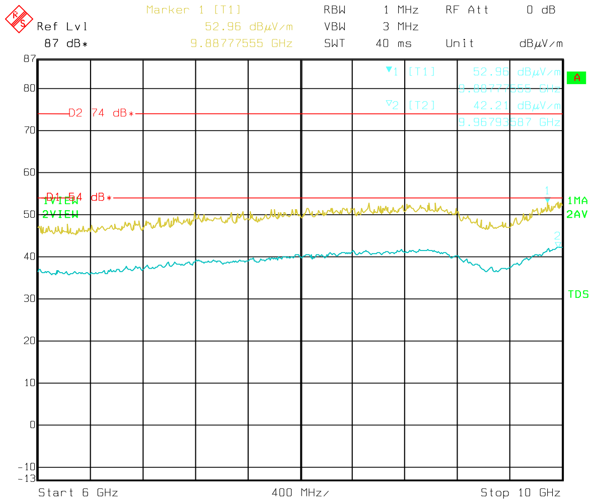
Graph 6 Radiated Emissions Test Results – Mode 1 – Receive Ch11 – Horizontal – 6 to 10GHz.
