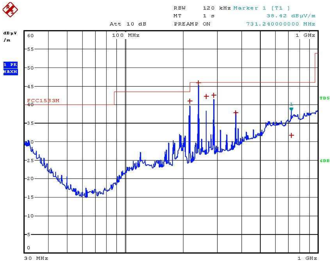
Graph 81 Radiated Emissions Test Results – Mode 5: Transmit Mode (Data Stream) – Ch18 – Horizontal.
