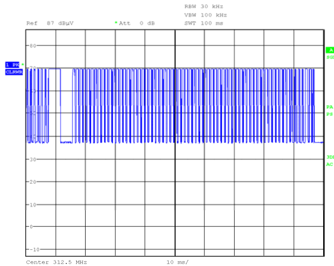
Figure 7.5.2-1: Duty Cycle
