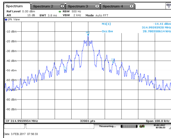
Figure 7.4.2-2: 99% Bandwidth
