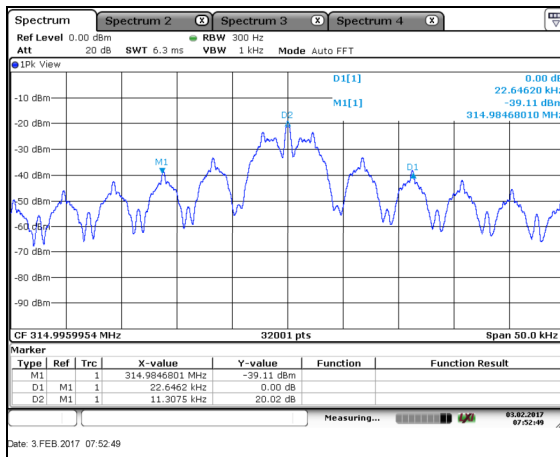
Figure 7.4.2-1: 20 dB Bandwidth
